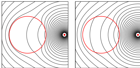
Fig. 5.1 Analogue of Figure 3.1 for the continuum approximation determined by (5.1) and (5.5)–(5.9). Again the number of disks is fixed at n = 12 and the radius r varies. Note the striking agreement of the two images shown with those of Figure 3.1, corresponding to values \alpha = 5.660 and 2.713 . The first image is absent because in this case rn > 1 , making \alpha negative and the homogenized approximation inapplicable. The mean potential \phi_0 of (5.7) is \log 2 \approx 0.693 .
