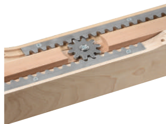
Standard Equalizing Gear Slides
