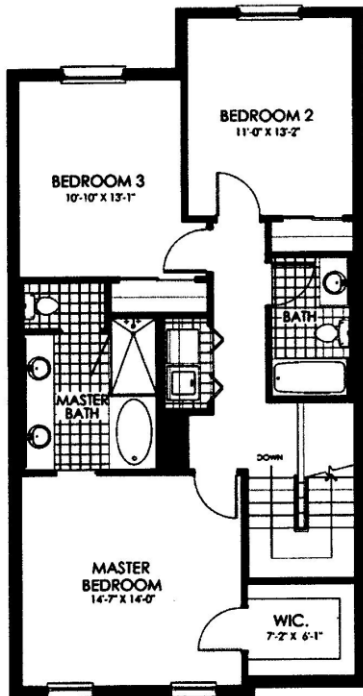
THIRD FLOOR
