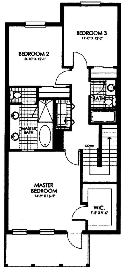
THIRD FLOOR
