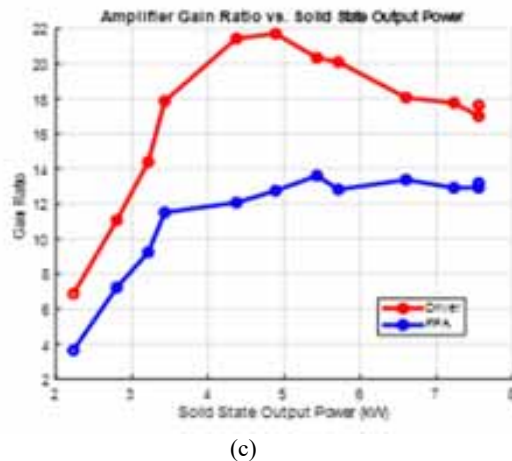
Figure 4: b), and (c) represent performance characterization of the FPA when driven by the driver tetrode, whereas (a), represents performance characterization of the FPA when driven by the Cryoelectra SSA.
