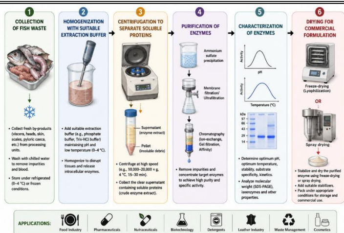
Figure 2. Extraction procedure of enzymes from fish waste Industrial applications
