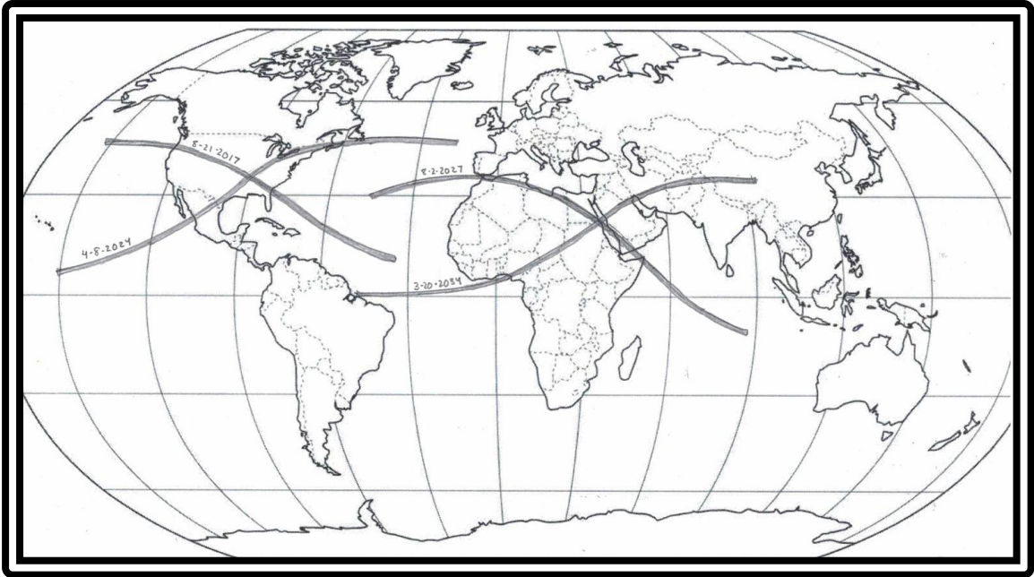
Above, The Egypt/Little Egypt Hepton Crosses of the Spring Equinox Metonic (2017 to 2034)
