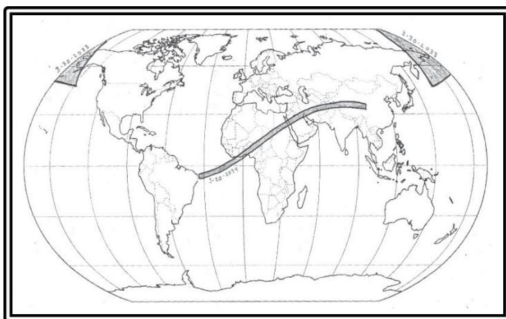
The total solar eclipses of 3-30- 2033 and 3-20-2034, one lunar year apart
