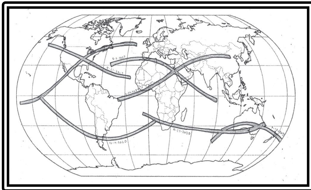
Above: The Hepton Cycle of 2017 to 2037
