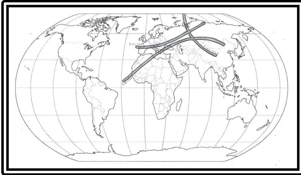
USSR eclipse Swarm
