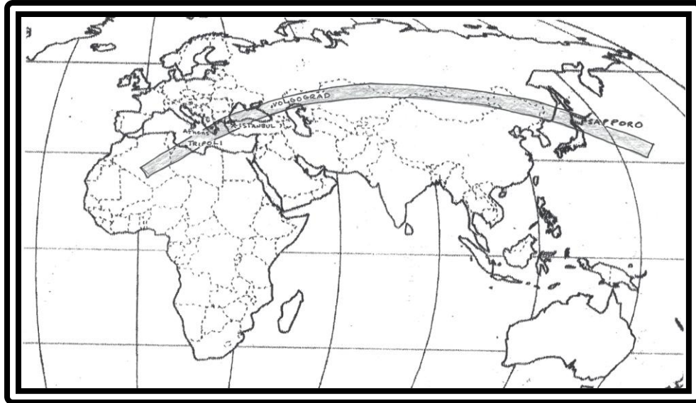
June 1 2030 Athens/Constantinople Ring of Fire.
