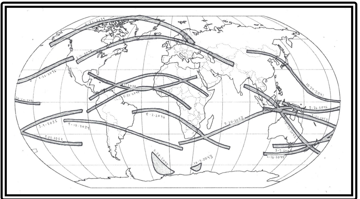
Above: 2034 to 2053 Ring of Fire Eclipses
