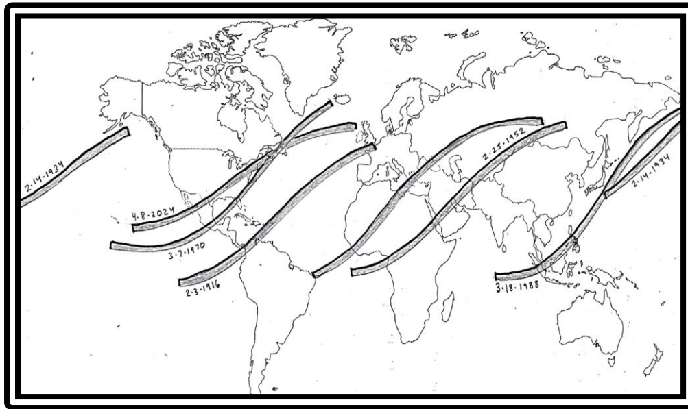
Saros 139 Total Eclipses Snapshot 1916 to 2024
