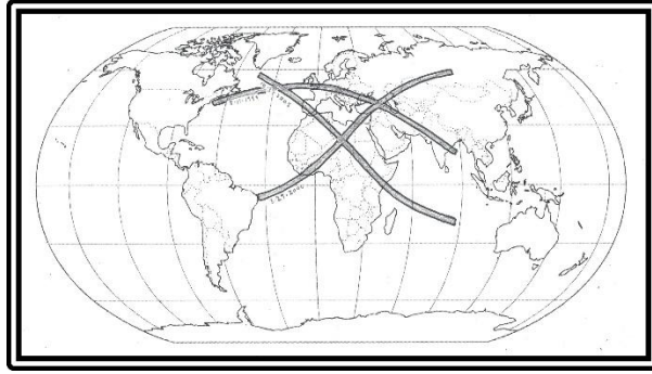
Mediterranean Aleph: Aug 11 1999, Oct 3 2005, March 29 2006
