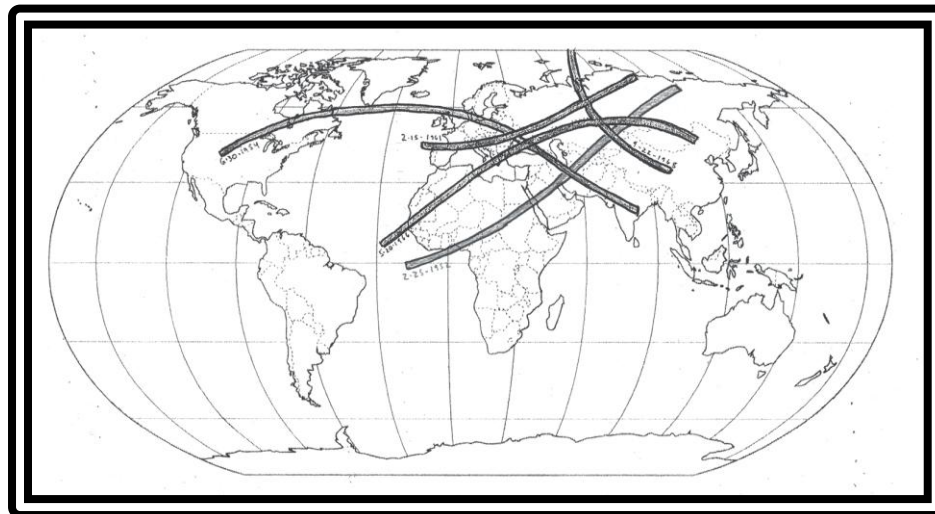
Full USSR Swarm 1952 to 1968 (above)
