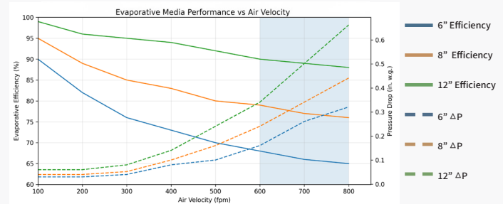
EVAPORATION EFFICIENCY AND PRESSURE DROP STAYCOOL PRO 7060 "7MM FLUTE 45/15 ANGLES
