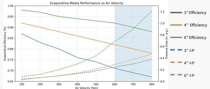
EVAPORATION EFFICIENCY AND PRESSURE DROP STAYCOOL HD 5090 "5MM FLUTE 45/45 ANGLES
