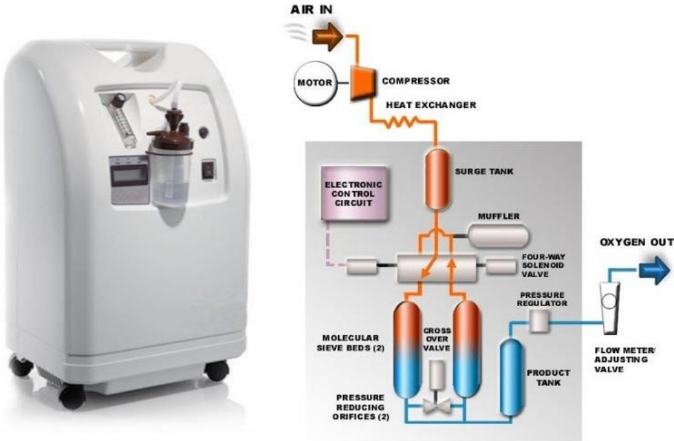
OXYGEN CONCENTRATOR
