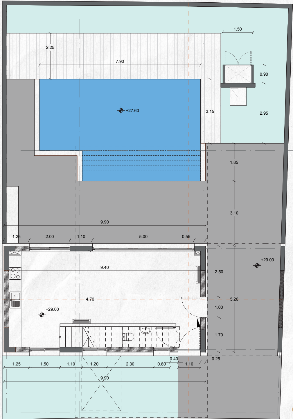
GROUND FLOOR
