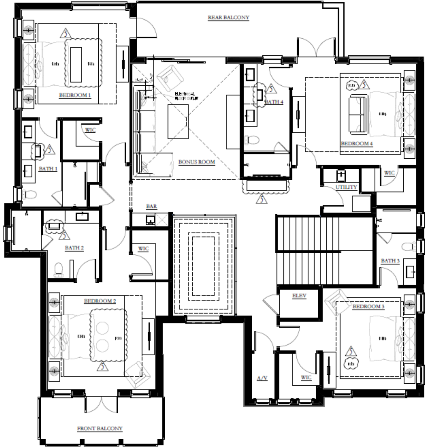
1 FURNITURE PLAN - SECOND FLOOR
