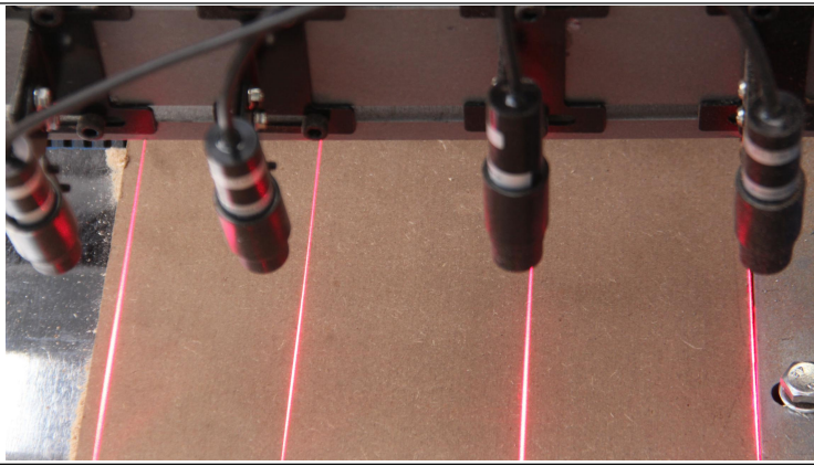
Optional Laser line for a precise guiding of cutting
