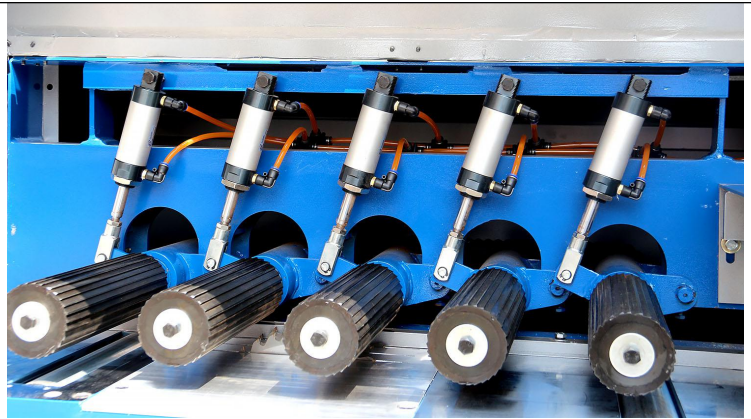
Multi 5 pcs of sharpen teeth or rubber roller for stable and smooth feeding
