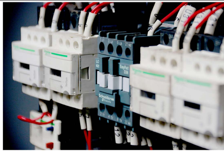
European electrical wiring
