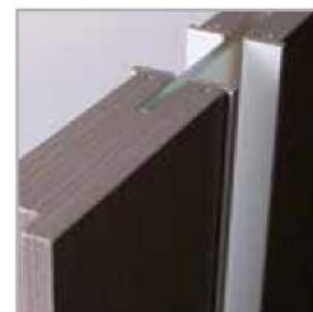
top door leaf edge without a rebate
