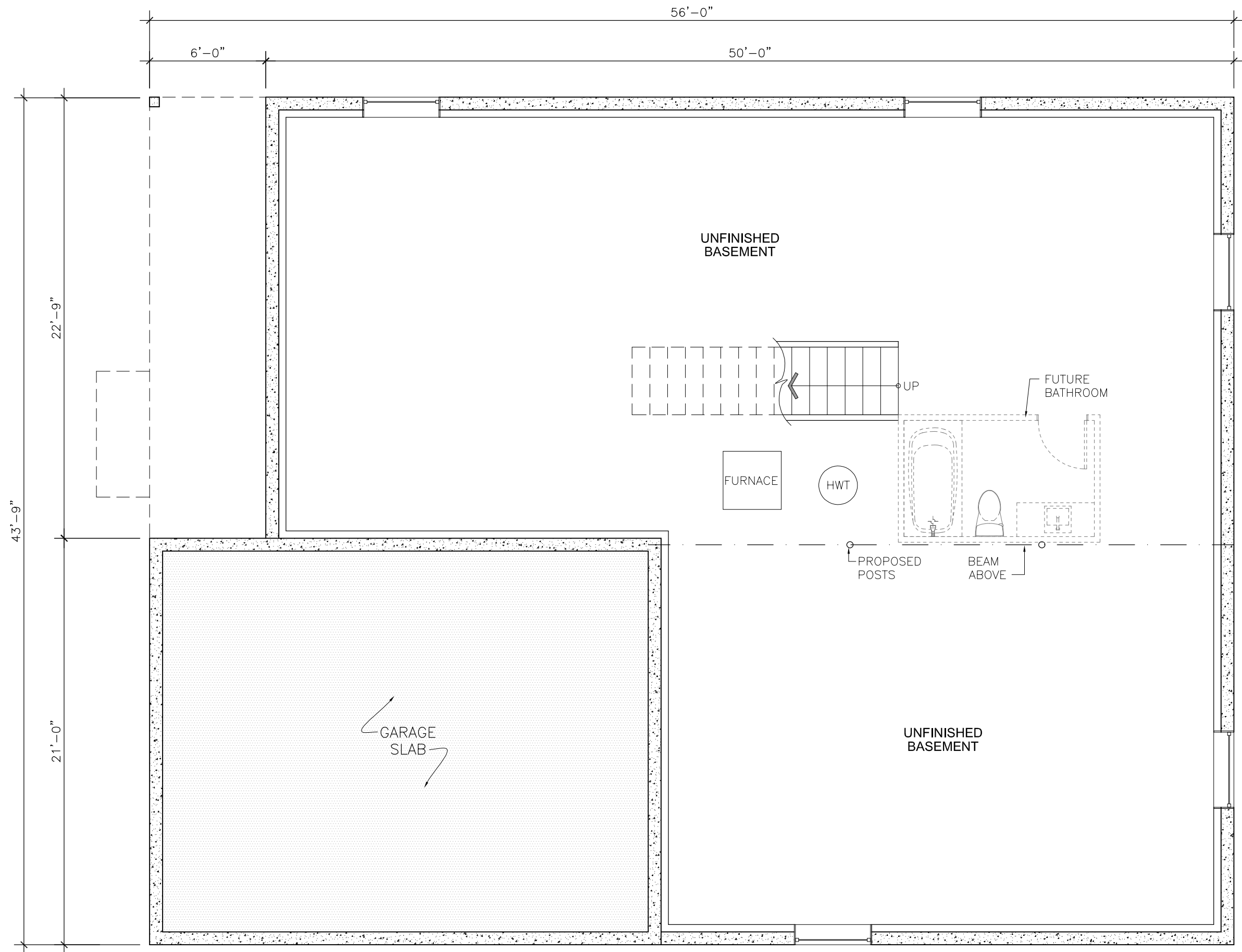
PROPOSED BASEMENT PLAN
