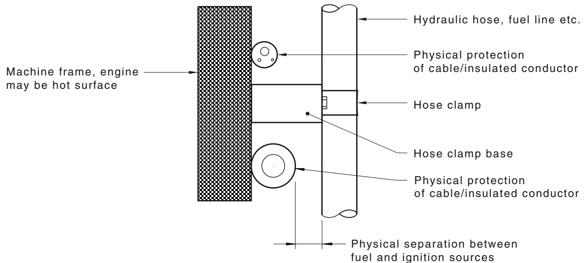
FIGURE C2 EXAMPLE OF GOOD PRACTICE—GOOD SEPARATION BETWEEN FUEL AND IGNITION SOURCES; PHYSICAL PROTECTION OF ELECTRICAL CABLES; HOSES SECURE
