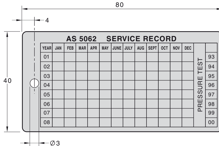
FIGURE 11.1 SERVICE TAG
