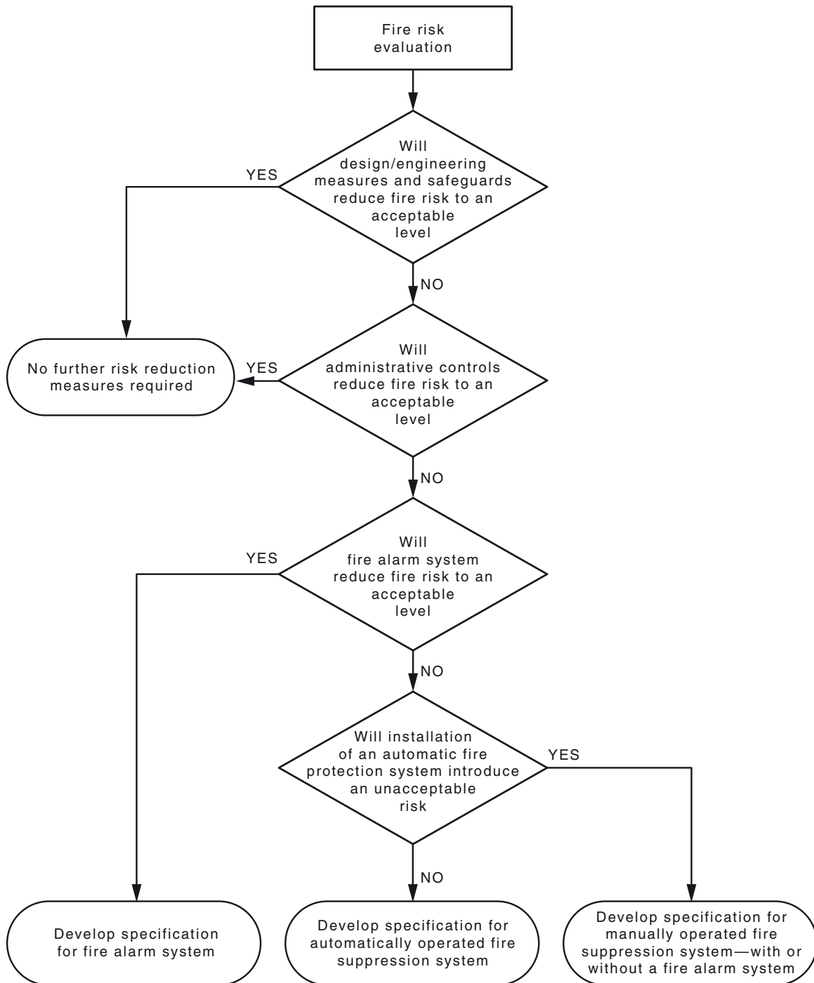
FIGURE 3.3 SELECTION OF FIRE SUPPRESSION SYSTEMS
