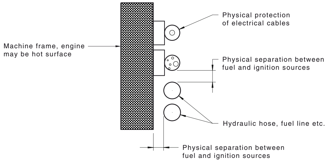
FIGURE C1 EXAMPLE OF GOOD PRACTICE—GOOD SEPARATION BETWEEN FUEL AND IGNITION SOURCES; PHYSICAL PROTECTION OF CABLES
