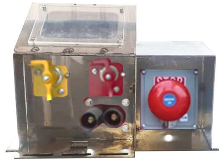
LOTOBOX 4SYSTEM, SWITCH PUSH PULL
