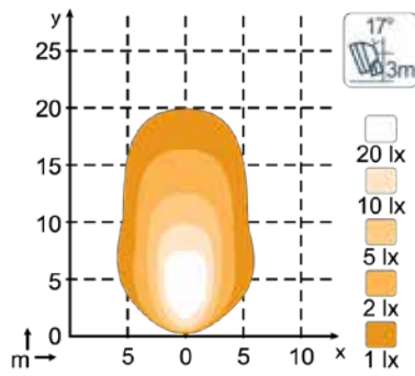
Canis GO 420, 1800lm Flood
