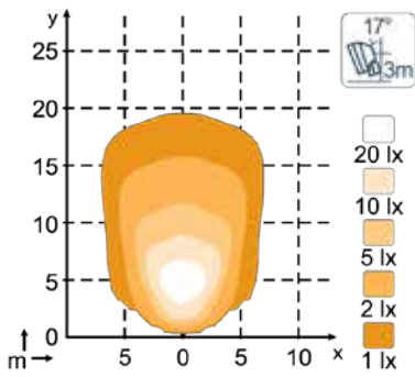
Canis GO 420, 1800lm Wide Flood
