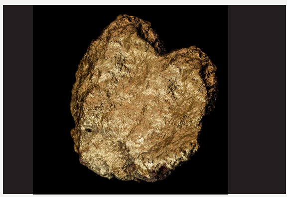
Gold
