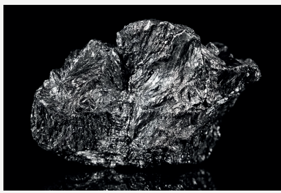
Graphite
