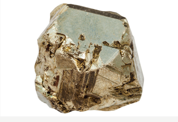
Pyrite
