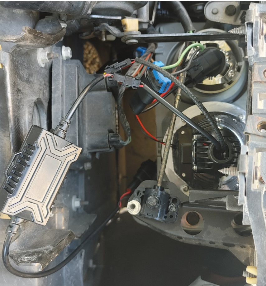
LED driver connected. (not yet mounted)
