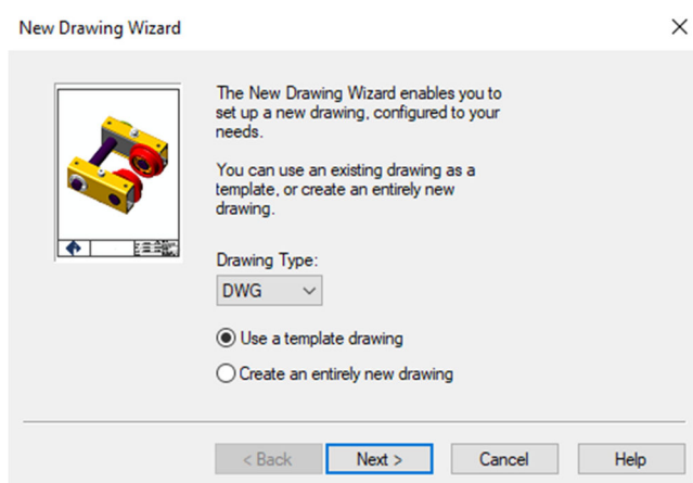
Figure 1 Template Setting
