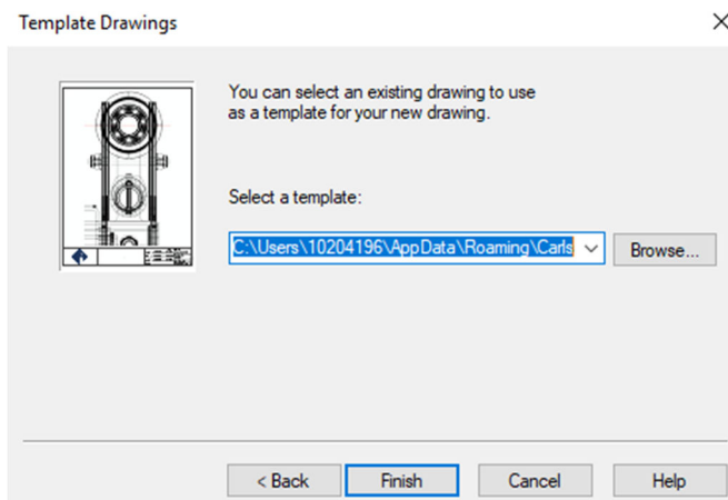
Figure 2 Template Selection
