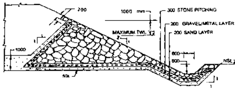
FIGURE 40. Details of rock toe protection with toe drain where TWL is higher than SGL
