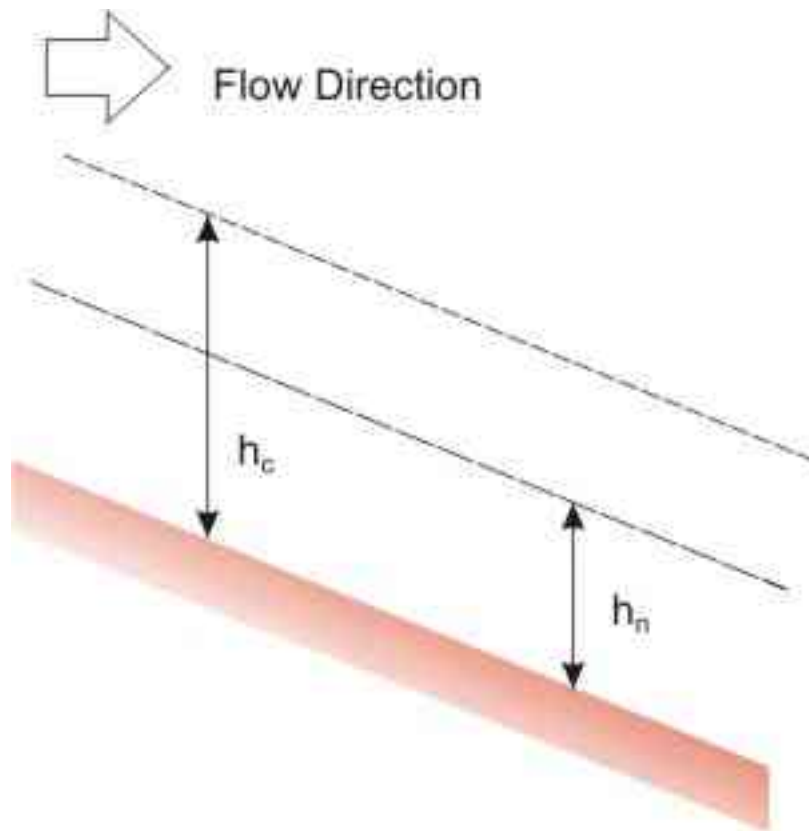
FIGURE 24. Slope increased substantially h_n < h_c ; Steep slope
