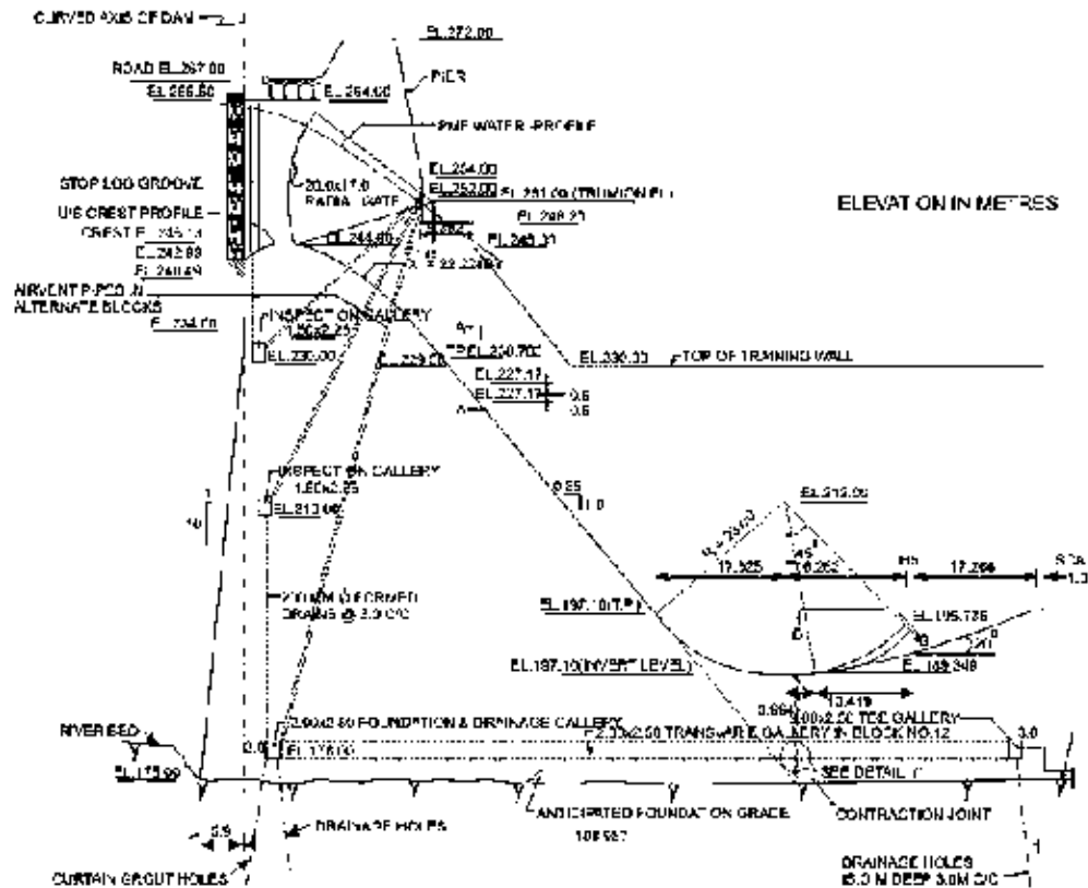
FIGURE 83. Indira Sagar Dam Spillway
