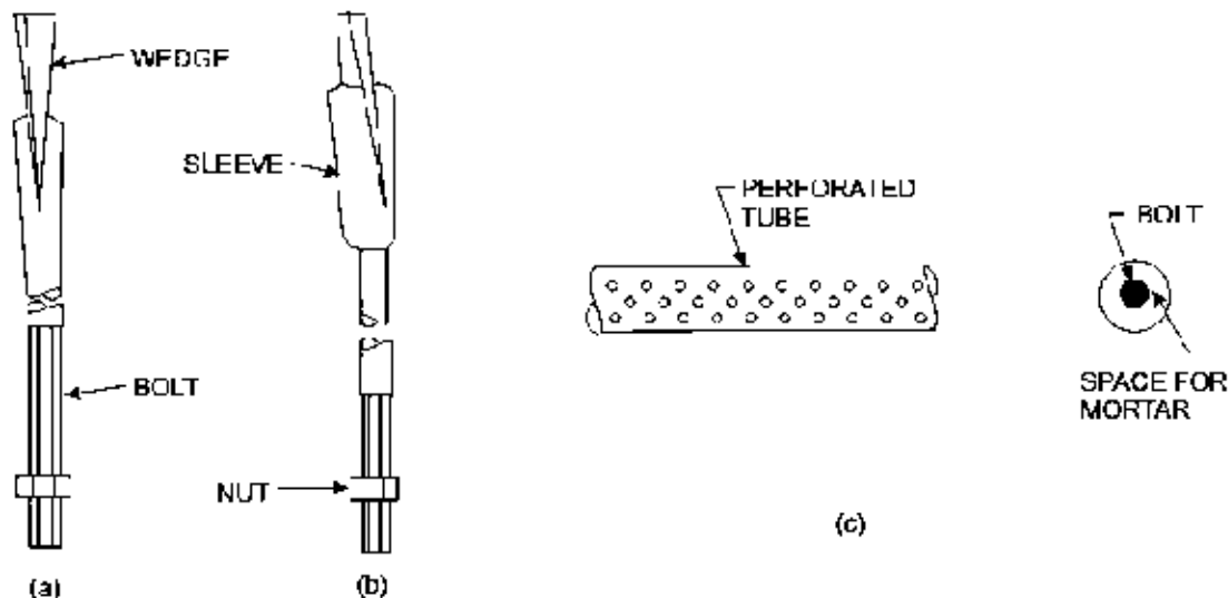
FIGURE 25 Different types of rock/roof bolts (a) Wedge & slot bolt (b) Wedge & sleeve bolt (c) Perforated tube
