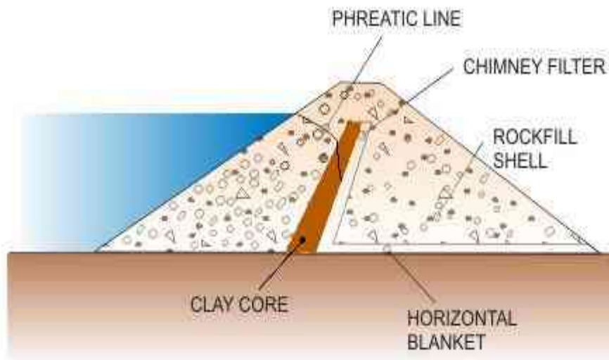
FIGURE 9 . Rock fill dam with inclined clay core, chimney drain and horizontal blanket
