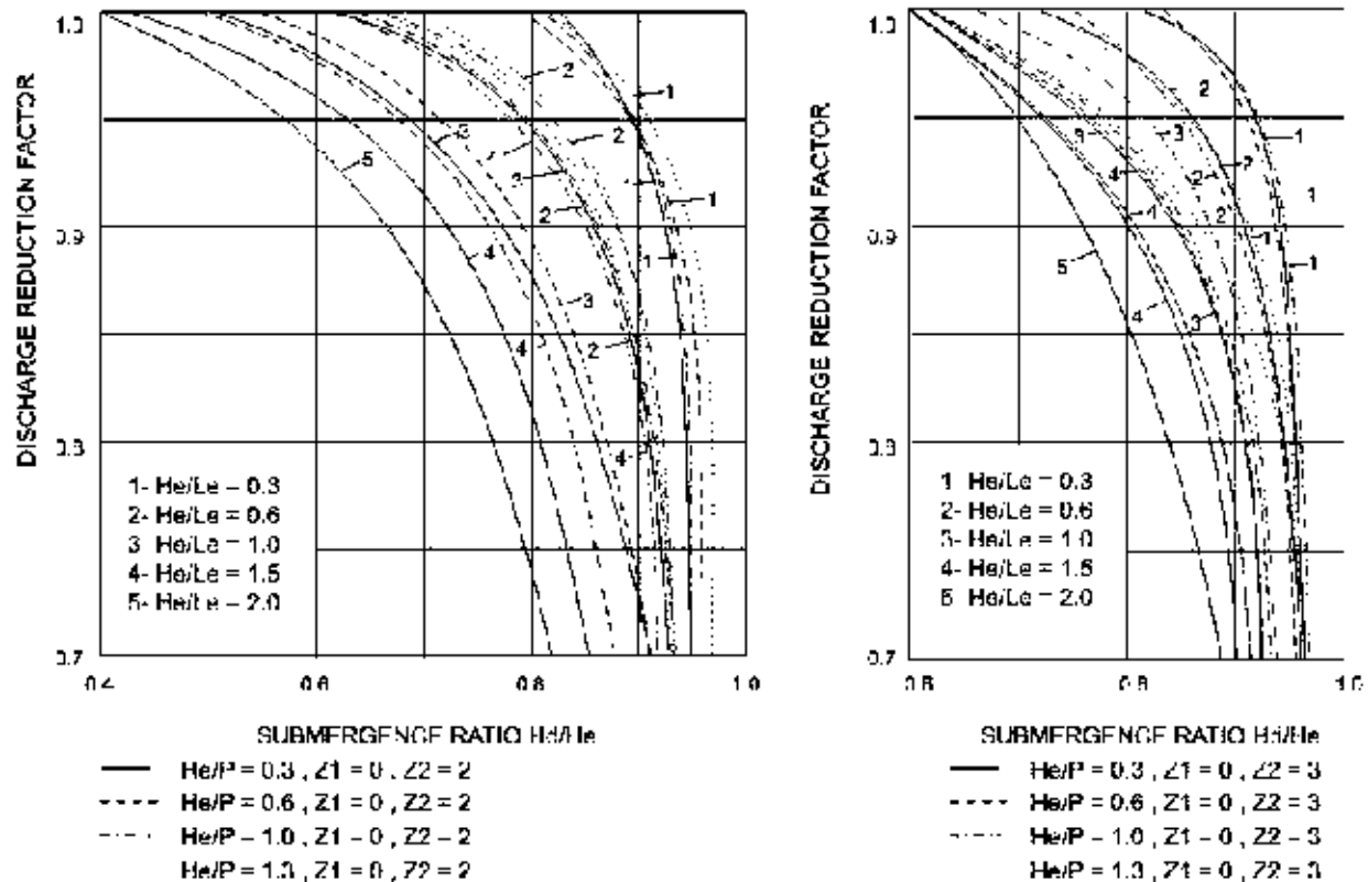
FIGURE 8. Variation of discharge reduction factor for submerged flow Adapted from IS 8534: 1994 Canal Head Regulators - Criteria for Design
