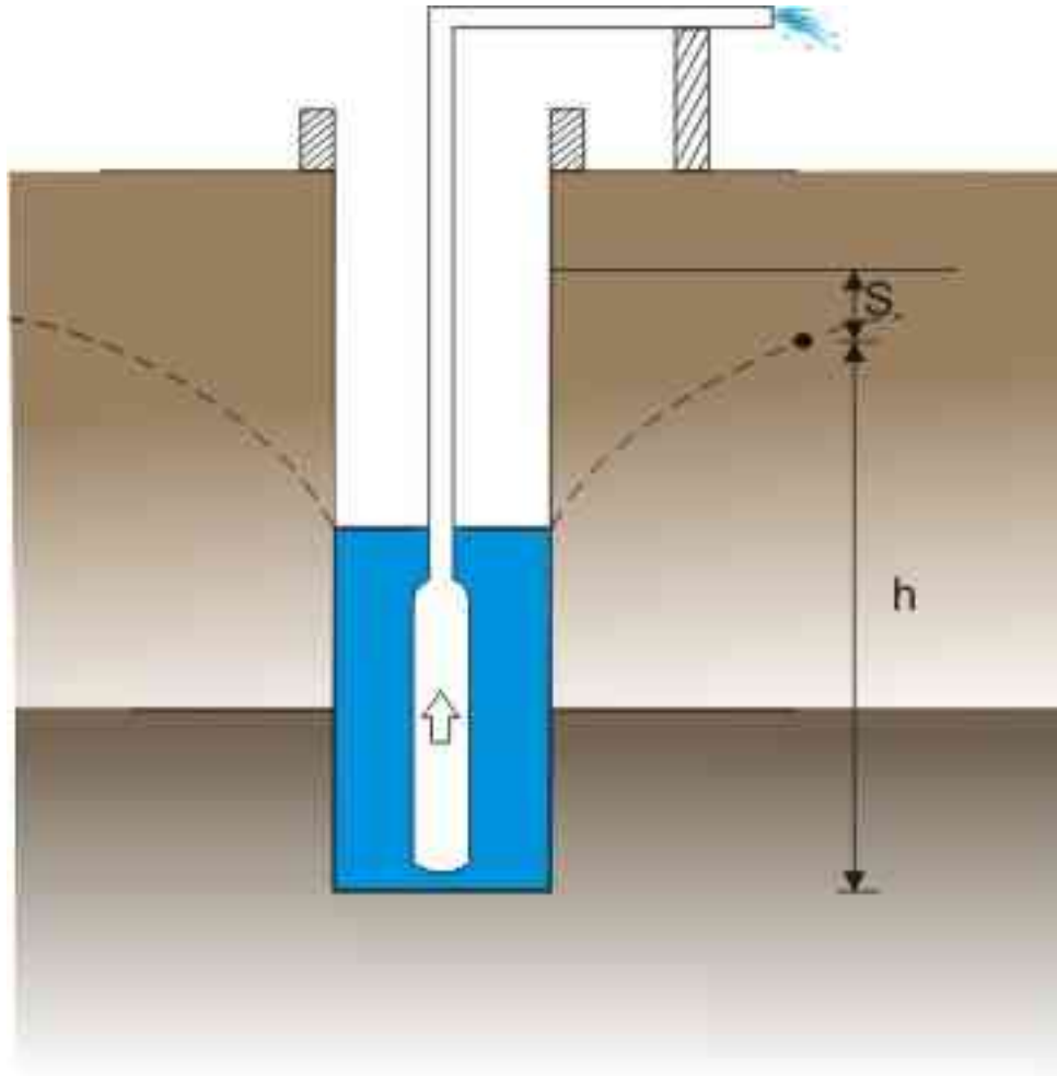
FIGURE .8 DEFINITION OF DRAWDOWN : S
