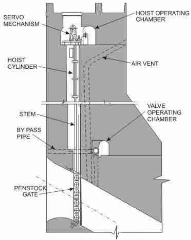
FIGURE 13. TYPICAL ARRANGEMENT OF VERTICAL LIFTGATE WITH WHEELS WITH HYDRAULIC HOIST
