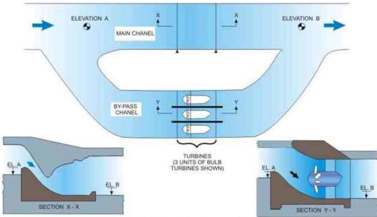
FIGURE 3. Canal Falls by-pass channel utilising the drop in canal elevation for power generation through bulb-turbines. Flow through the Canal Fall is usually controlled by a gate to allow flow through the turbines.
