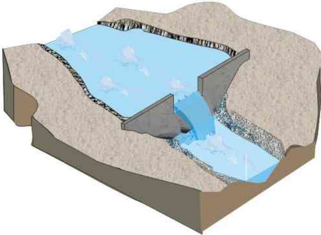
FIGURE 10. General view of a sharp created rectangular weir
