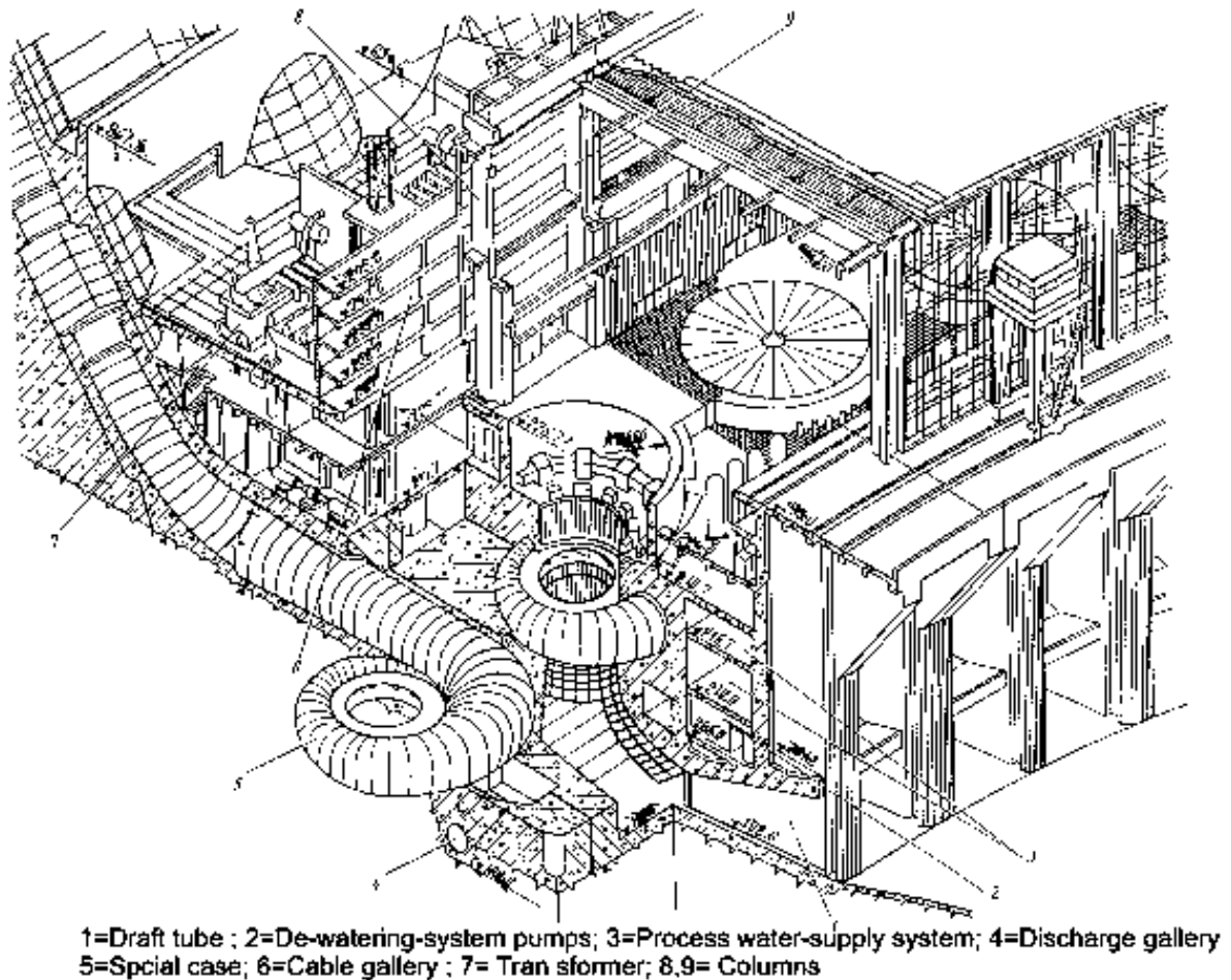
FIGURE 10. Cut-out view through the water passage and powerhouse of a reaction turbine
