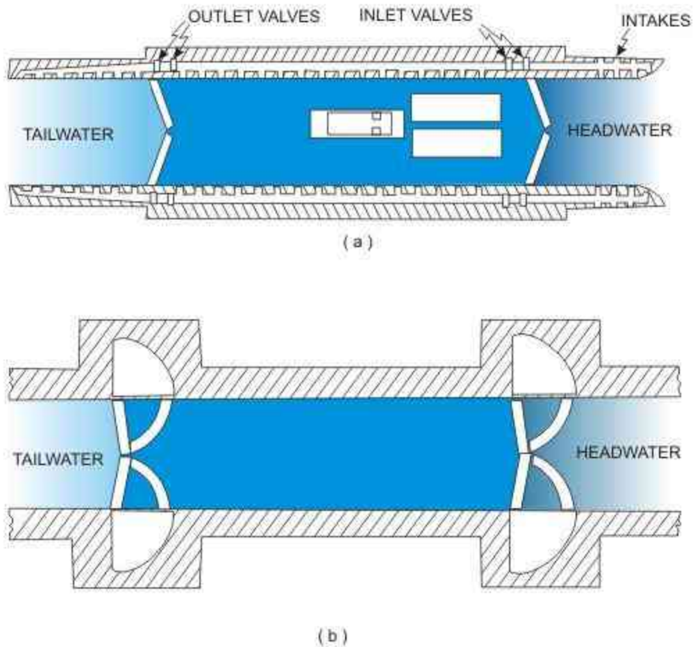
FIGURE 23. PLAN OF NAVIGATION LOCK
