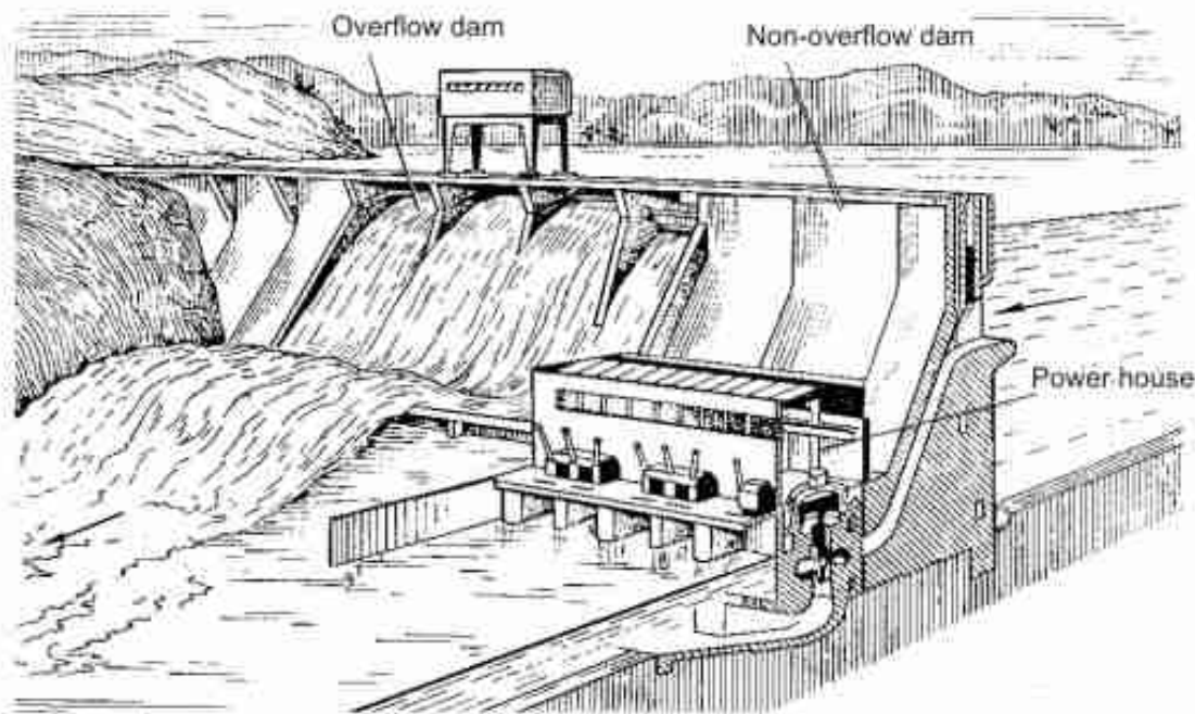
FIGURE 8. A typical storage-type hydroelectric station with a power house built at the toe of the dam
