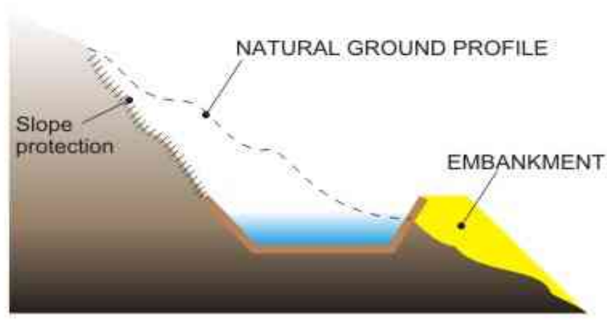
FIGURE 11. Cross section of a power canal in partly cutting & partly filling.
