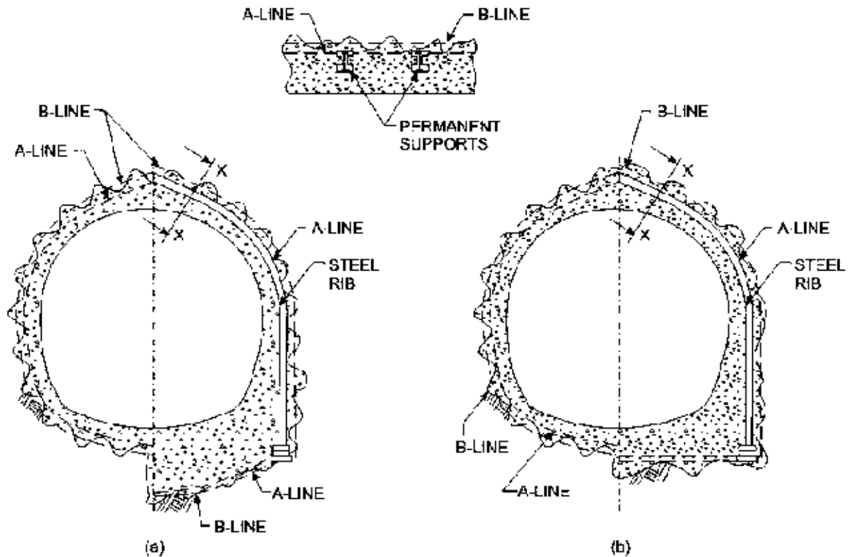
FIGURE 23. Steel support for tunnel and finished in the form of (a) Horse shoe section & (b) Circular section
