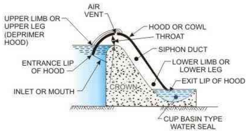
FIGURE 17. Saddle Siphon
