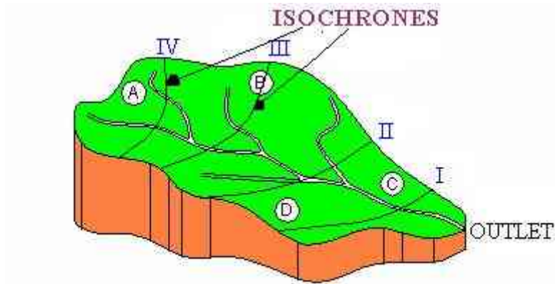
FIGURE 5. Typical isochrones over a catchment
