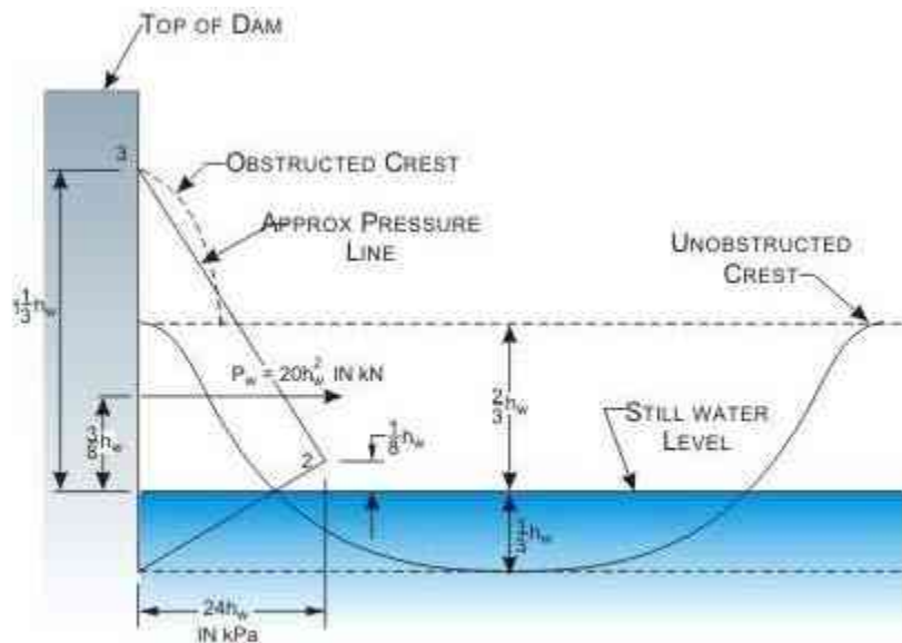
FIGURE. 36: Wave height, pressure and center of action
