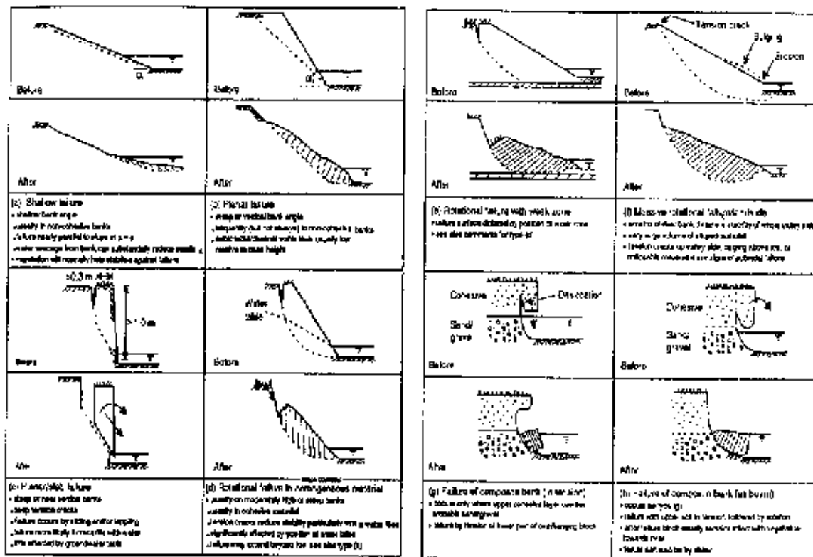
FIGURE 12. Modes of bank failure
