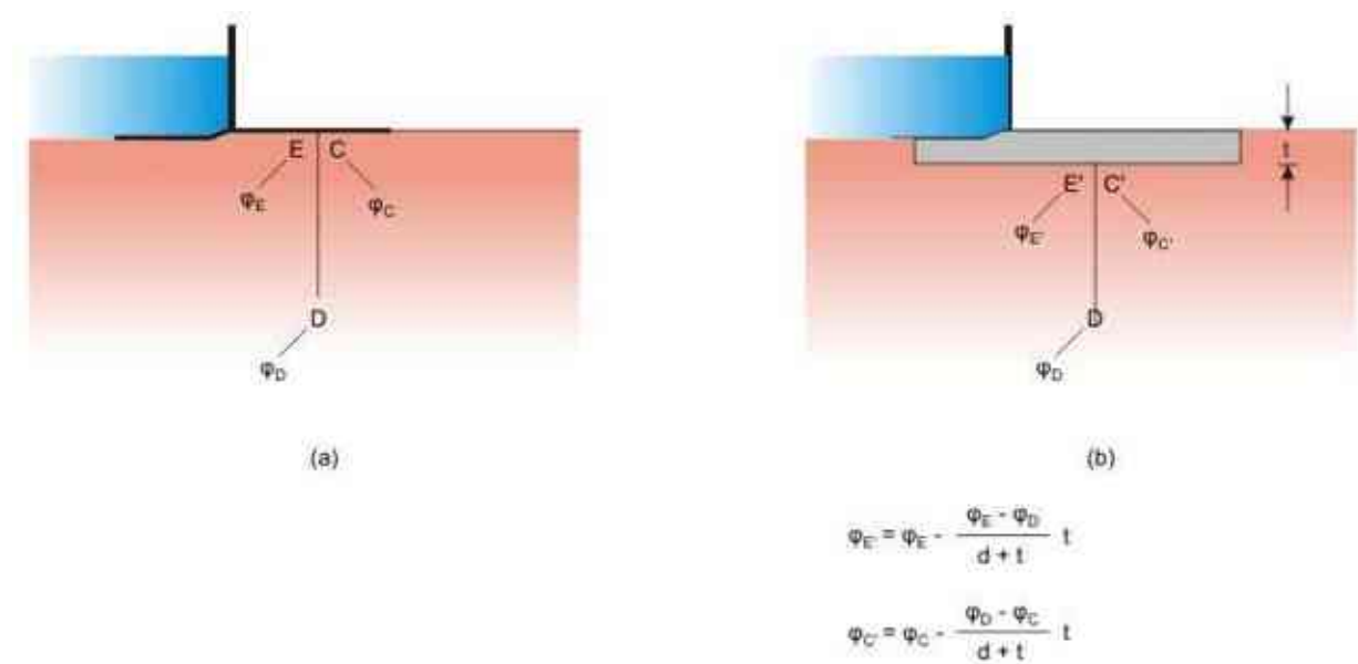
FIGURE 8. Correction to uplift for floor thickness (a) \phi_D , \phi_E and \phi_C as obtained from simplified formulae ; (b) Corrected values \phi_{E'} and \phi_{C'} at the same location considering thickness of floor
