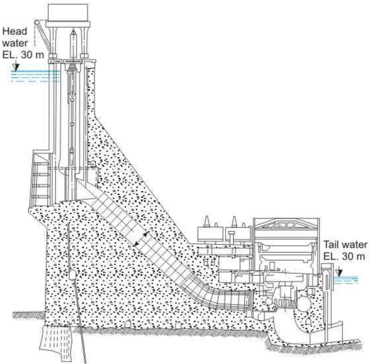
FIGURE 13. Sectional view of a typical medium head hydropower station.
