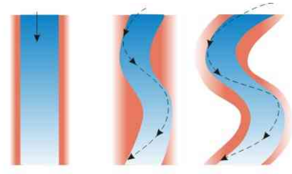
Figure 11. Sinuosity for a straight and meandering river (a) Straight: Sinuosity = 0; (b) Sinuosity = 1.1 ; and (c) Sinuosity = 1.5
