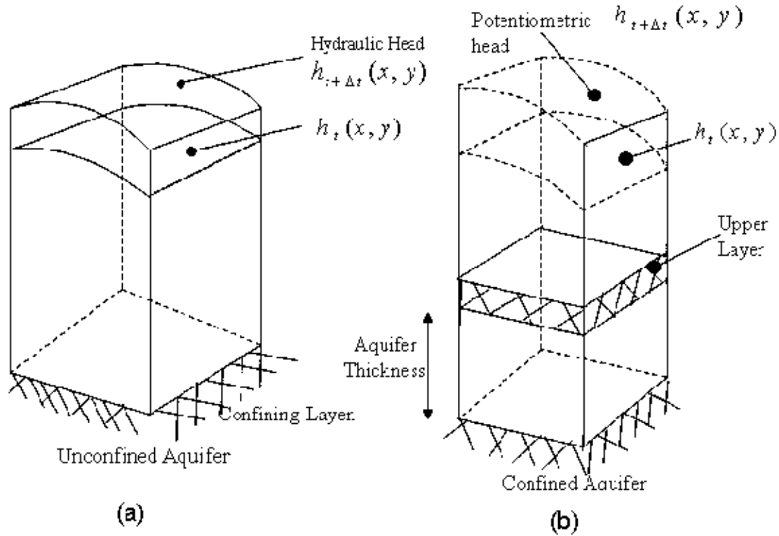
FIGURE 3. (a) Free surface of ground water table in unconfined aquifer (b) Potentiometric surface in confined aquifer
