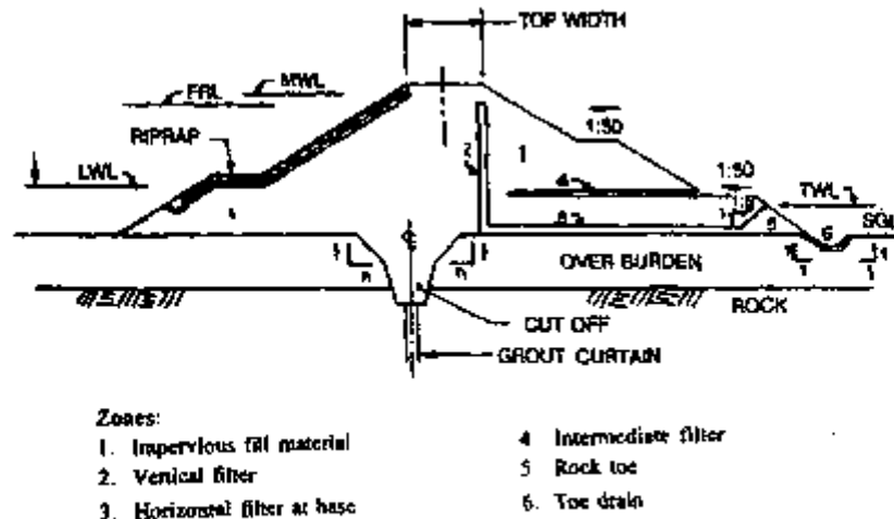
FIGURE 35. Section of homogeneous dam showing seepage control features
