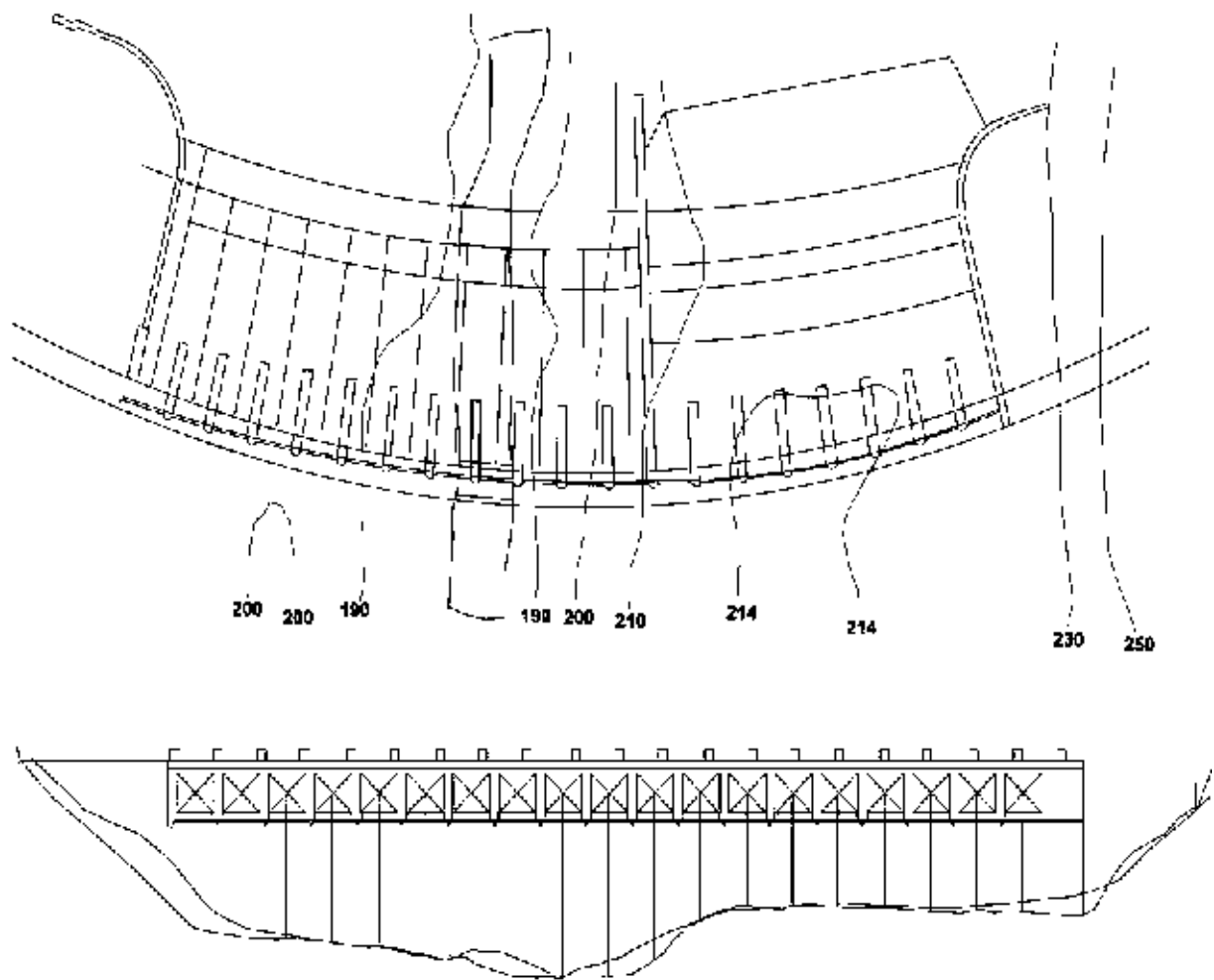
Figure 30. Detailed plan of the Indira Sagar dam and upstream elevation
