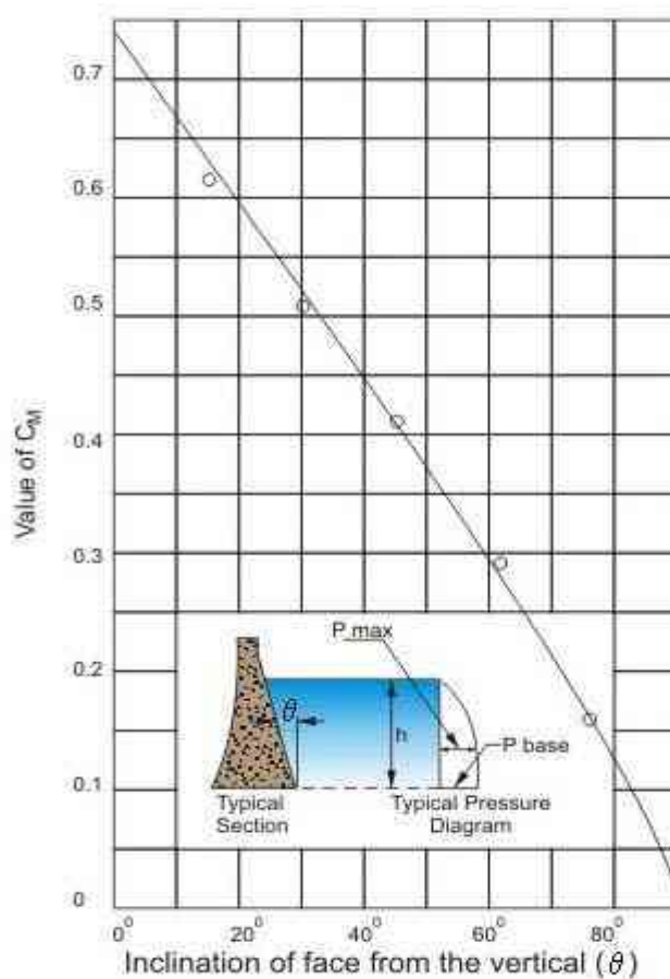
FIGURE.35: Maximum values of pressure coefficient ( C_M ) for dams with constant sloping faces
