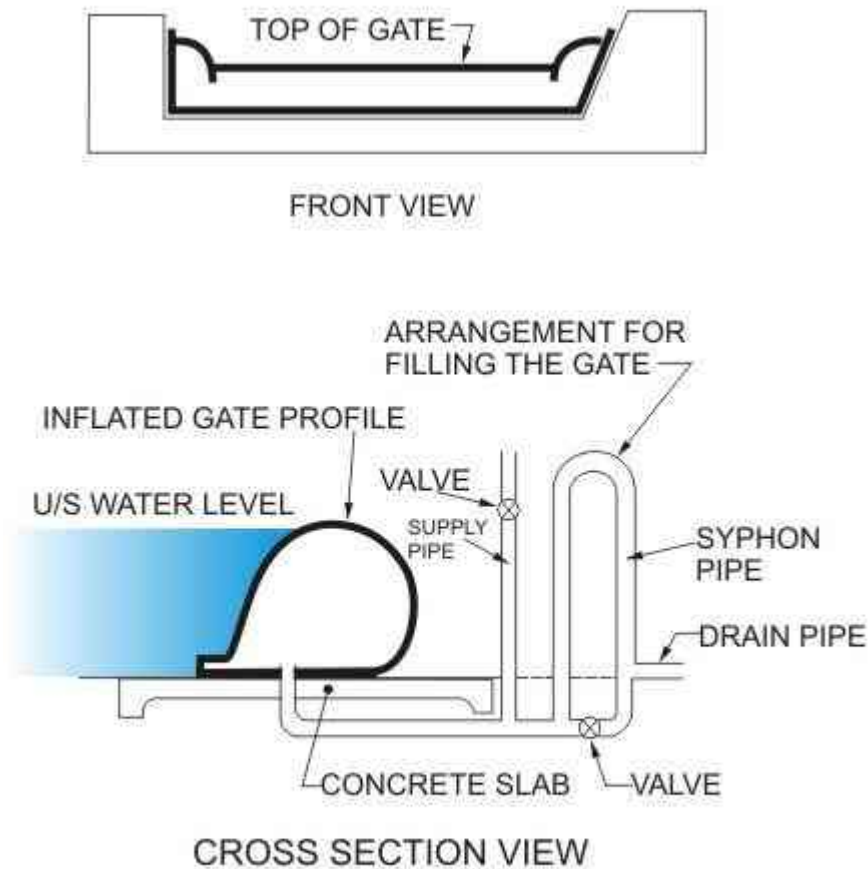
FIGURE 8 : INFLATABLE GATE
