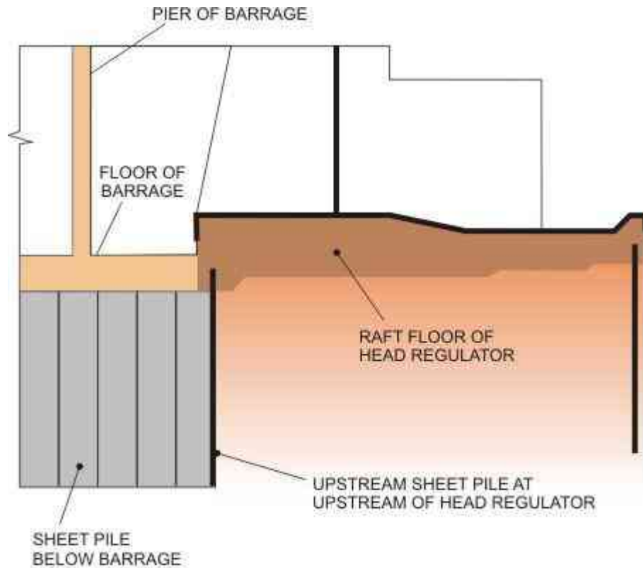
FIGURE 11. Sheet pile on the upstream of head regulator floor
