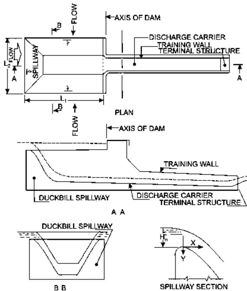
FIGURE 20. Duckbill Spillway
