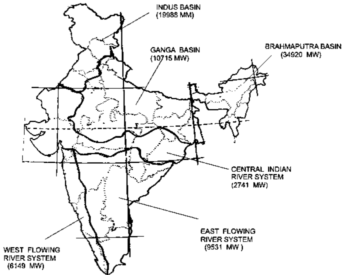
FIGURE 5. Basin-wise hydro power potential of India.
