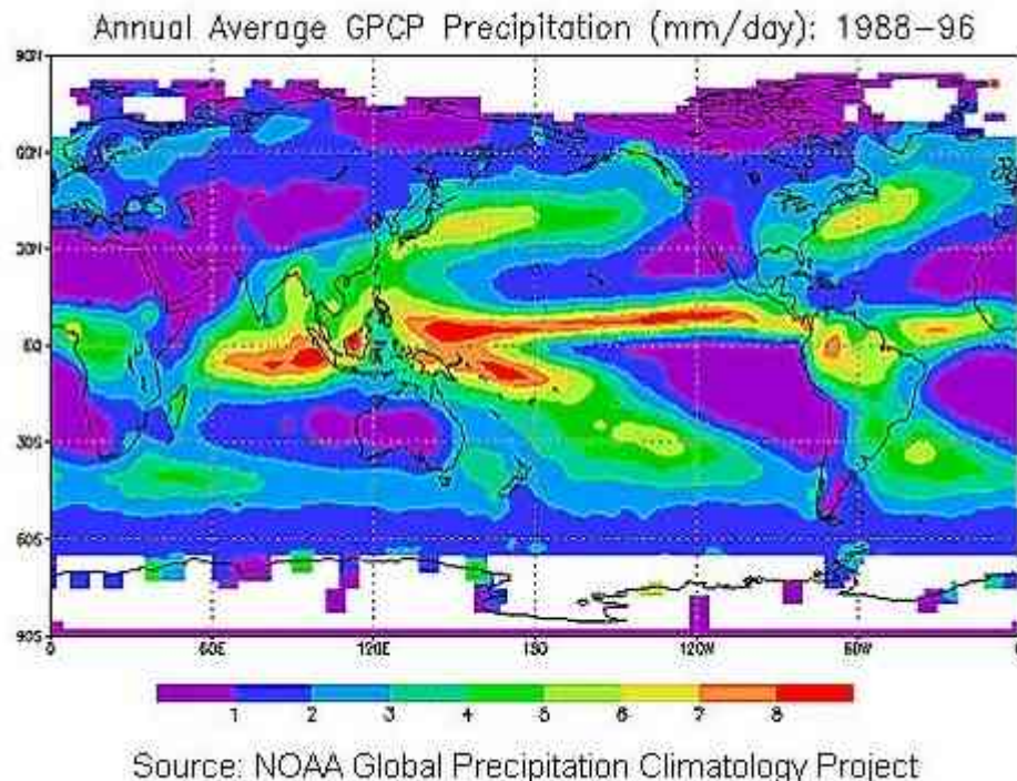
Figure 4. A typical distribution of global precipitation (Courtesy: Global Precipitation Climatology Project)
