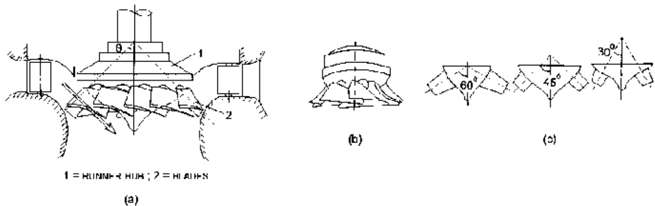
FIGURE 5. Adjustable-blade diagonal (Deriaz) turbine
