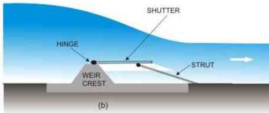
Fig.10: Manually operated falling shutter (a) Closed Position, (b) Open Position
