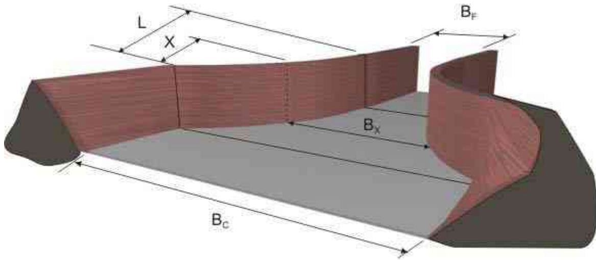
FIGURE 19. Transition canal banks warped to vertical and then flumed
