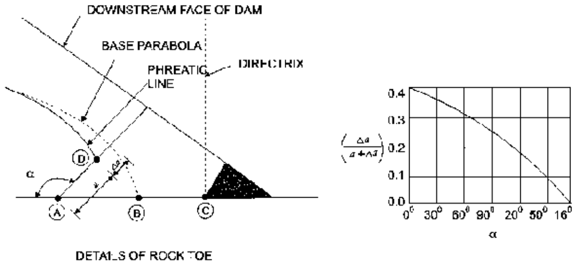
FIGURE 52. Determination of point of attachment (B) of phreatic line and upstream face of rock toe
