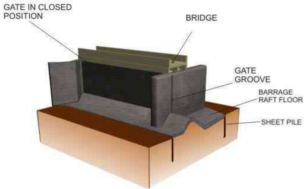
FIGURE 2B. Section through a barrage (with vertical lift gate) showing raft foundation and sheet piles. Gate hoisting arrangement not shown.
