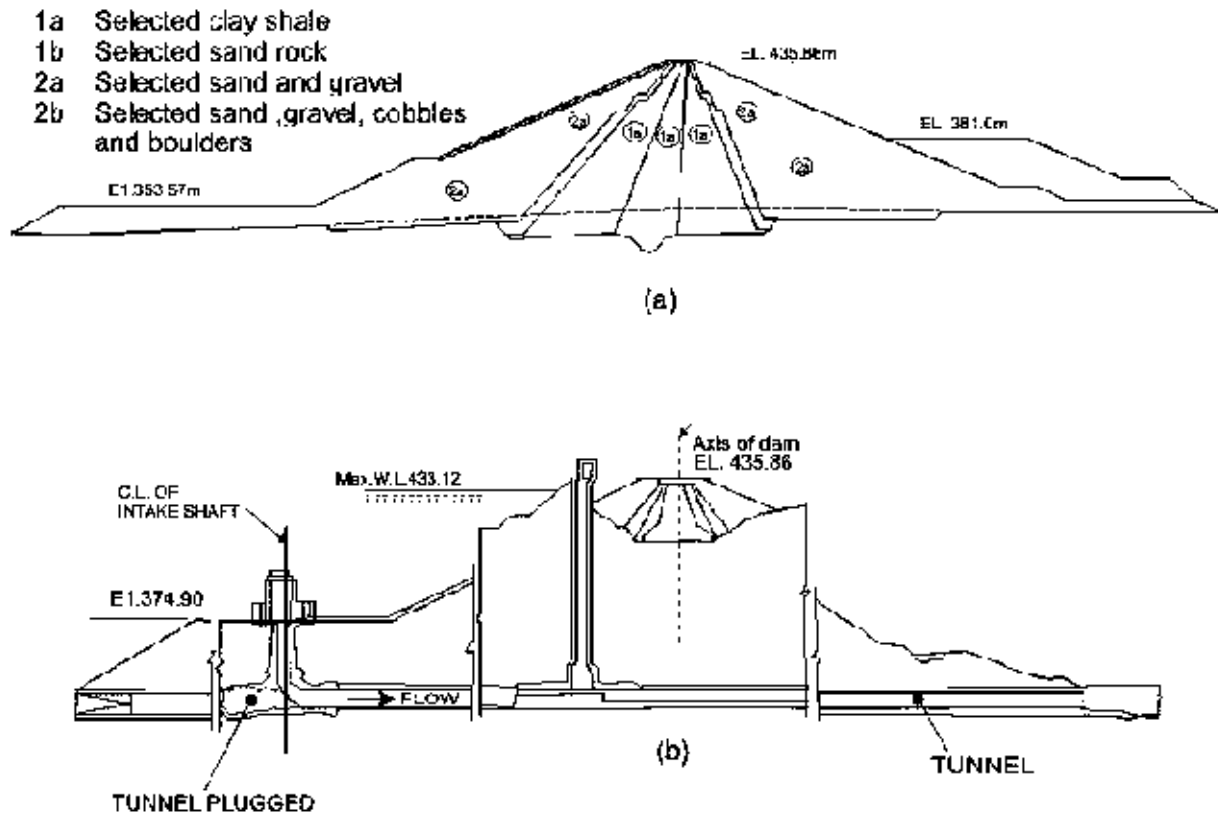
Figure 19. Beas dam at Pong (a) Maximum section of earth dam (b) Outlet work for power house through earth dam section
