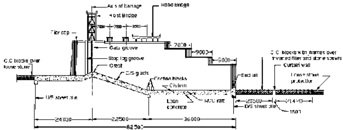
FIGURE 16 Typical section of undertuice without silt excluding tunnels
