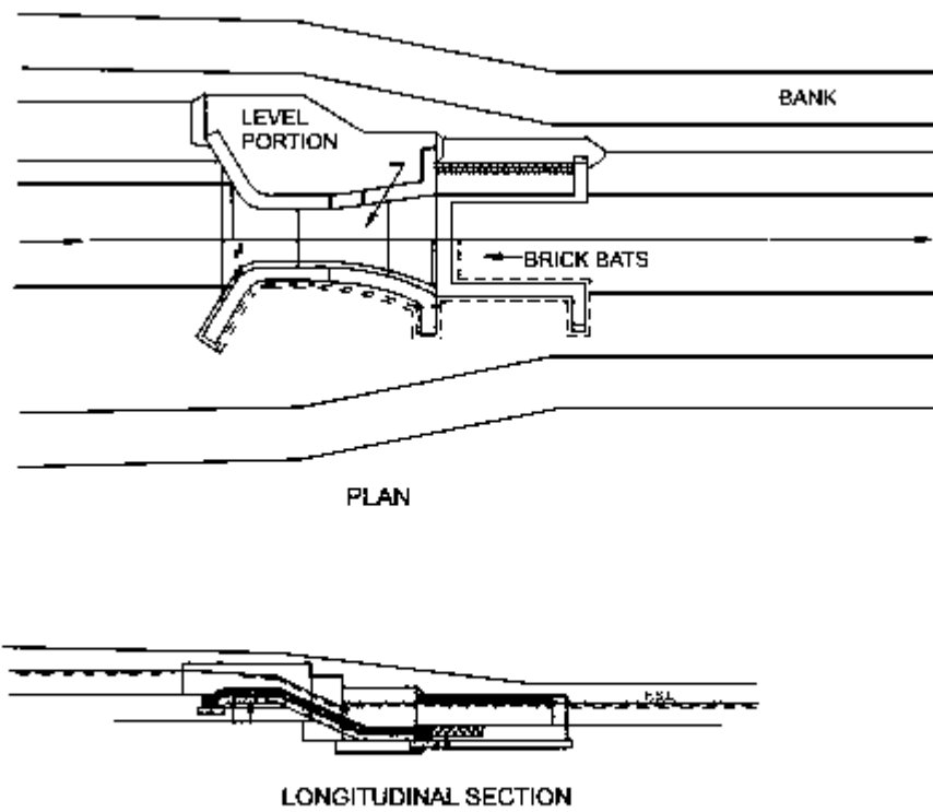
FIGURE.15. CDO PUNJAB TYPE FALL UPTO 1m DROP
