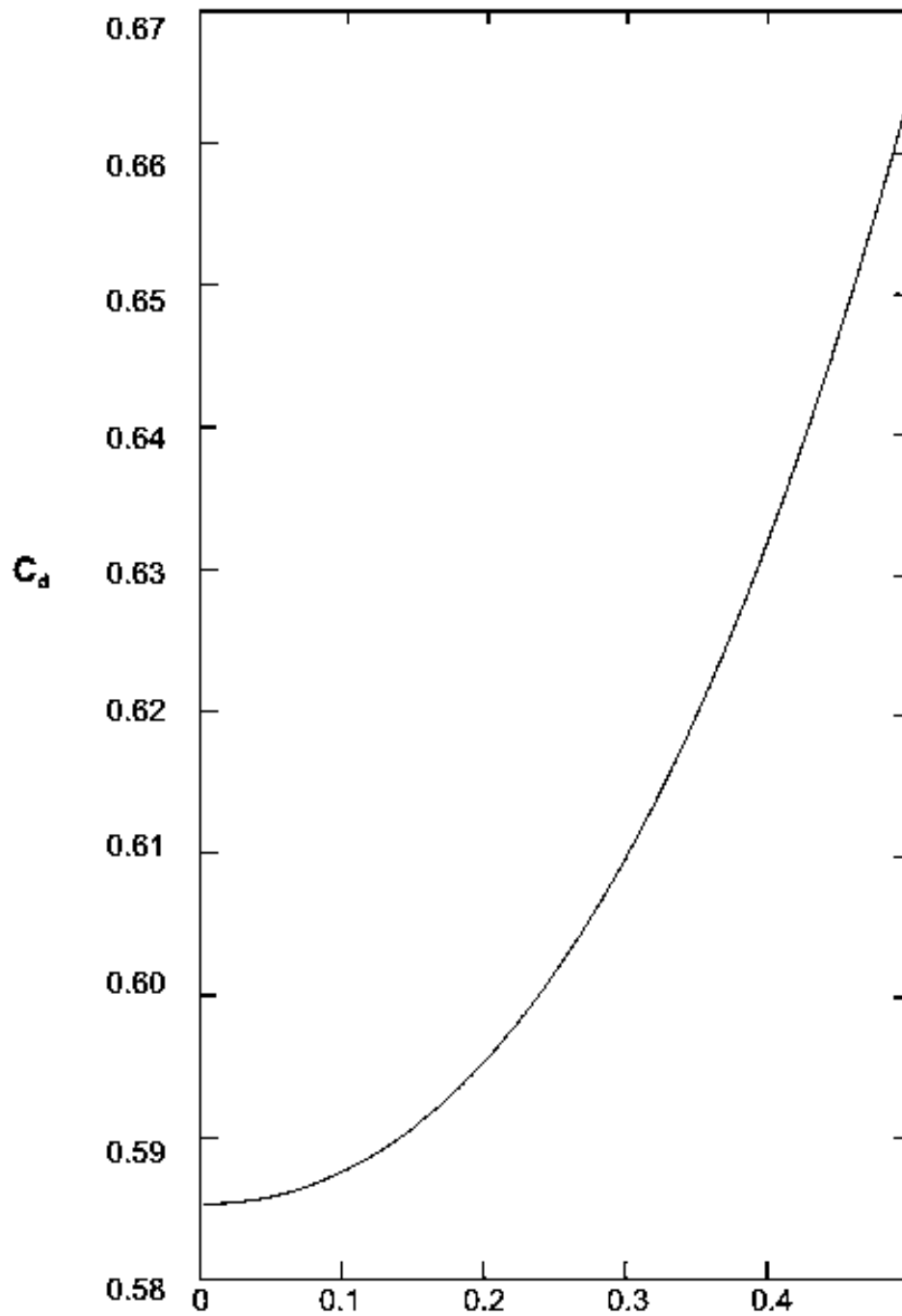
FIGURE 13. Variation of C_d for 90° V-Notch weir with H^2/A
