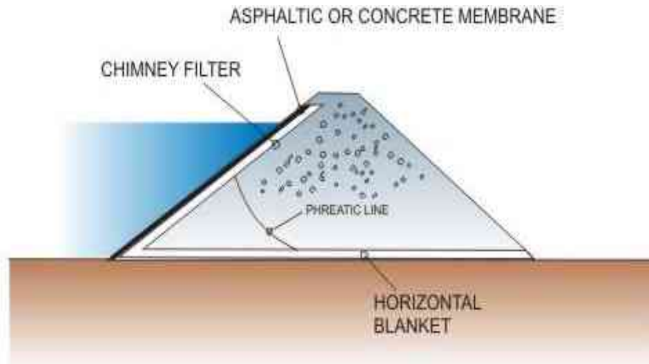
FIGURE 10. Decked rock fill dam with upstream asphaltic or concrete membrane with chimney drain and horizontal blanket. The phreatic line is for the small amount of water that leaks through the cracks of the upstream membrane.
