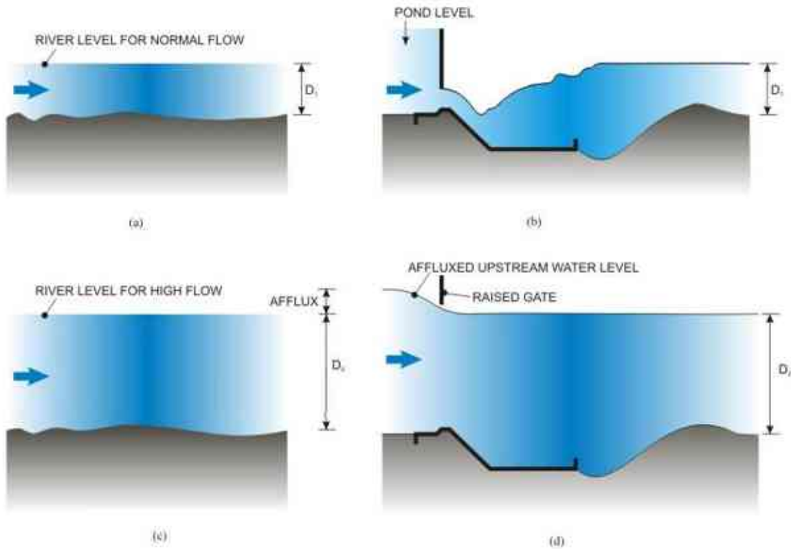
FIGURE 7. Afflux explained. (a) River at normal flow: Depth almost same as on the downstream of a ponded flow as in (b). (c) River at flood level: Downstream depth almost the same as that of the original river; upstream depth higher than downstream depth, the difference being called Afflux as in (d).
