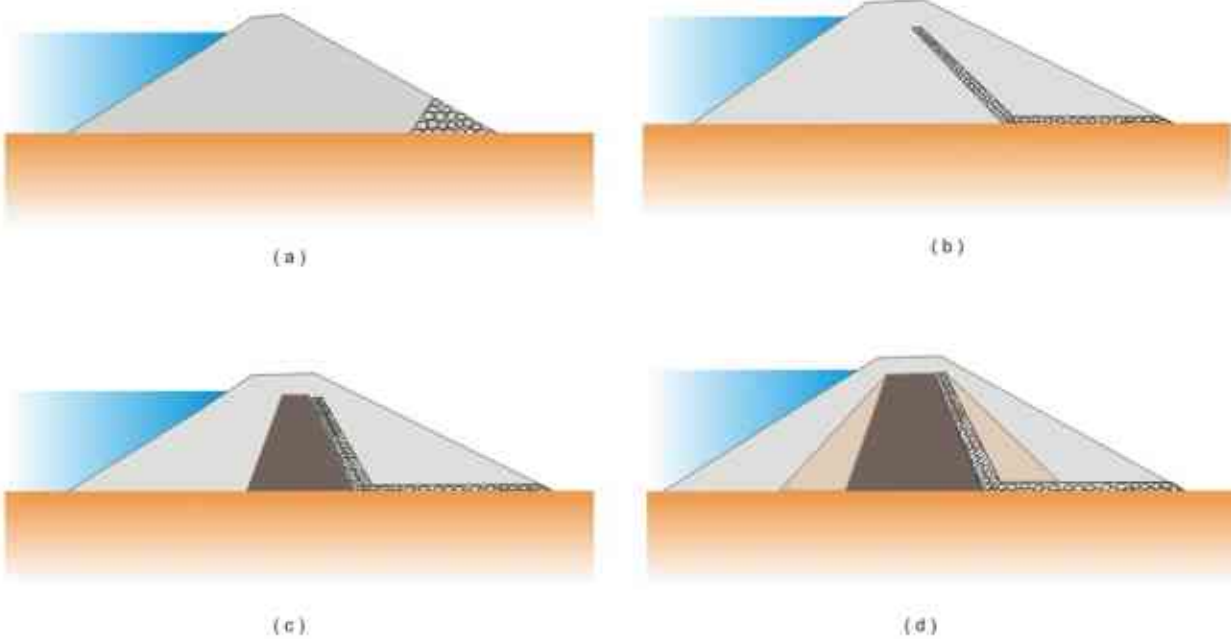
FIGURE 2. Principal types of earthen embankment dams (a) Homogeneous with toe drain, (b) Homogeneous with chimney drain & horizontal blanket, (c) Zoned with clay core chimney drain & horizontal blanket, (d) Zoned with earth & rockfill
