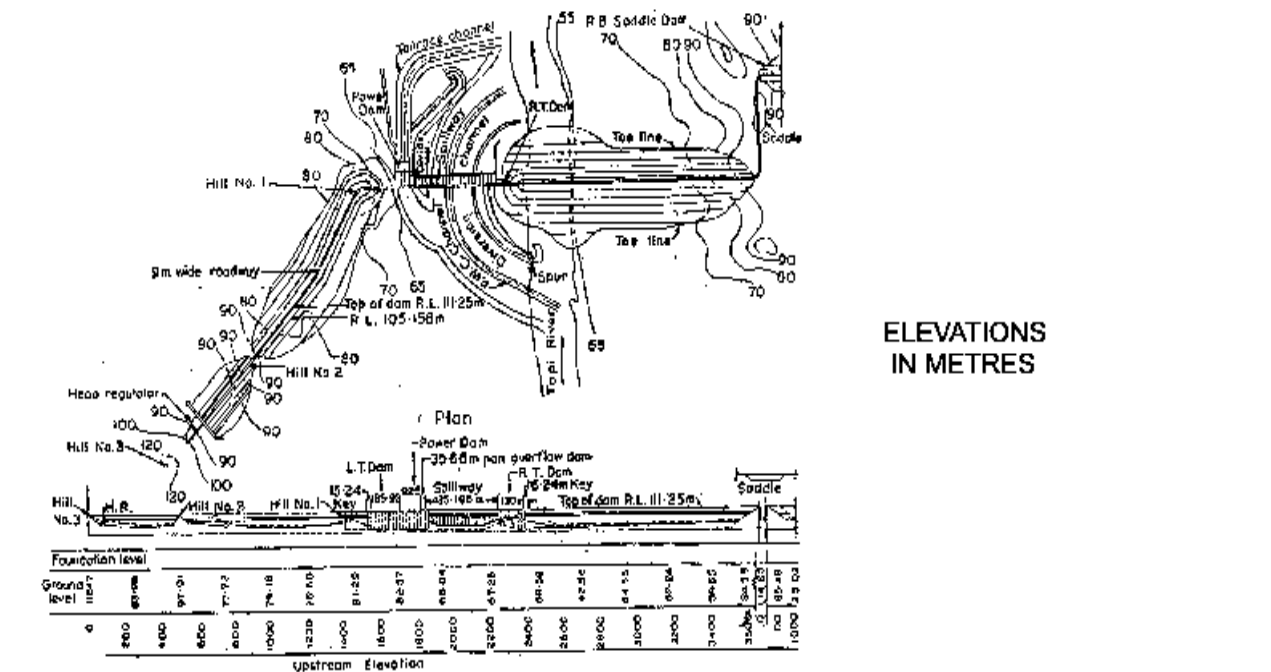
FIGURE 14 . Layout of Ukai dam- showing concrete spillway and embankment dam
