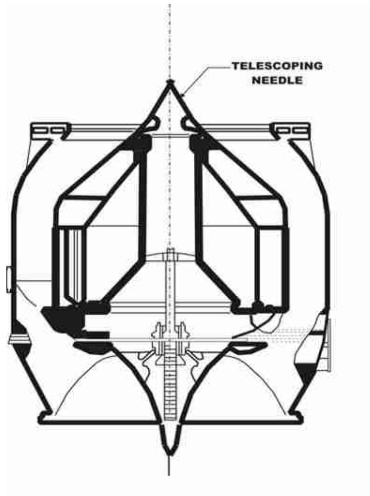
FIGURE 35. Interior differential needle valve
