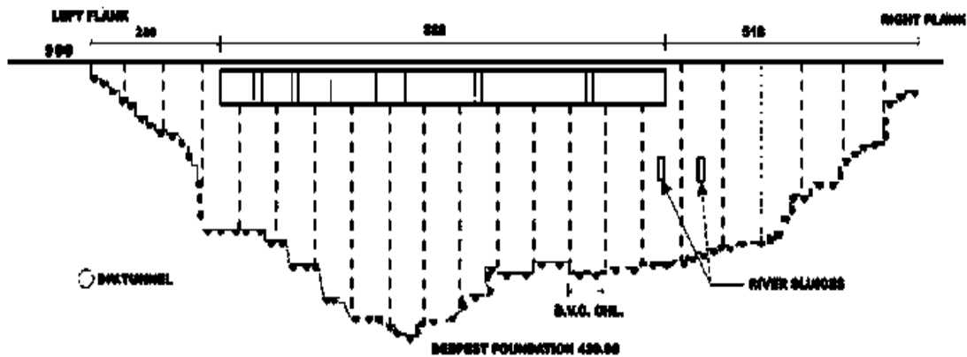
Longitudinal section of the Srisailem Dam along reference line
