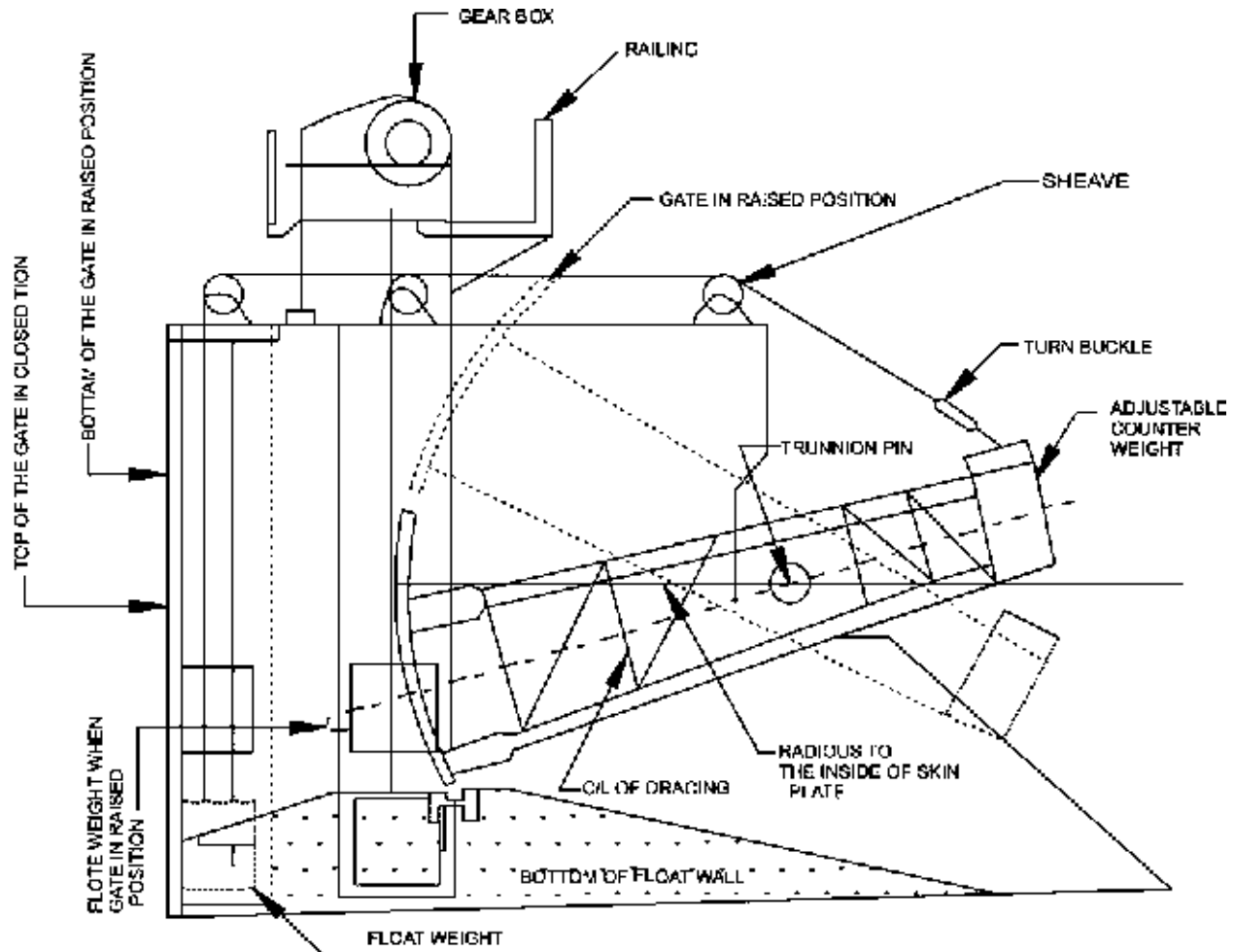
FIGURE 11. AUTOMATIC FLOAT OPERATED RADIAL GATE
