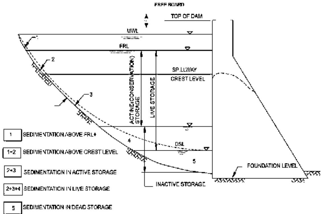
FIGURE 2. SCHEMATIC DIAGRAM SHOWING ZONES OF RESEERVOIR SEDIMENTION
