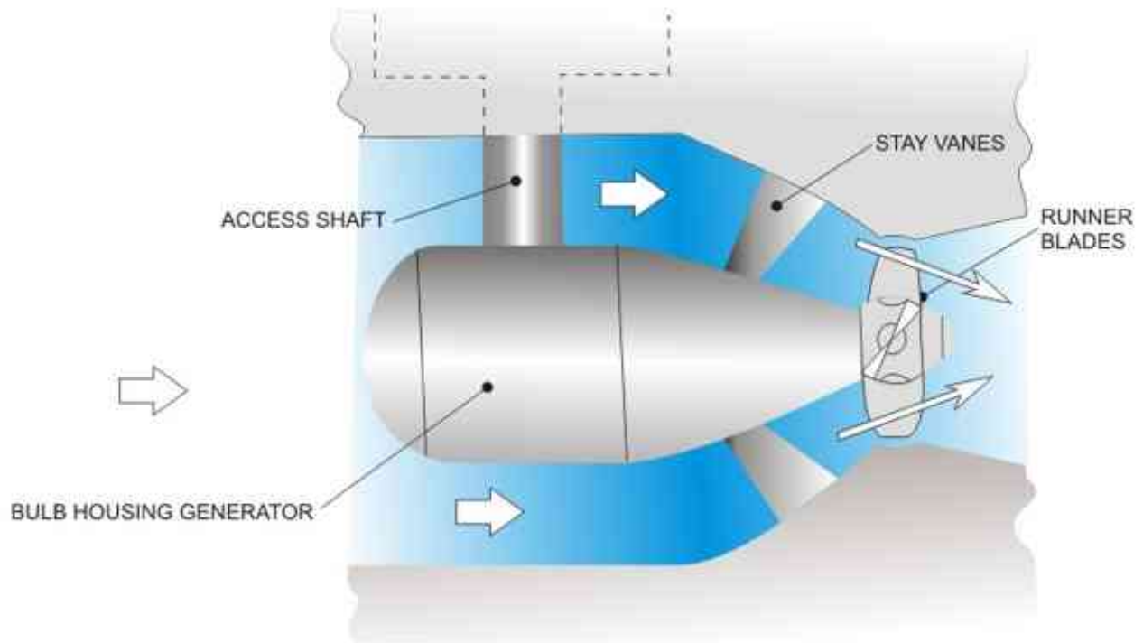
FIGURE 6. Axial - flow bulb turbine
