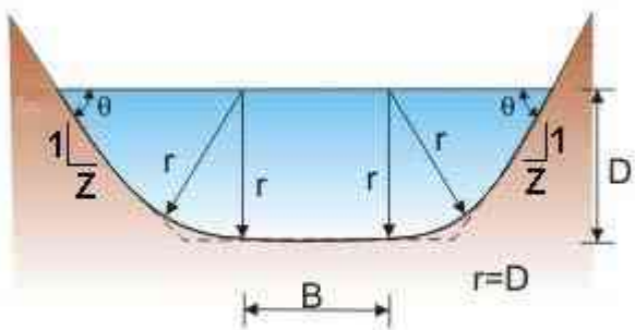
FIGURE 2. Trapezoidal channel section
