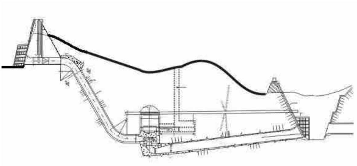
FIGURE 23 Underground power house of Sardar Sarovar Dam project
