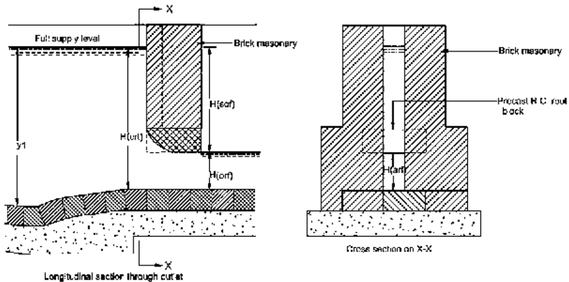
FIGURE 8.DETA-LS OF BLOCK FOR ADJUSTABLE PROPORTIONAL MODULE
