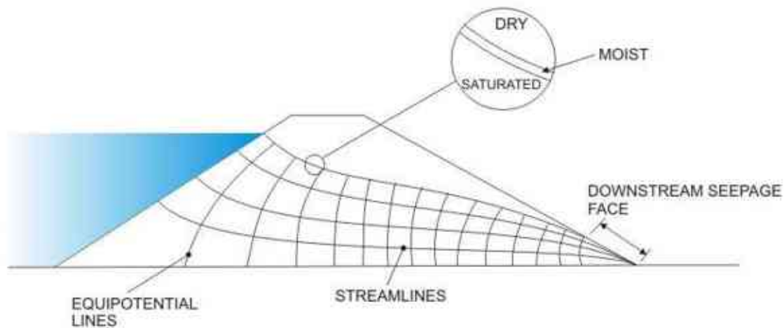
FIGURE 49. Flow net showing equipotential and streamlines for saturated flow through a homogeneous embankment dam
