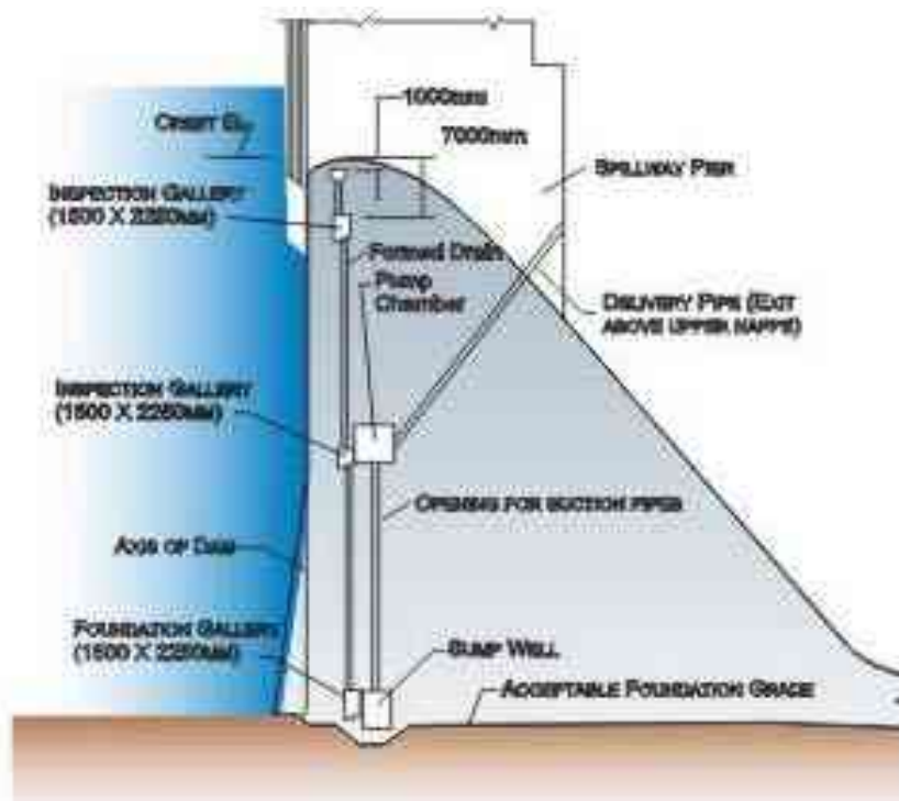
FIGURE 21. Galleries in a non-overflow section of a typical concrete gravity dam.
