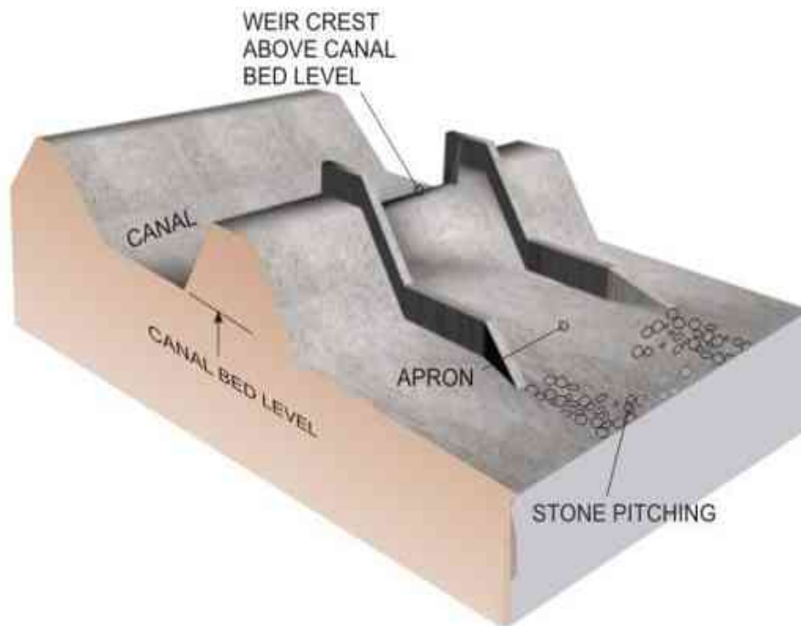
FIGURE 26. Weir Escape
