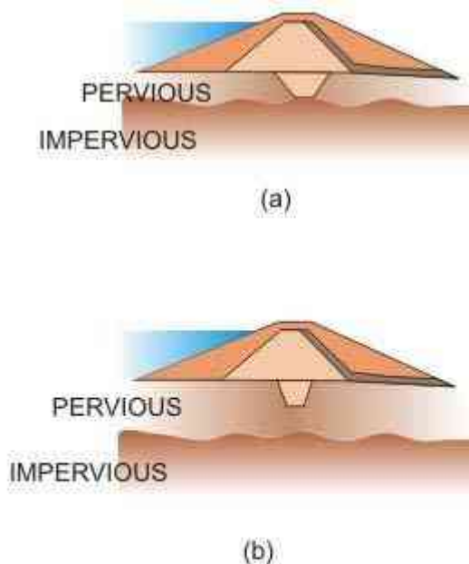
FIGURE 45. Cut off trenches (a) Positive cut-off (b) Partial cut-off
