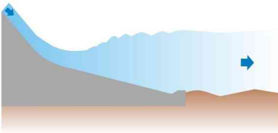
FIGURE 58. Inclined stilling basin
