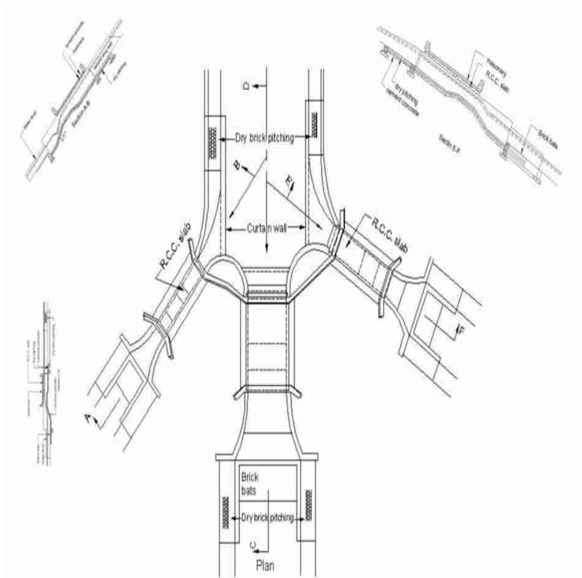
FIGURE 2. Proportional distributor structure with two offtakes
