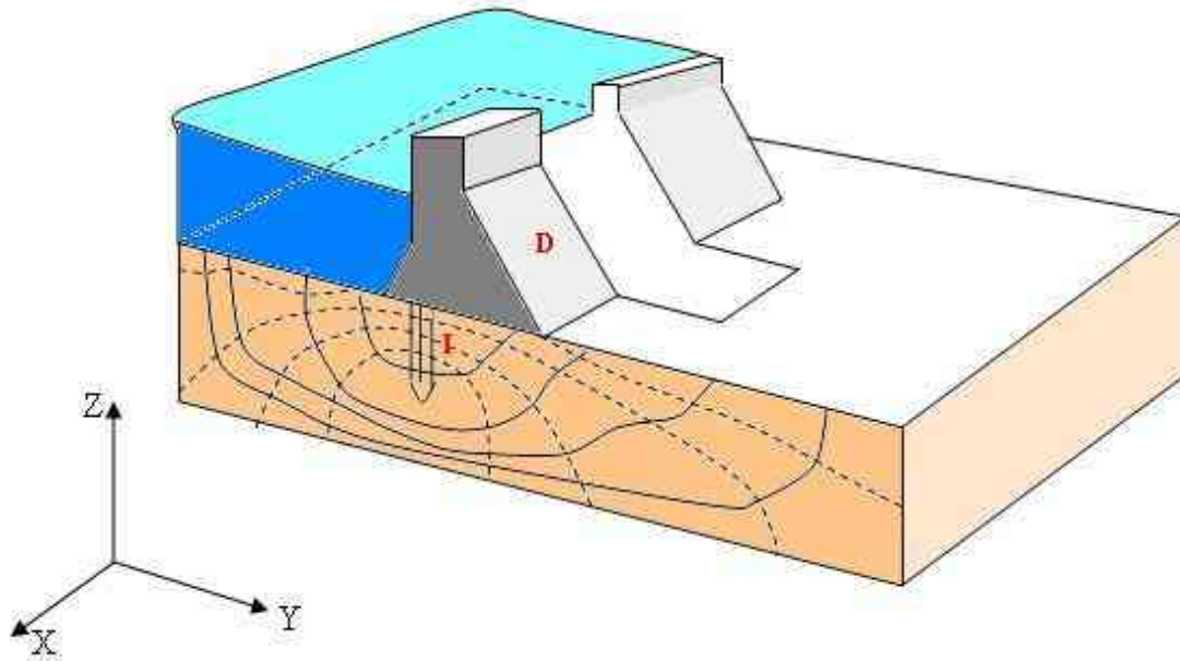
FIGURE 5. Seepage flow below a concrete gravity dam
