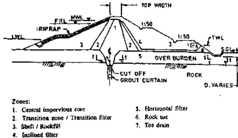
FIGURE 36. Section of zoned dam showing seepage control features
