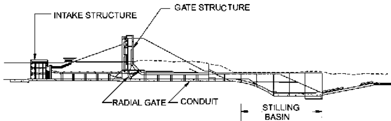
FIG4. OUTLET WITH A TRASH-RACK BOX INTAKE,PRESSURE CONDUIT ON UPSTREAM AND FREE FLOW CONDUIT ON DOWNSTREAM
