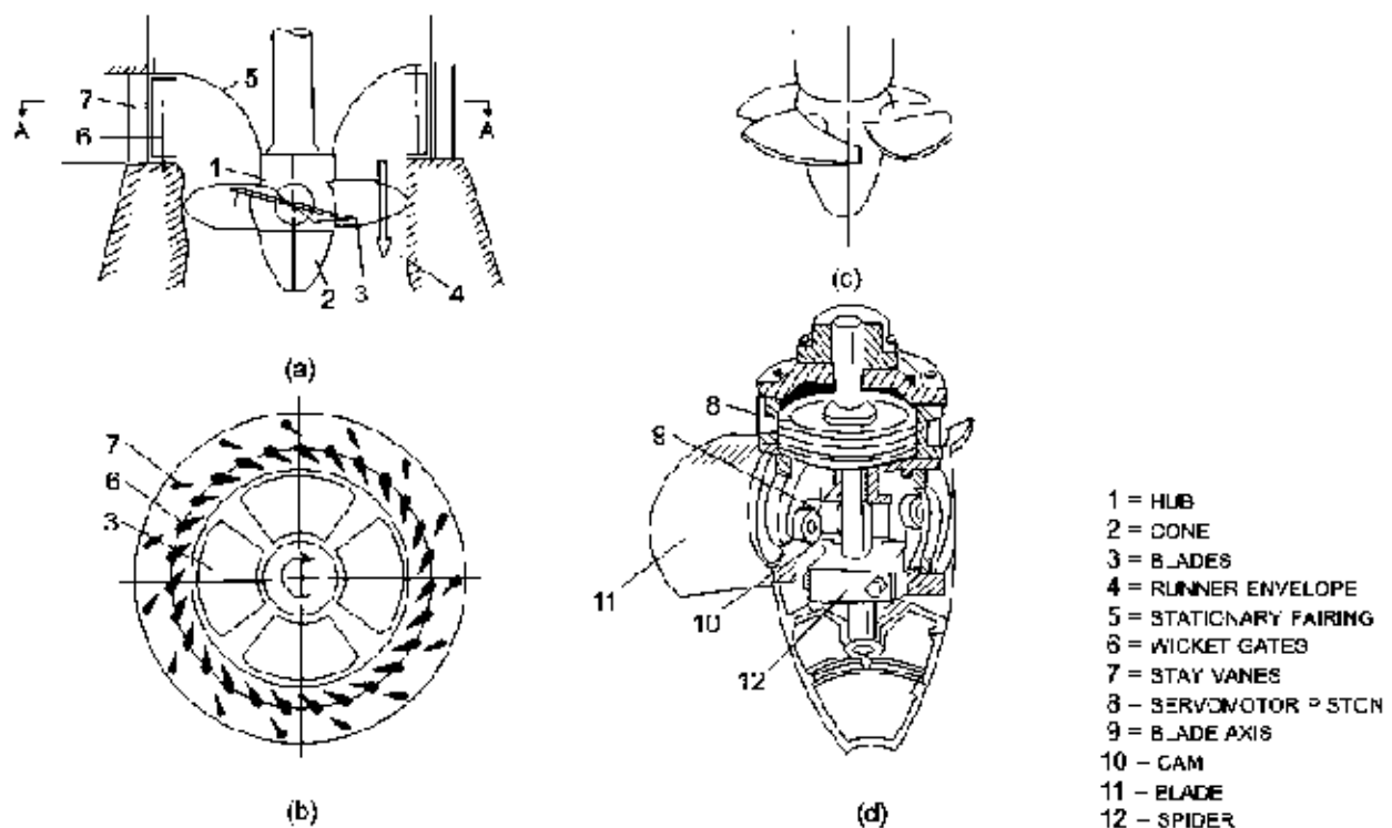
FIGURE 3 Adjustable-blade propeller (Kaplan) turbine (a) Cross-sectional elevation; (b) Horizontal section A-A through runner; (c) General appearance of runner; (d) Section through blade adjustment mechanism
