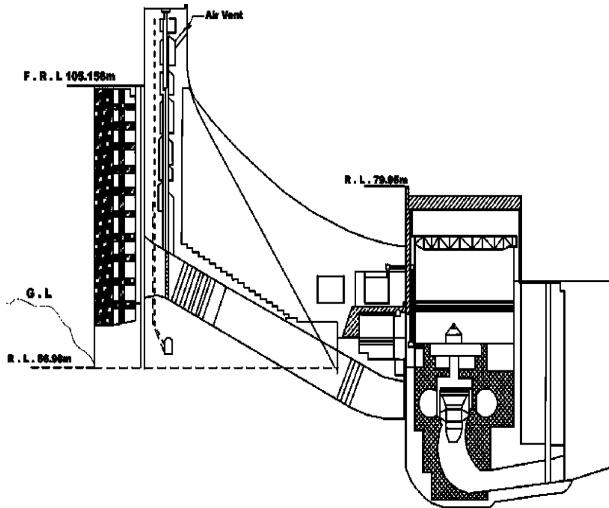
FIGURE 20. Power dam section of Ukai project
