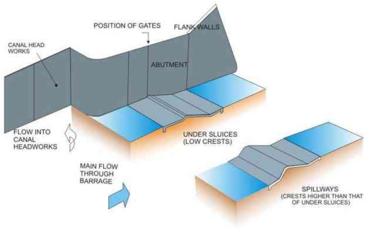
FIGURE 12. Relative shapes of under sluice bays (towards the canal end) and spillway bays of a barrage. Piers, gates and walls have not been shown.
