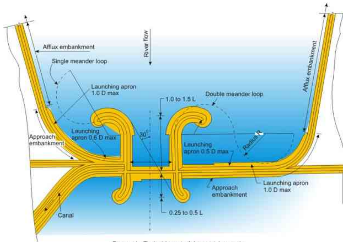
FIGURE 1. Typical layout of river training work.
