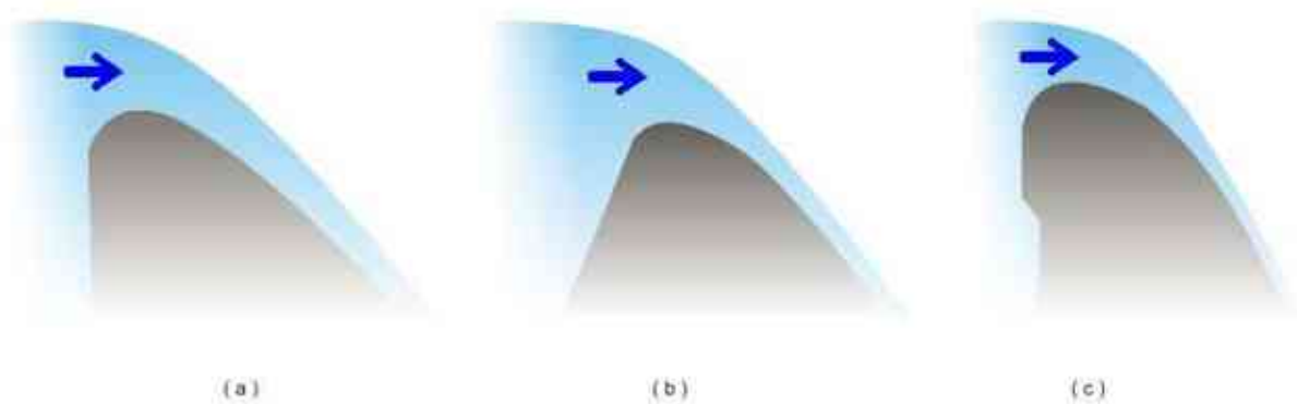
FIGURE 21. Ogee crest control weirs with (a) Vertical upstream face (b) Inclined upstream face (c) Overhangs on the upstream
