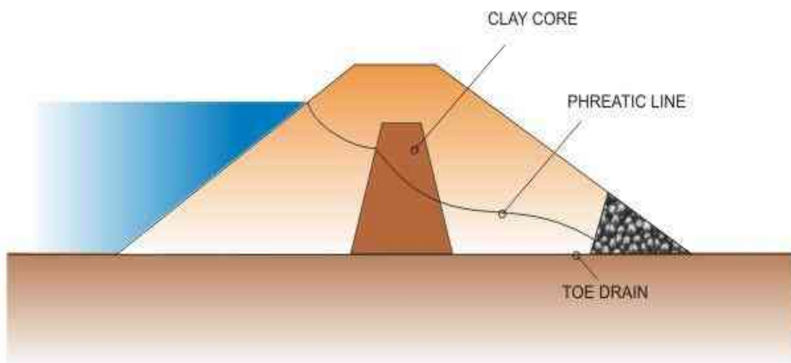
FIGURE 5. Zoned dam with central vertical clay core and toe drain
