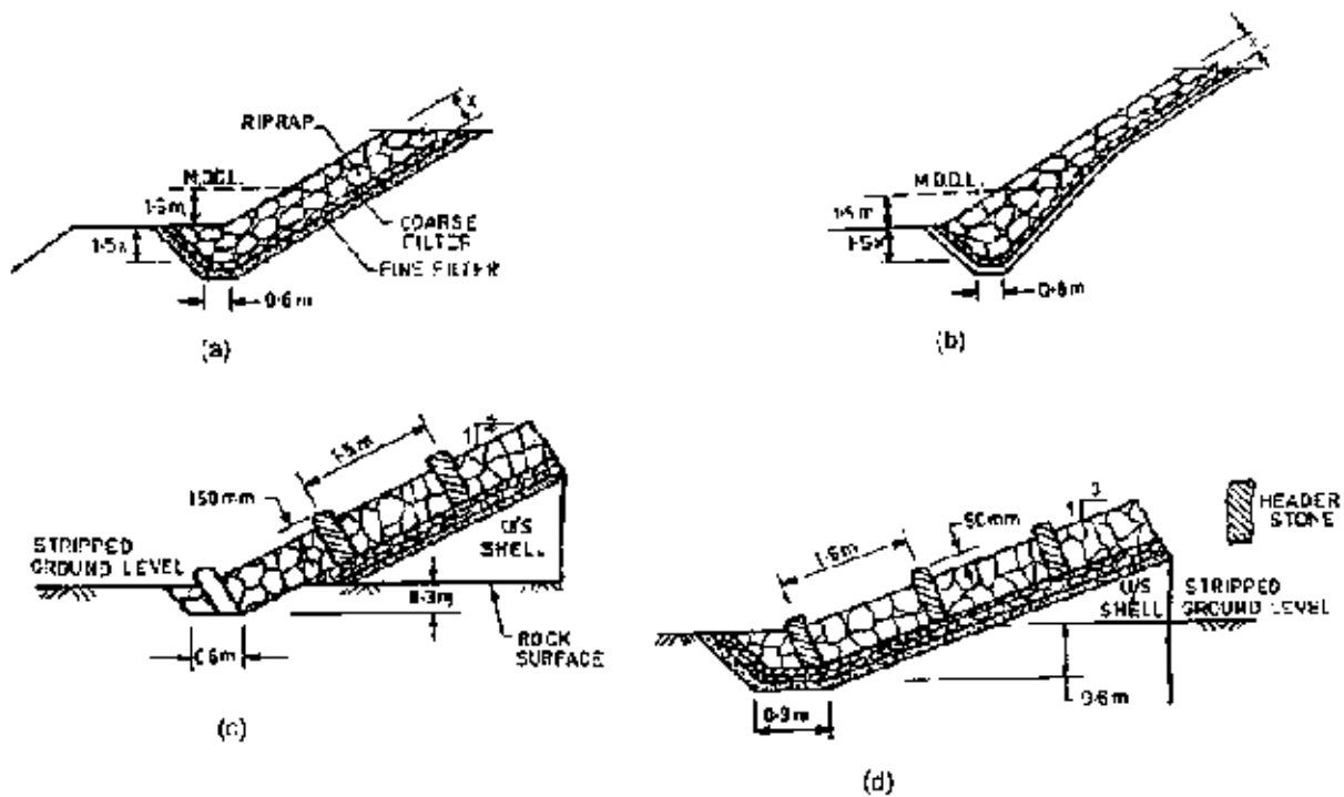
FIGURE 33. Pitching of rip rap (a) With berm below MODL, (b) Without berm below MODL, (c) Terminating at rock surface; (d) Terminating at stripped ground level
