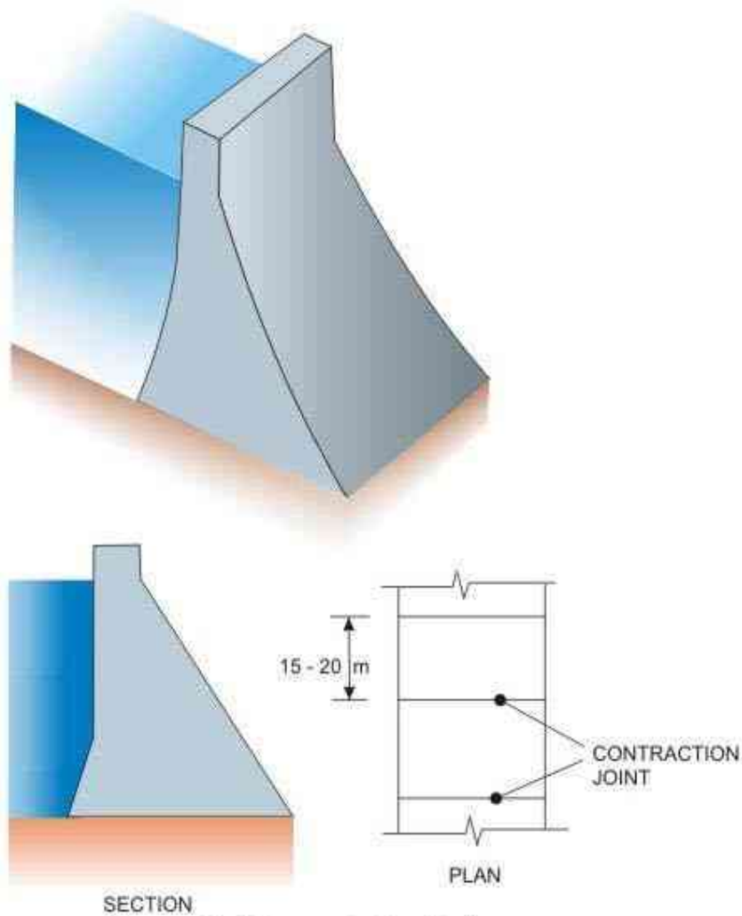
FIGURE 4(a) Concrete Gravity dam
