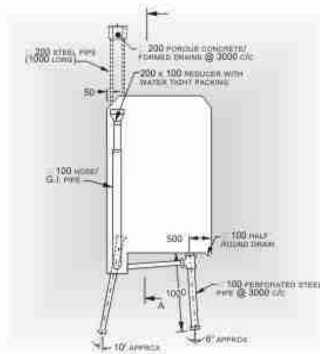
FIGURE 16. Details of a foundation drainage gallery
