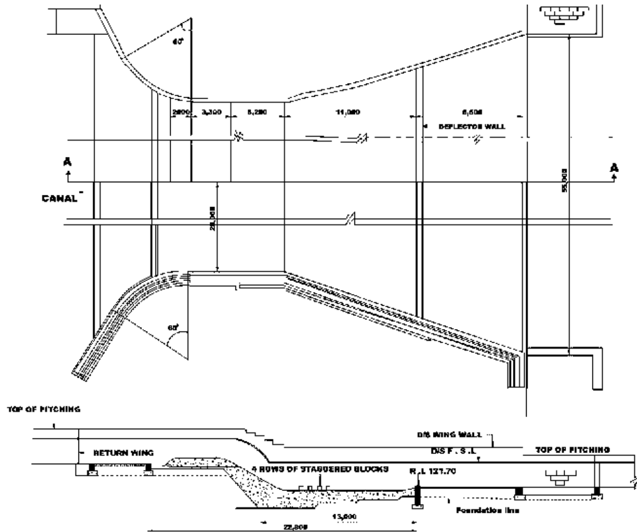
FIGURE 14 Flumed glauis wall: metered fall
