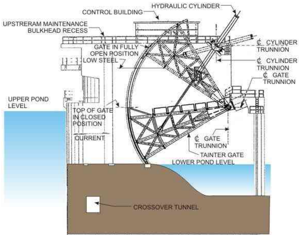
FIGURE 30. HYDRAULIC HOIST OPERATED TAINTER GATE
