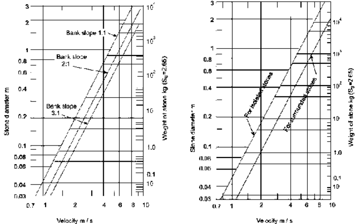
Figure 3. Graph for determining pitching and stone aprons.
