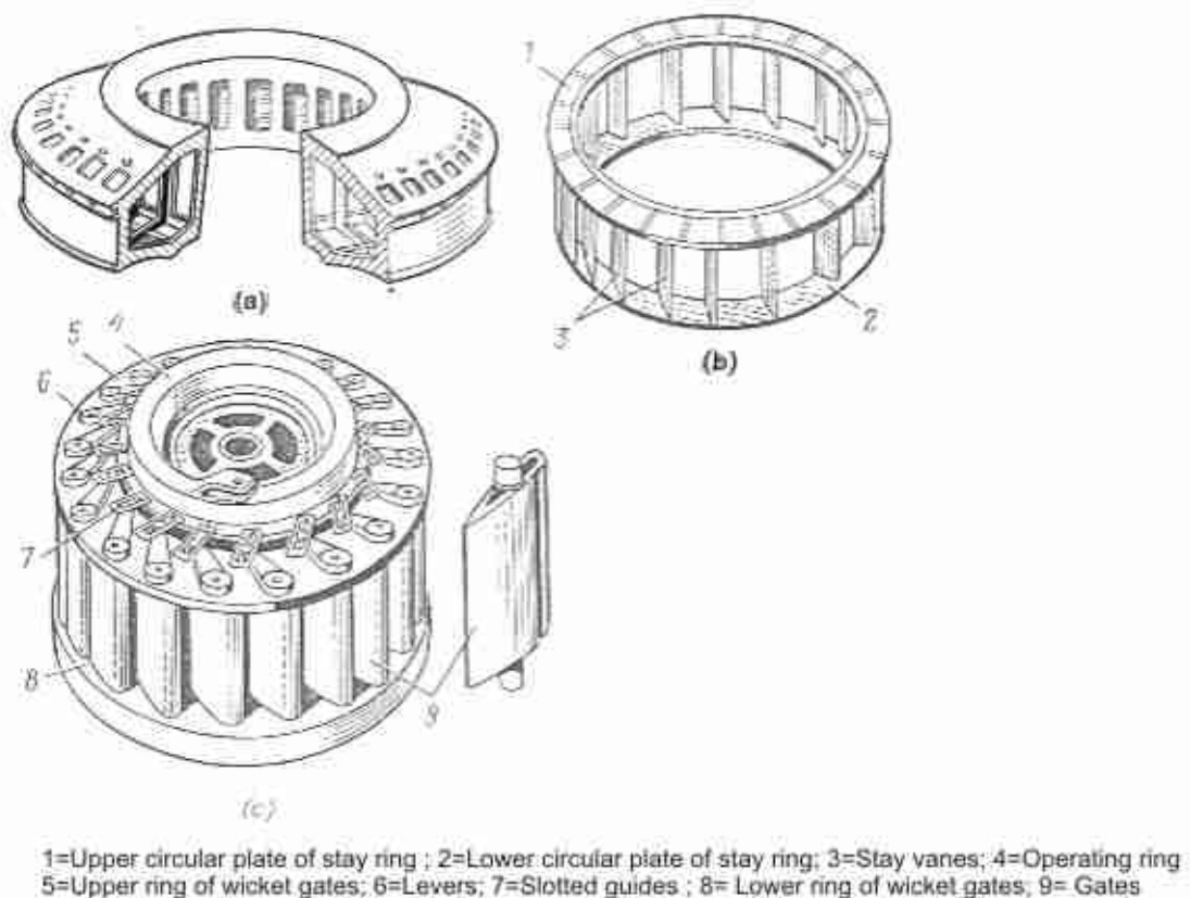
FIGURE 2. Stationary components of a reaction turbine (a) Cover ; (b) Stay ring ; (c) Wicket gates
