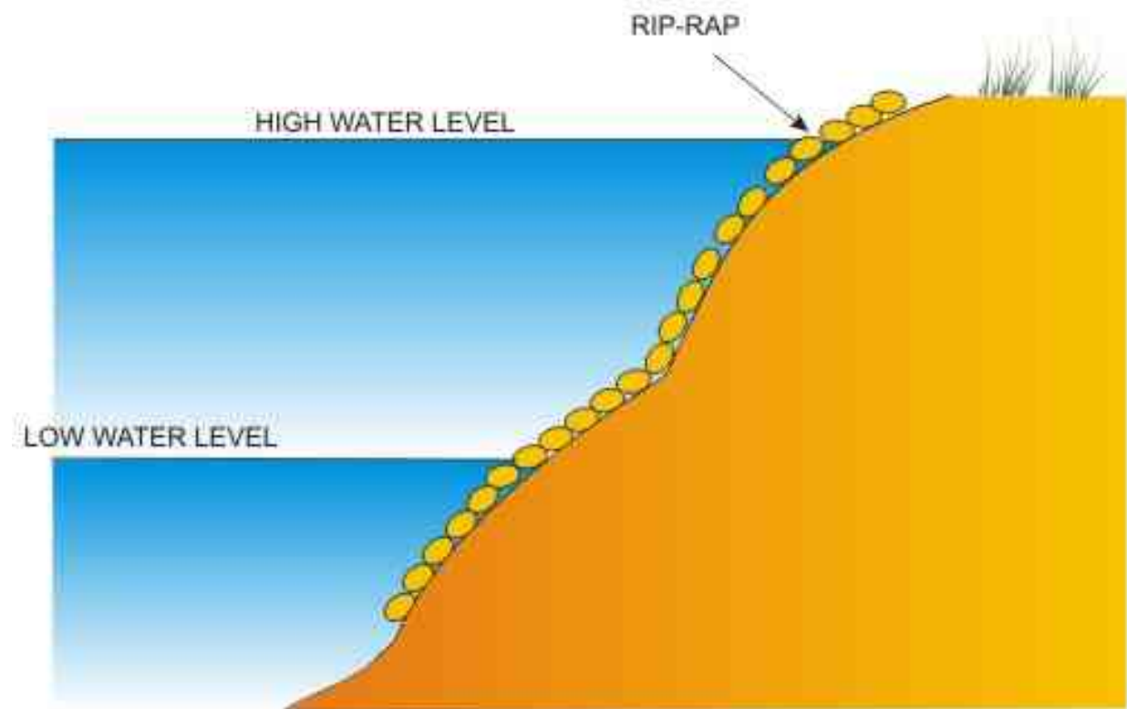
FIGURE 11. Typical river bank section shown protected by riprap blanket
