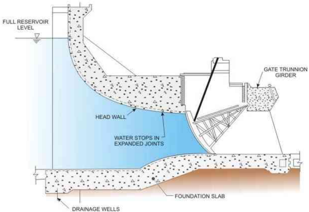
FIGURE 19. Sluice spillway
