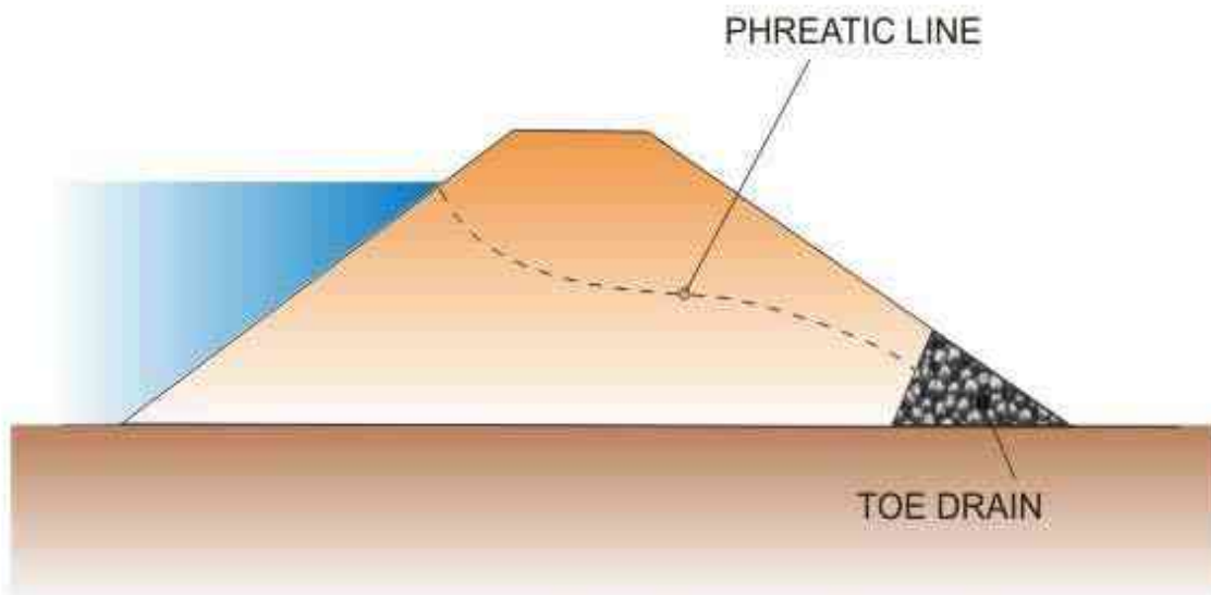
FIGURE 2. Homogeneous earthen embankment dam with toe drain
