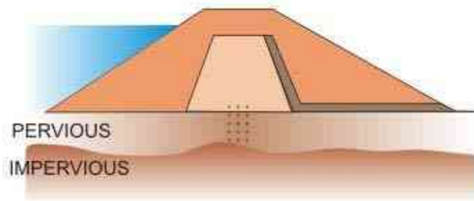
FIGURE 47. Grout curtain
