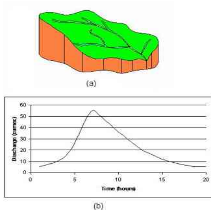
Figure 1. (a) Pear shaped catchment with narrow end towards upstream and blunt end towards outlet (b) Corresponding hydrograph for a hypothetical rainfall
