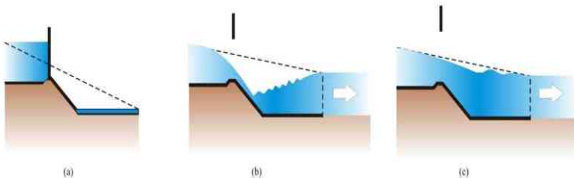
FIGURE 2. Seepage line gradient changes (a) steepest during no flow ; (b) Average during medium flood ; and (c) Almost none during high floods.
