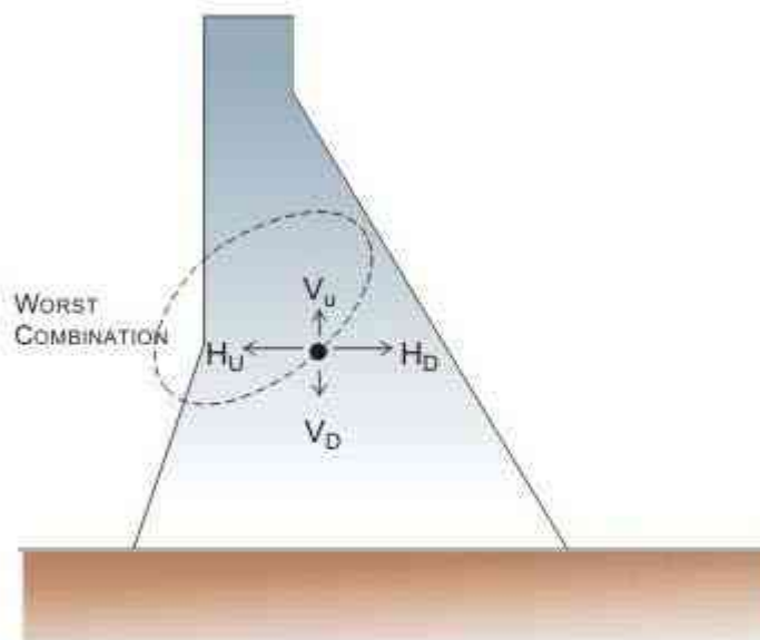
FIGURE 30. Worst combination of earthquake forces under reservoir empty condition
