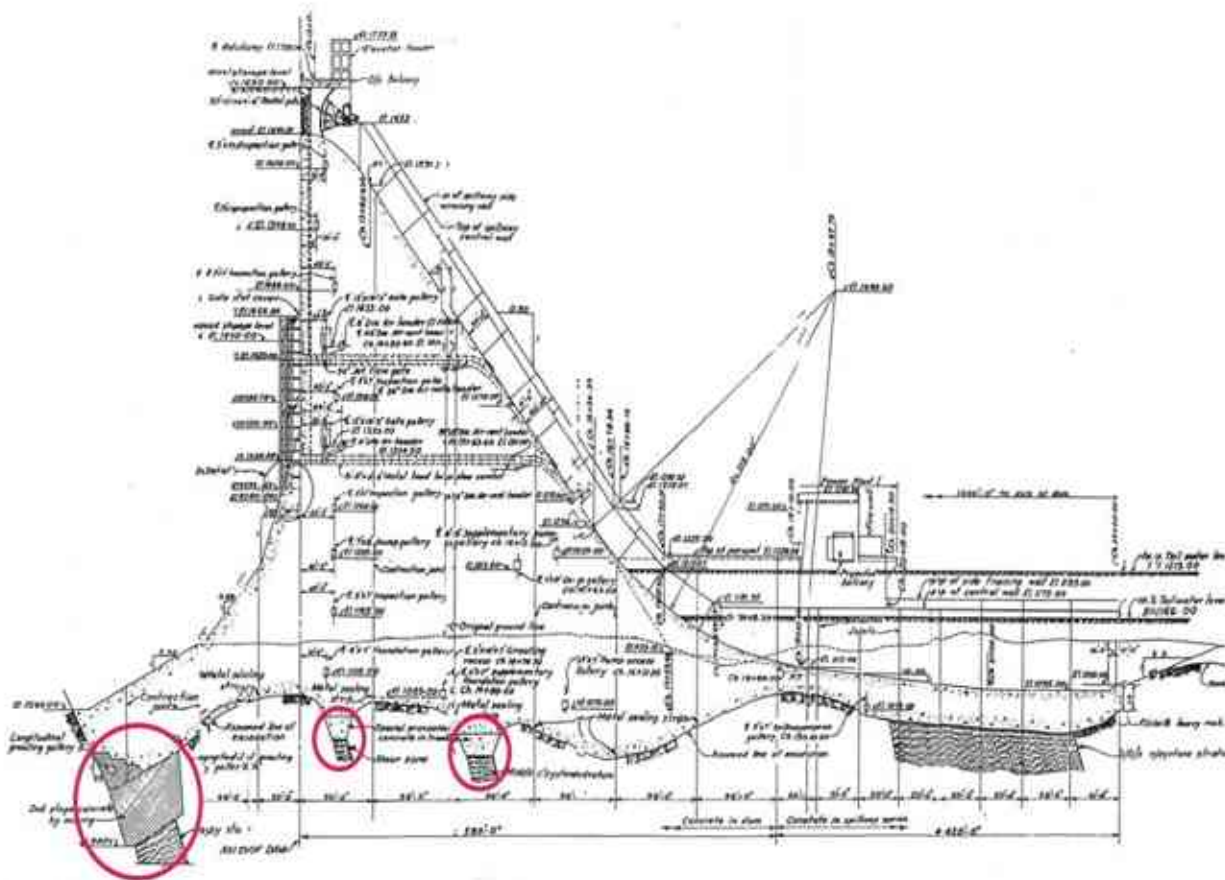
FIGURE 42. FOUNDATION FEATURE FOR BHAKRA DAM
