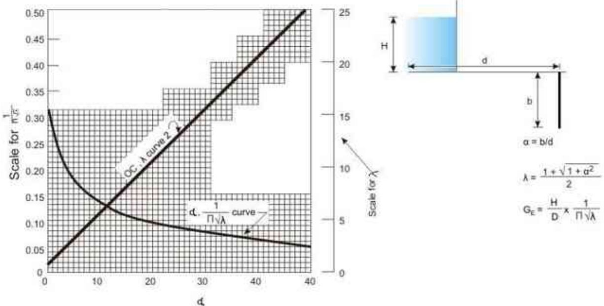
FIGURE 11. Curves for estimating Exit Gradient.
