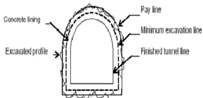
TYPICAL CROSS SECTION OF TUNNEL 4.50 m dia.
