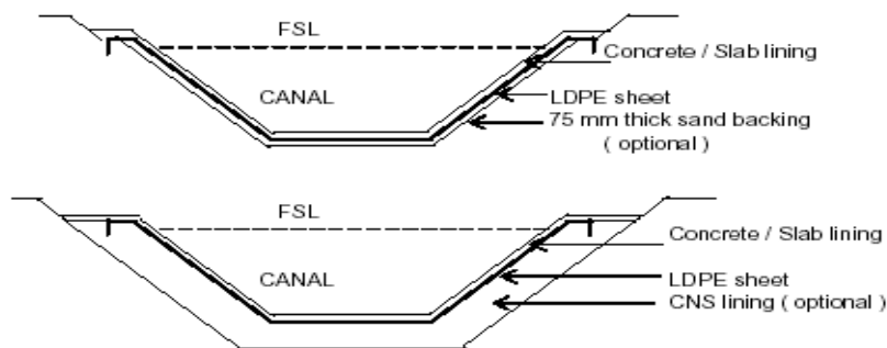
TYPICAL SKETCH SHOWING LDPE SHEET FOR CANAL LINING
