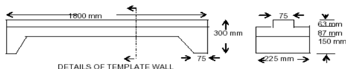
DETAILS OF TEMPLATE WALL
