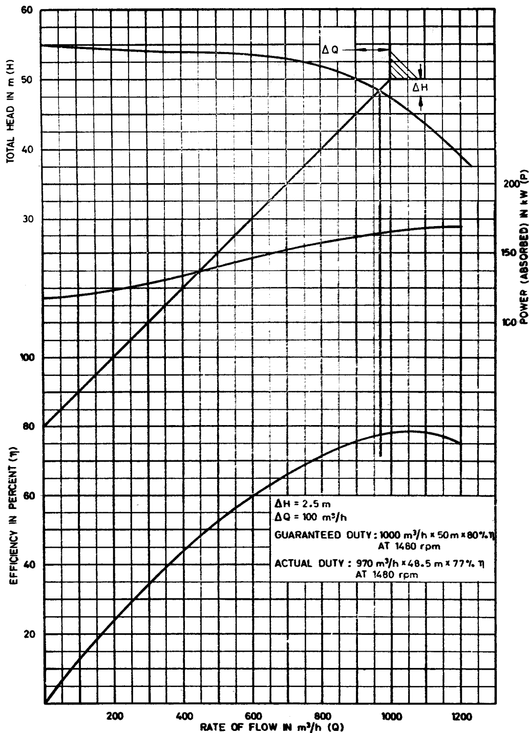
FIG. 10A CHARACTERISTIC CURVE FOR PUMP OF GUARANTEED DUTY OF 1 000 m³/h DISCHARGE × 50 m HEAD
