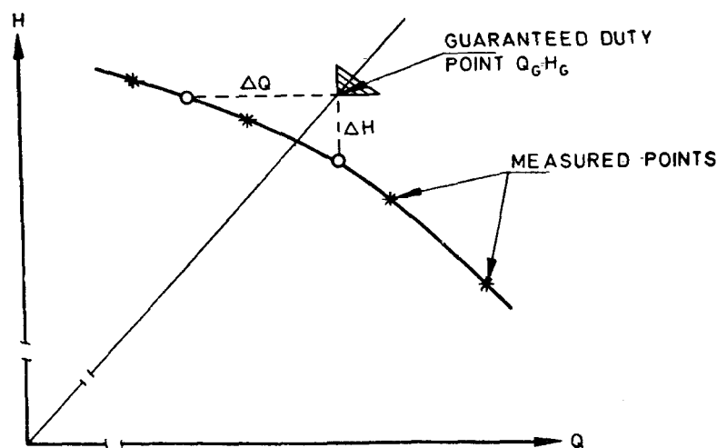
FIG. 10 CURVE QH FOR THE VERIFICATION OF THE GUARANTEE
