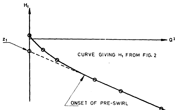
FIG. 12 CORRECTION OF MEASURED INLET HEAD
