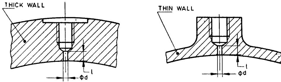
FIG. 1 REQUIREMENTS FOR STATIC HEAD TAPPINGS
