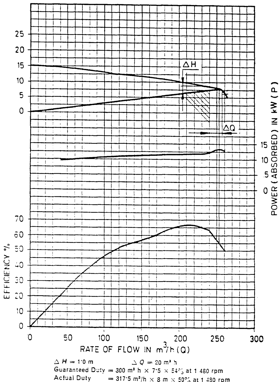
FIG. 10D CHARACTERISTIC CURVE FOR PUMP OF GUARANTEED DUTY OF 300 \text{ m}^3/\text{h} DISCHARGE \times 7.5 \text{ m} HEAD
