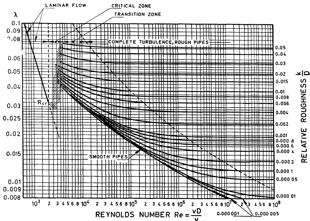
FIG. 15 VALUES OF FRICTION FACTOR \lambda MOODY CHART
