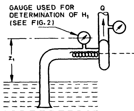
FIG. 11 EXAMPLE OF INSTALLATION WITH PRE-SWIRL
