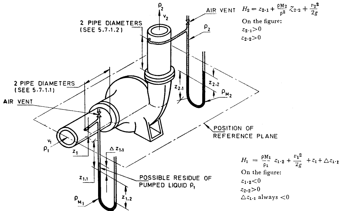
FIG. 1 REQUIREMENTS FOR STATIC HEAD TAPPINGS
