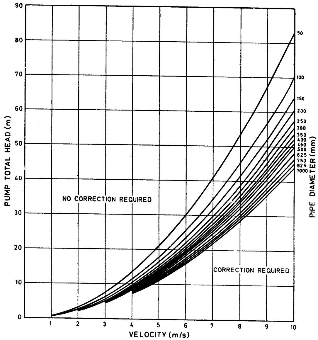
FIG 13 CHART SHOWING VELOCITIES ABOVE WHICH LOSS CORRECTIONS ARE REQUIRED
