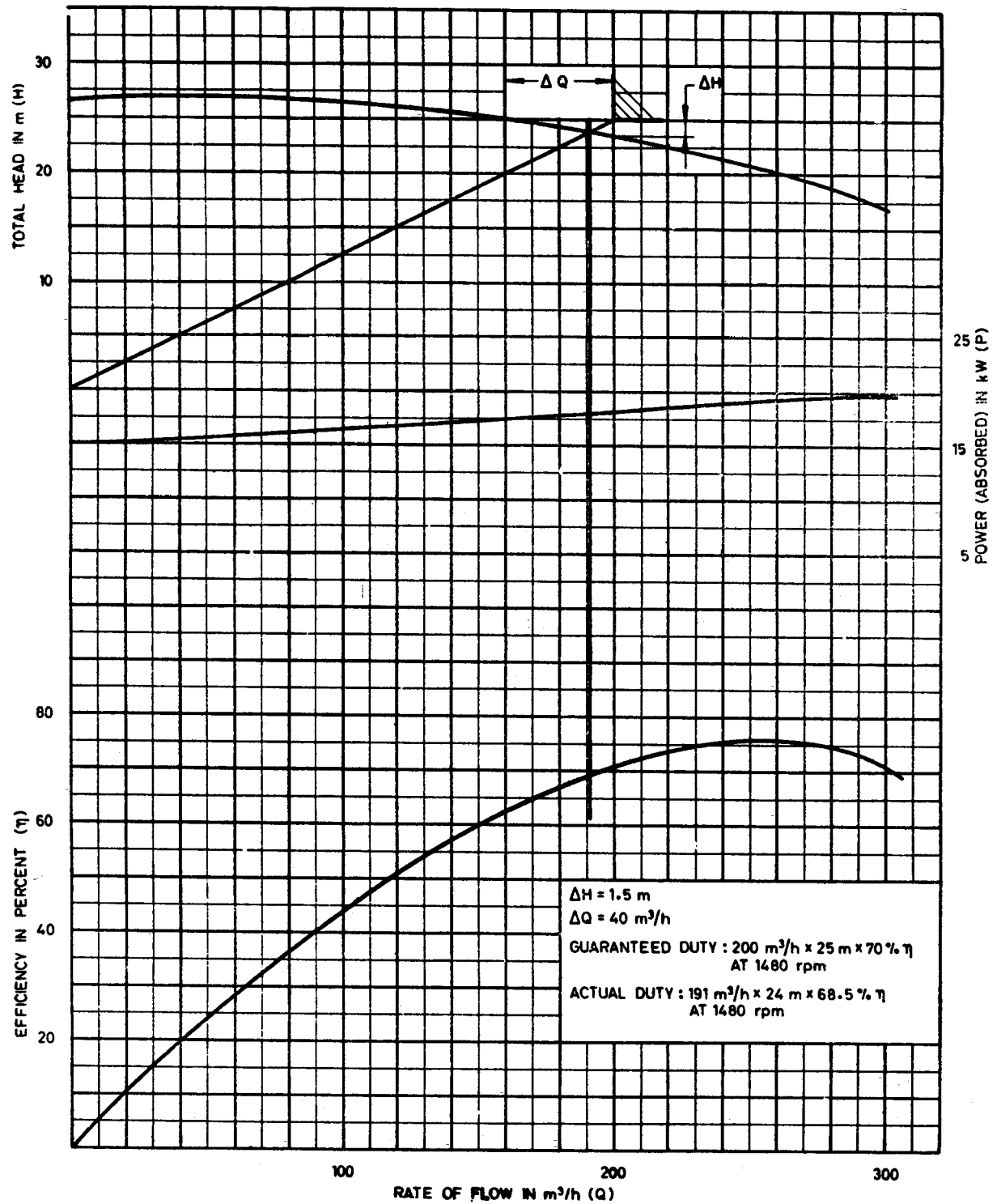
FIG. 10B CHARACTERISTIC CURVE FOR PUMP OF GUARANTEED DUTY OF 200 \text{ m}^3/\text{h} DISCHARGE \times 25 m HEAD
