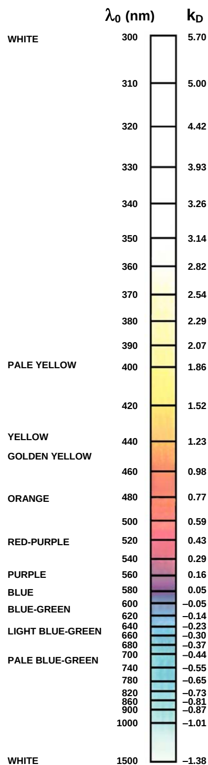
Figure 1. CSDS (central stop dispersion staining color) vs. corresponding matching wavelength \lambda_0 (in nm) and Su's conversion factor K_D (Su, 1993). (Modified from the Dispersion Staining Color Chart, McCrone, 1967)
