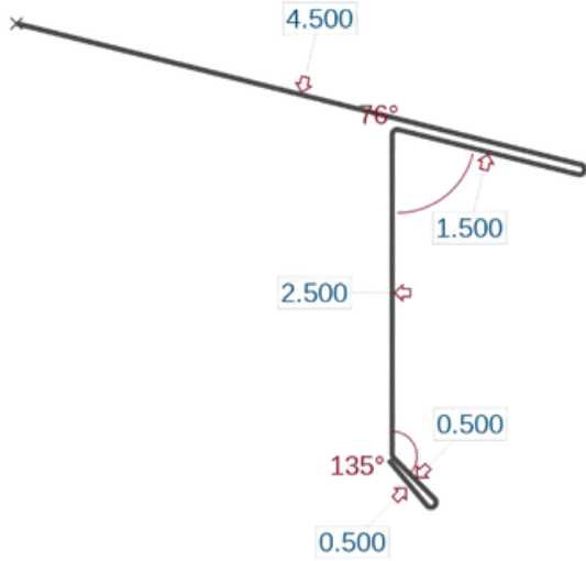
Residential Drip Edge D Style (RDE)
