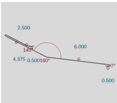
1.75 Inside Corner (IC1)
