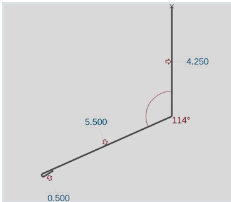
7.2 Snow Stop (ST72)
