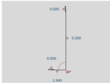
Commercial Inside Corner (CIC1)
