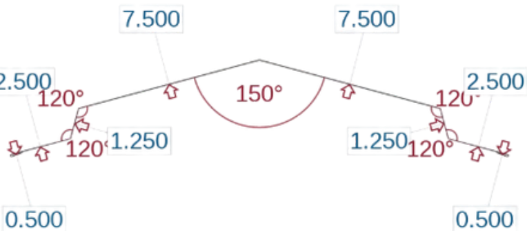
RidgeCap Floating 7.5" (SSRCP7)
