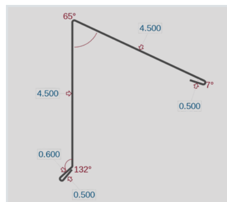
1.75 Outside Corner (OC1)
