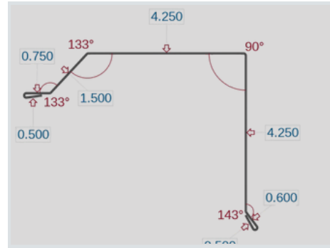
Commercial Slope Transition (CST)
