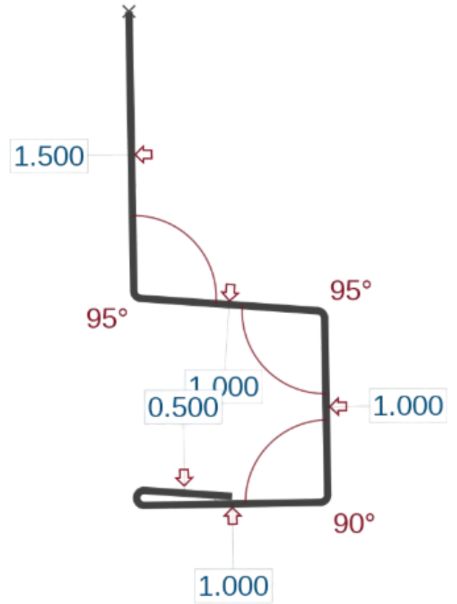
Square Base (SBA)
