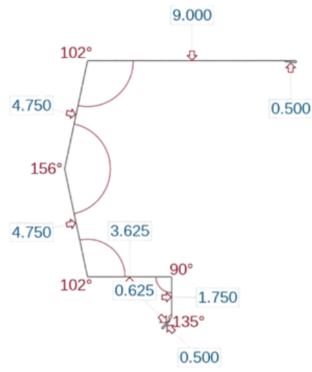
Sculptured High Side Eave > 2:12 (SSHI>)
