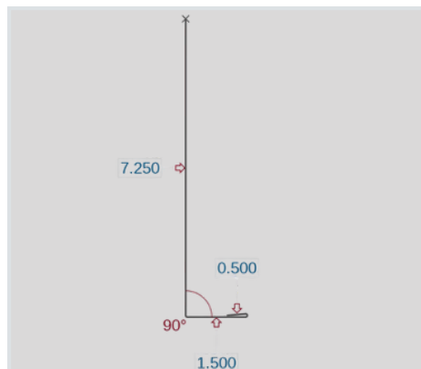
7.2 Inside Corner (IC72)
