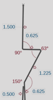
Soffit Rat Guard (SFRG)
