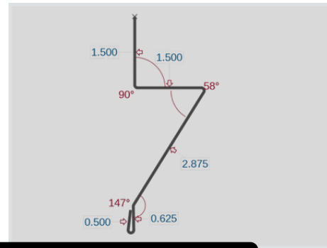
Commercial Downspout (CDS)
