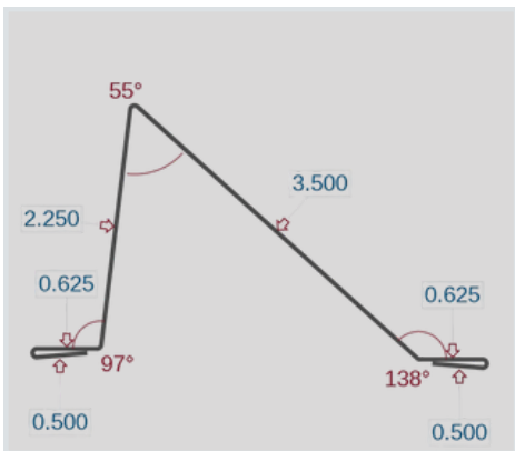
SB Outside Corner (SBOC)
