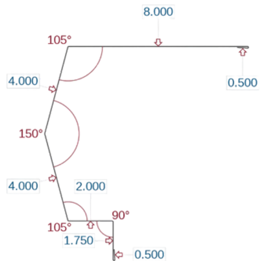
Sculptured High Side Eave (HI)
