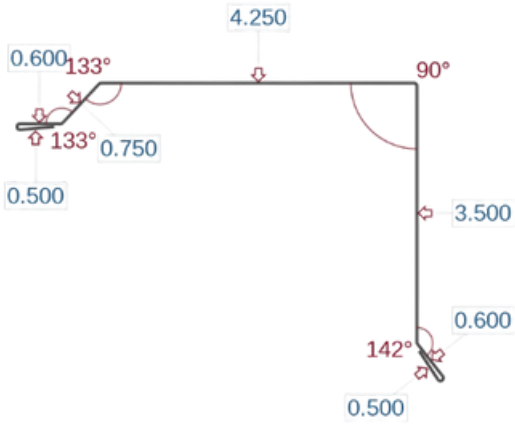
Residential Rake Trim (RRT)
