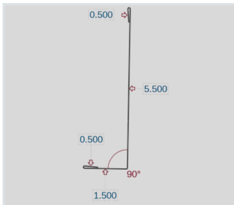
SB Inside Corner (SBIC)
