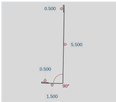
Inside Corner (IC1)
