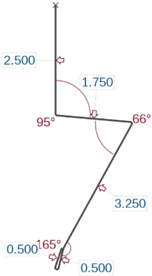
1 3/4" Commercial Ratguard (RGC)
