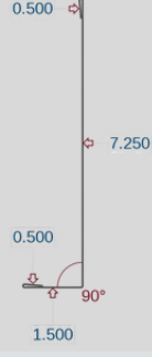
Soffit Garage Door J (SFGDJ)
