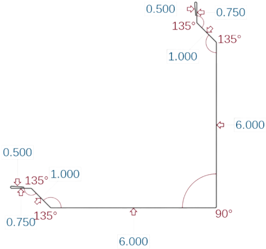
Corner Style Rake 6" Face (CSR)
