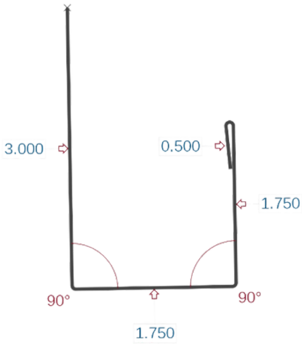
J - Channel 1 3/4" Receiver R-Loc Open
