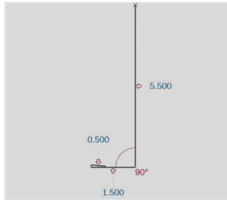
7.2 Outside Corner (OC72)
