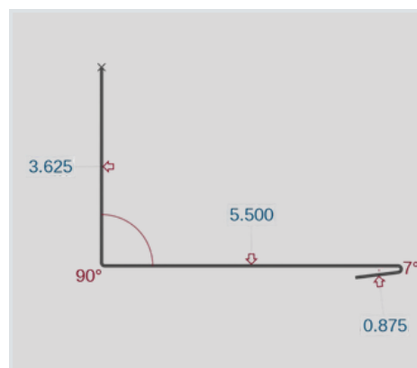
1.75 Drip Cap (DC1)
