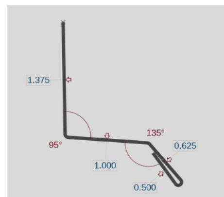
Angle Base (AB)
