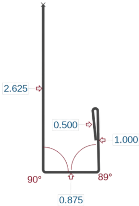
J - Channel (JT)
