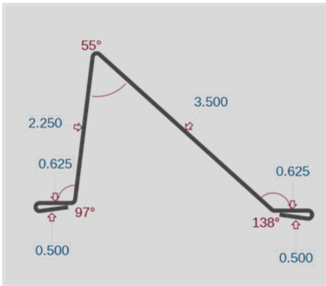
7.2 Drip Cap (DC72)
