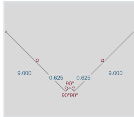
SB Window Drip Cap (SBWDC)
