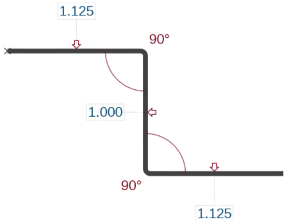
ZEE Closures (HLZC)
