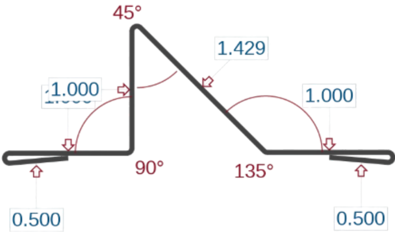
Exposed Fastener Snow Guard 1"
