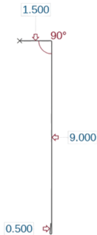
9" Door Post Trim (DJ9)
