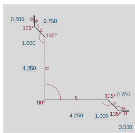
Wainscot (WC)
