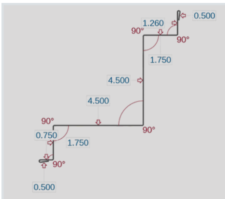
1.75 Rat Guard (RG1)
