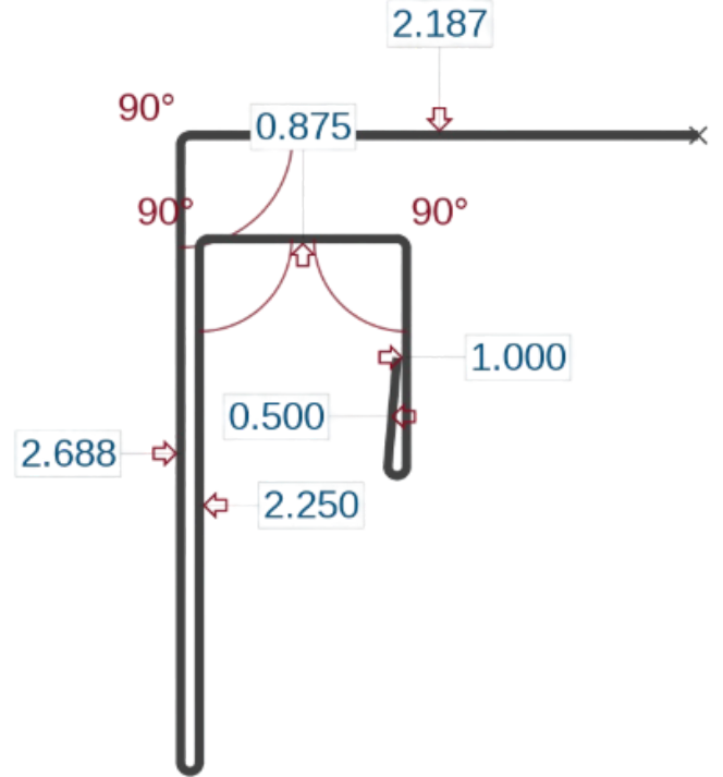
Soffit F and J channel (SFJ)
