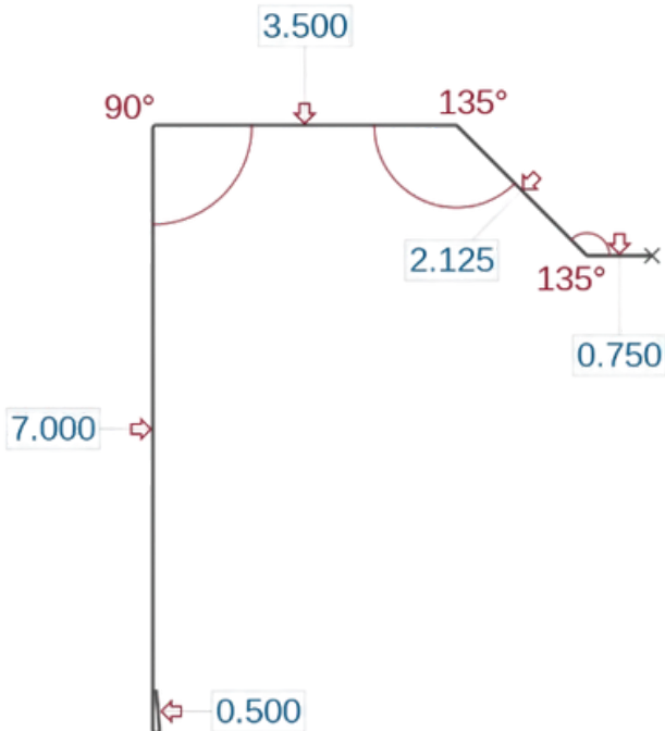
Track Door Jamb (TDJT)
