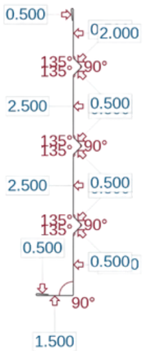
Fascia 11 1/2" Ribbed (FR)
