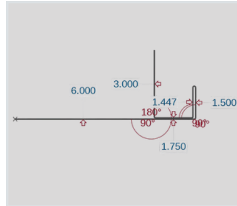
7.2 Rat Gaurd (RG72)
