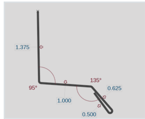
BB Angle Base (BBAB)
