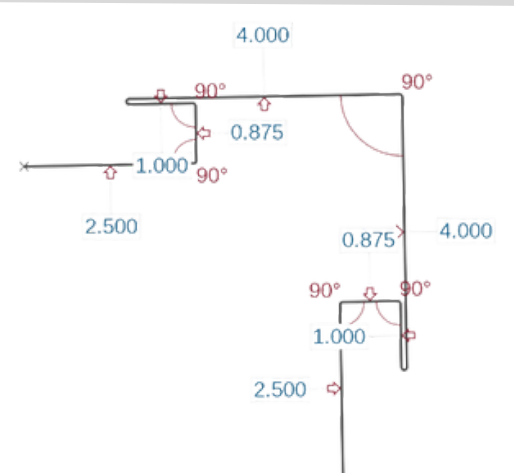
Outside Corner with 1" Receiver (OC1R)
