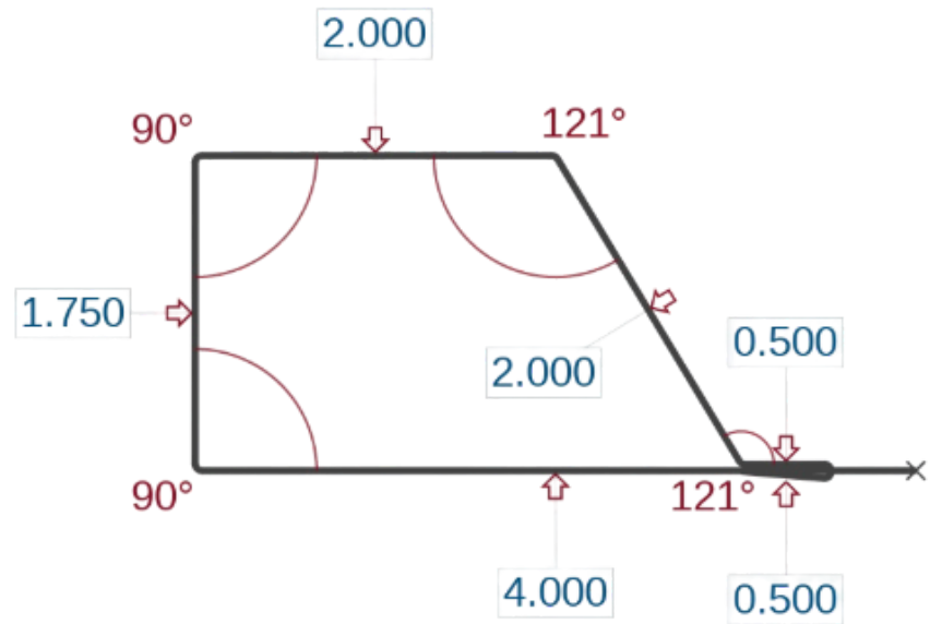
J-Channel R-Loc Closed
