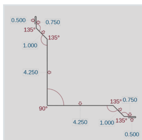
Wainscot (WC)
