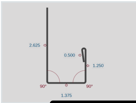
Commercial Gable (CG)
