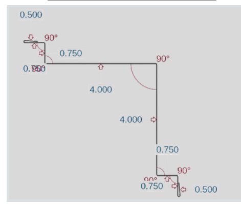
BB Window Drip Cap (BBWDC)
