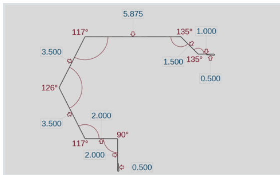
Commercial Gable (CG)
