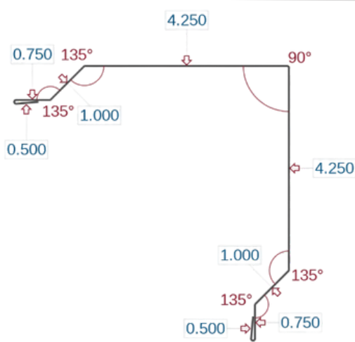
Outside Corner (COR)
