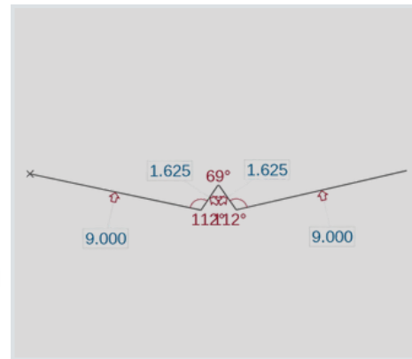
7.2 FJ Channel (FJC72)
