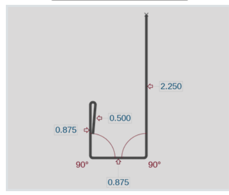
BB Angle Base (BBAB)
