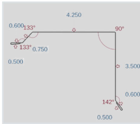
Sloped Transition (ST)
