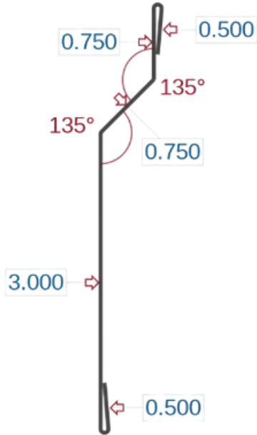
Counter Flashing (CF)
