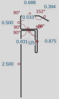
Soffit Outside Corner (SFOC)
