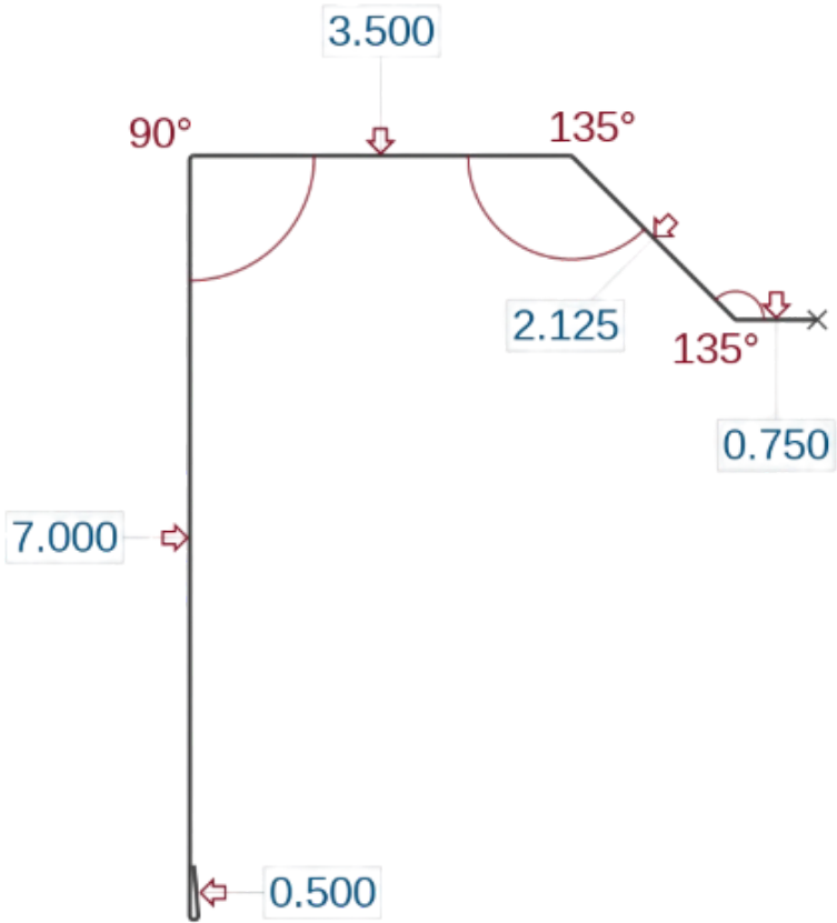
Track Door Jamb (TDJT)
