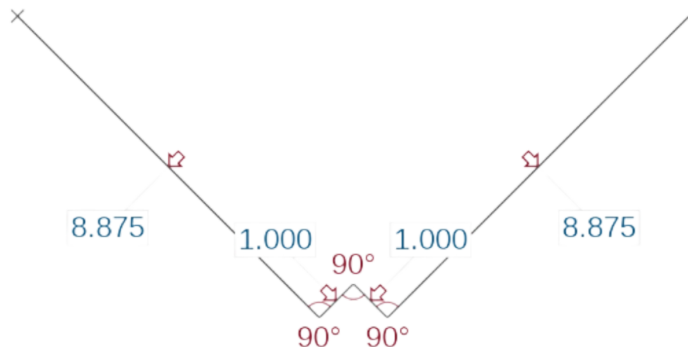
Valley Trim NO HEM (VT)
