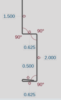
Soffit J Channel (SFJC)
