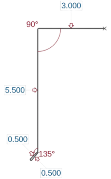
Long Eave (LEA)
