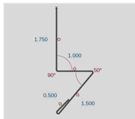
Rat Guard (RG)
