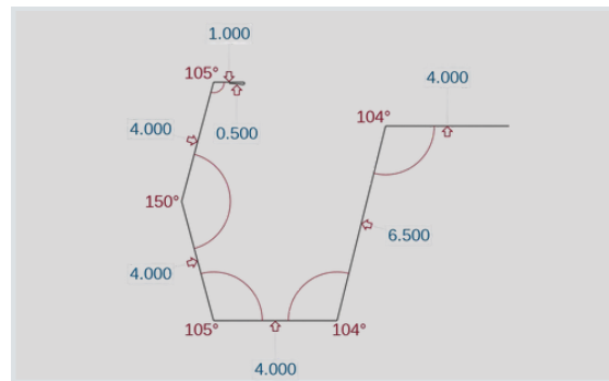
Sculptured Gutters (SHOG...)
