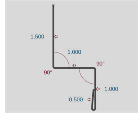
BB Wainscot (BBWC)
