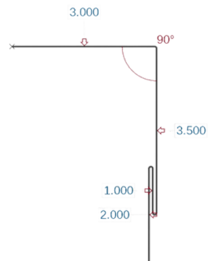
Style L Eave With Receiver Channel
