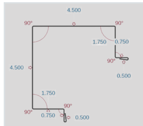
1.75 Angle Base (AB1)
