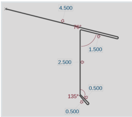
1.75 8"x8" Flat Ridge Cap (FRC1)
