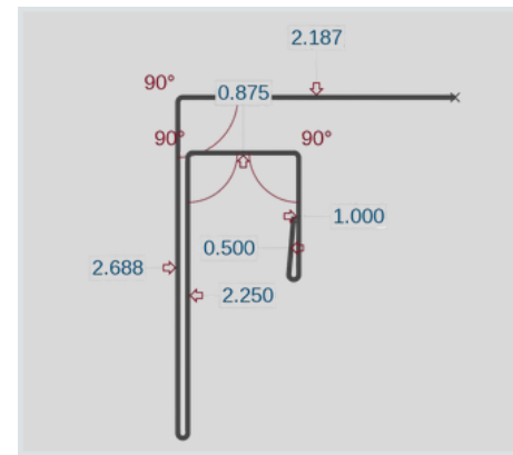
Garage Door J (GDJ)
