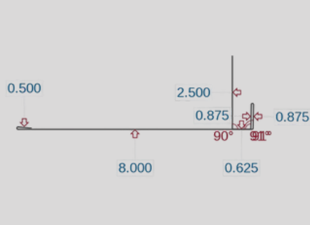
Soffit Rat Guard (SFRG)
