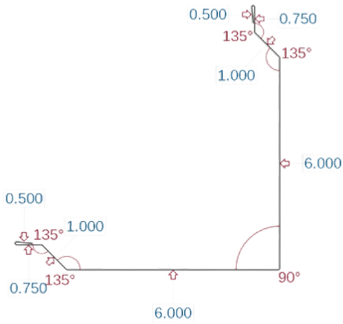
Corner Style Rake 6" Face (CSR)
