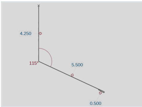
Commercial Snow Guards (CSG)
