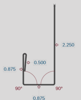
Soffit Wainscot (SFWC)
