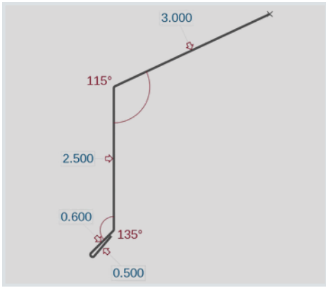
SB Endwall (SBEW)
