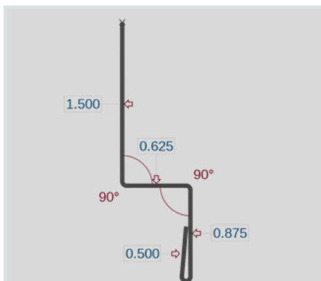
SB Wainscot (SBWC)
