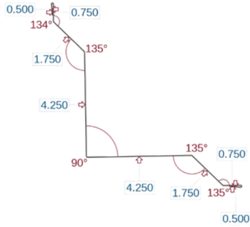
Commercial Inside Corner (CIN)
