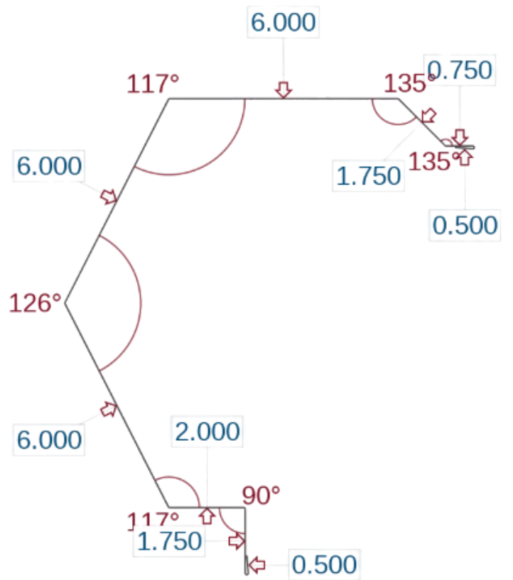
Sculptured Gable Flashing
