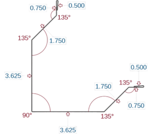
Commercial Outside Corner (COU)
