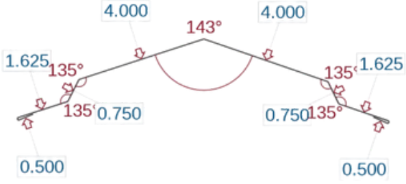
Step Up Ridge Cap (RCP)
