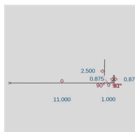
Angle Base (AB)
