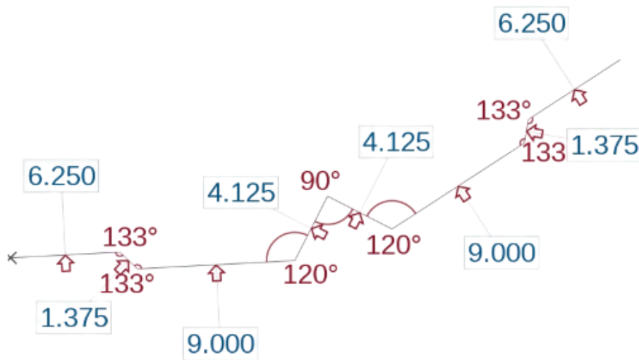
High Valley (HVAL)
