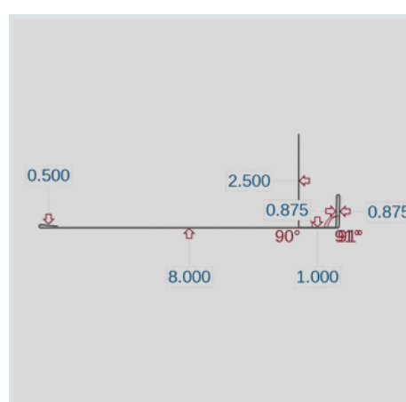
SB Garage Door J (SBGDJ)
