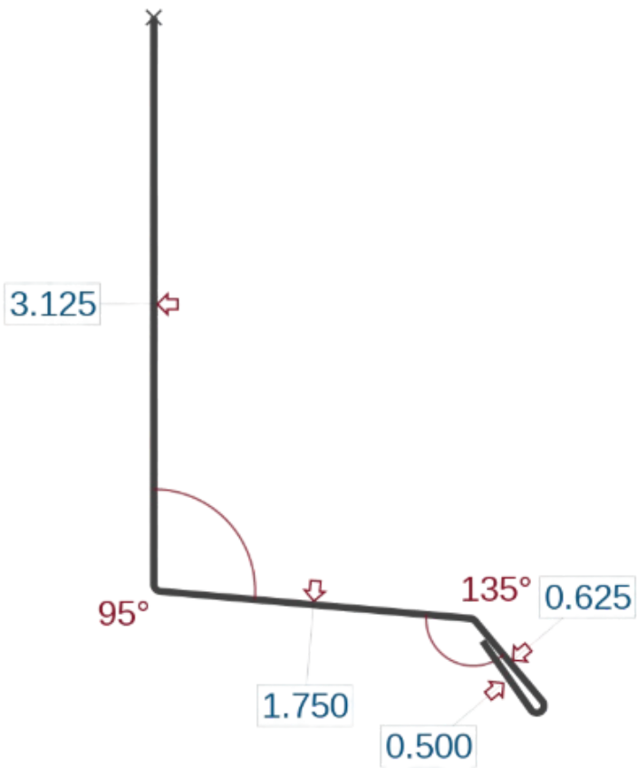
Base Trim (BA)
