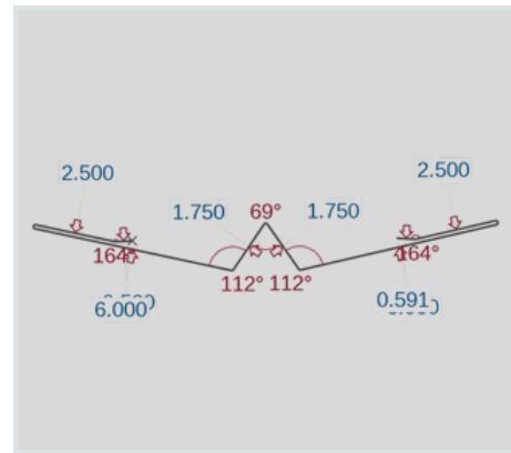
1.75 High Side Peak Trim (HPT1)
