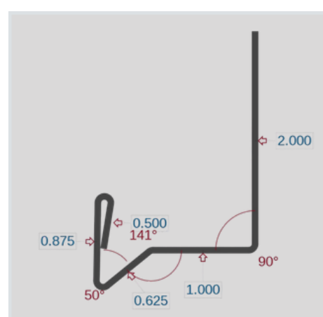
Rat Guard (RG)
