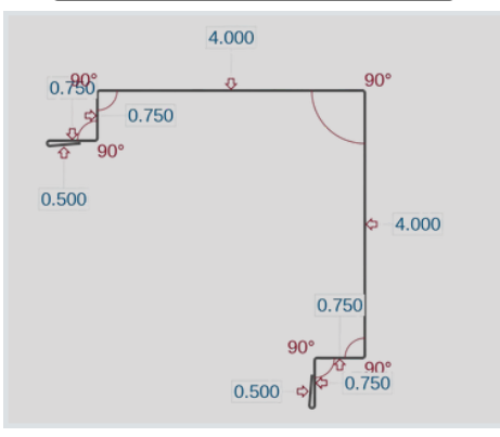
BB Garage Door J (BBGDJ)
