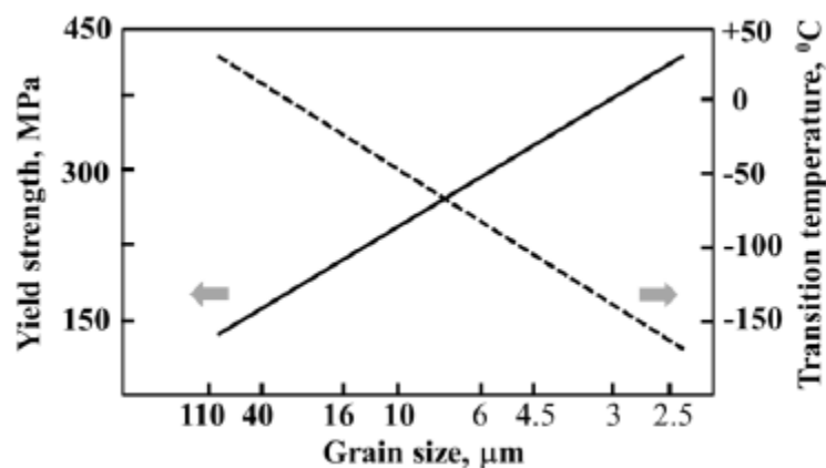
Figure 5. Ferrite grain size relationship to yield strength and Ductile to Brittle Transition Temperature
