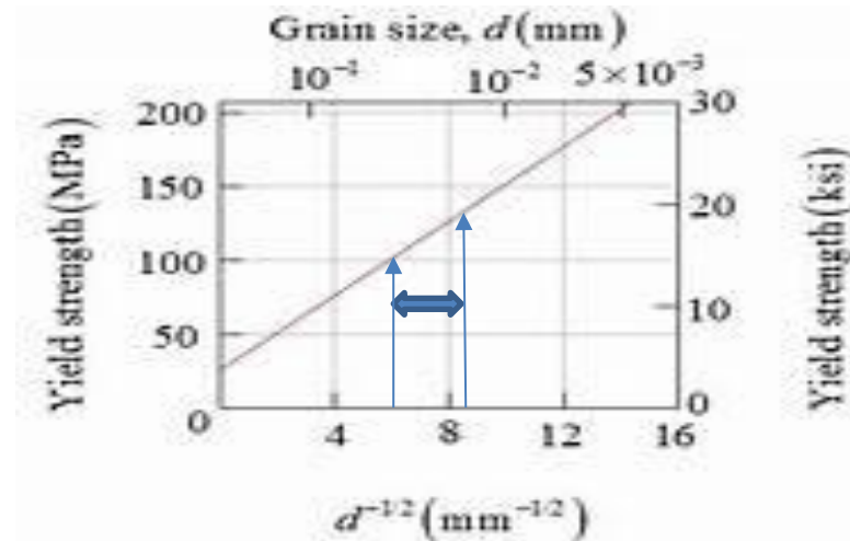
Figure 7. Grain size effect on yield strength [13]
