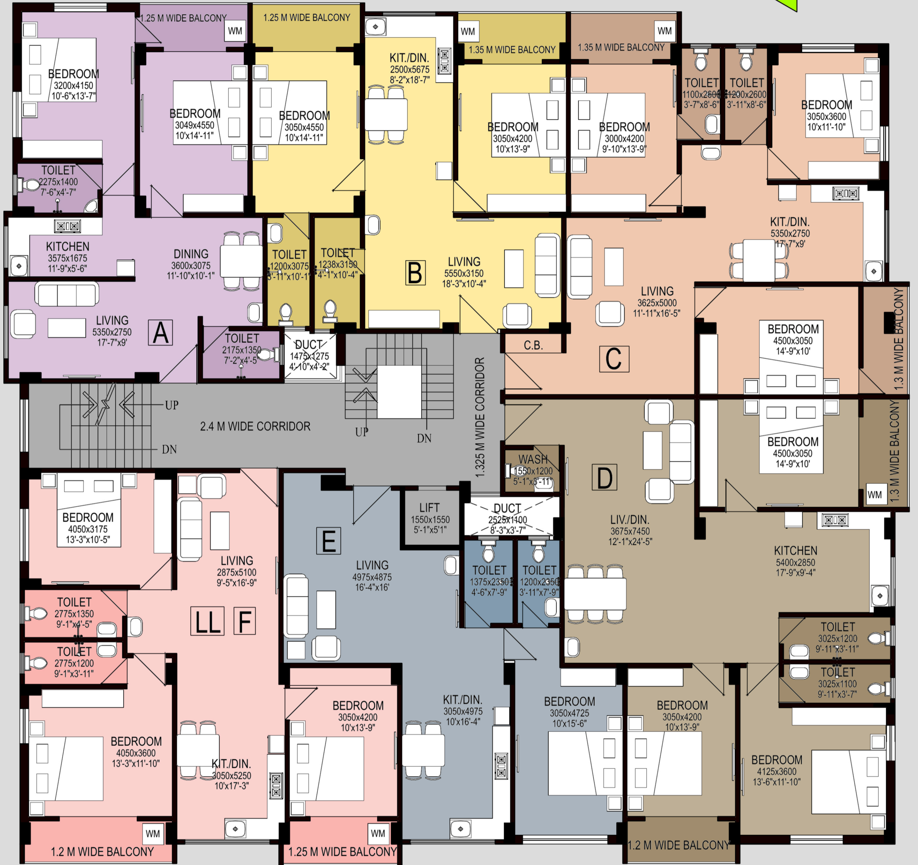
4TH FLOOR PLAN
