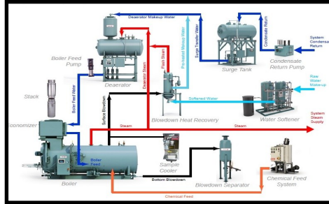
Steam Utilities
