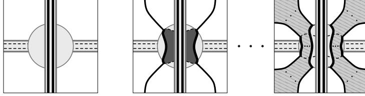
Figure 8: An arbitrary crossing ball: (left) disjoint from F , (center) intersecting F in a single component, (right) intersecting F in at least two components (c.f. Lemma 4.1.3).
