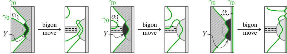
Figure 12: Every innermost circle \gamma_0 \subset F \cap S^\pm is disjoint from \partial C (c.f. Proposition 4.2.2).
