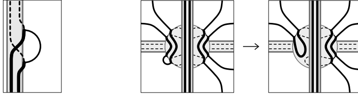
Figure 9: No arc of F \cap S^+ \cap S^- is parallel in S^+ \cap S^- to \partial\nu L (left) or to \partial C (right).
