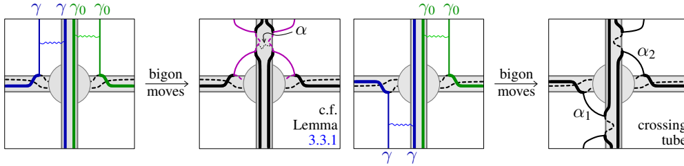
Figure 13: If both circles \gamma, \gamma_0 of F \cap S^\pm traversing a given over/underpass, say at C_t , have height zero, then F can be isotoped to have a standard tube near C_t .
