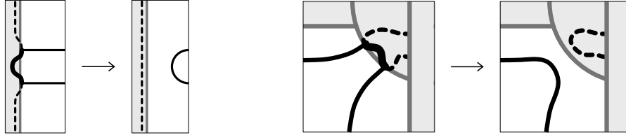
Figure 7: No arc of F \cap \partial\nu L \cap S^\pm is parallel in \partial\nu L to S^+ \cap S^- (left), and no arc of F \cap \partial C \cap S^\pm is parallel in \partial C to S^+ \cap S^- (right).
