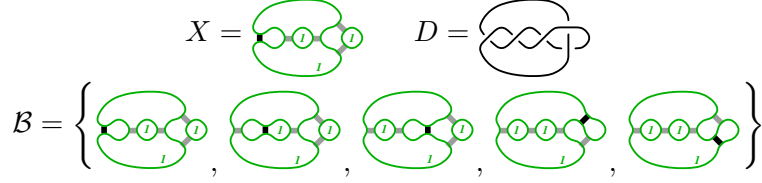
FIGURE 10. Over \mathbb{F}_2 , this enhancement X of an inessential state x of D represents a nonzero homology class, since dX = 0 and \varepsilon \circ \pi_{\mathcal{B}} \circ d \equiv 0 , where \mathcal{B} is an \mathbb{F}_2 -basis for \mathcal{C}_{\mathbb{F}_2}^{i_x, j_X}(D) .
