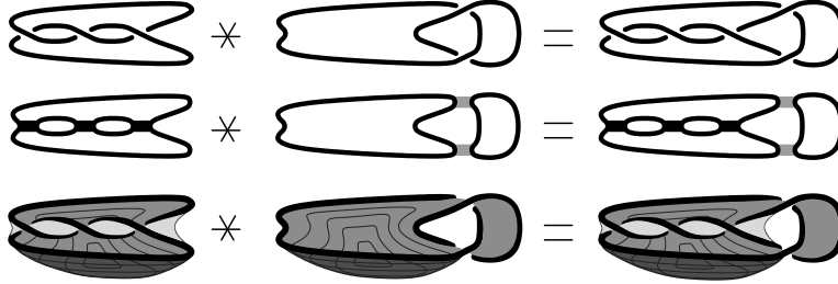
FIGURE 6. Plumbings of link diagrams, states, and surfaces.
