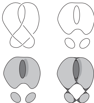
FIGURE 8. Constructing a state surface.
