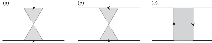
FIGURE 32. (a) and (b): Up to symmetry, the two possibilities for the orientation on L near the removed crossing band. (c): In the case of (b), gluing an untwisted band extends the orientation on L^* to one on L .
