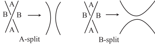
FIGURE 10. A and B splittings in the construction of a state surface.
