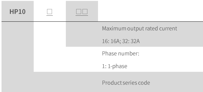
Fig. 4-3 Model number definition
