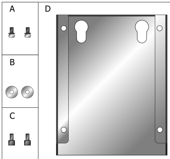
Fig. 5-1 Wall-mounting accessories
