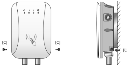
Fig. 5-8 Fixed the wallbox
