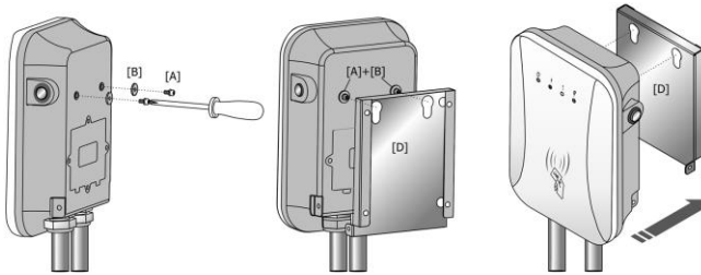
Fig. 5-7 Mounting the wallbox on the accessories-D
