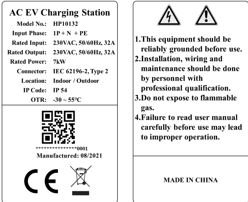
Fig. 4-4 The location and content of the nameplate
