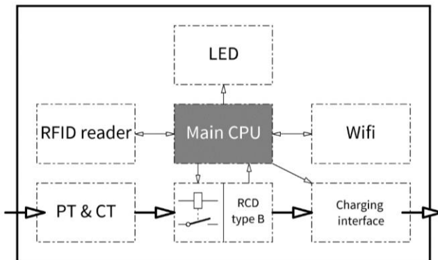
Fig. 4-2 Block diagram of products
