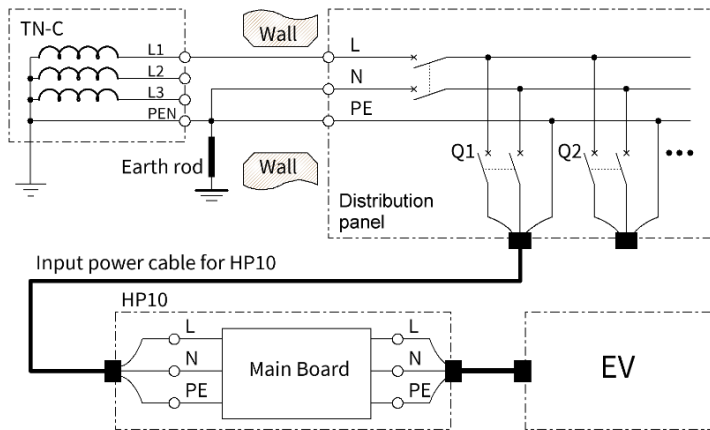
Fig. 5-4 HP10 work in TN-C system with earth rod
