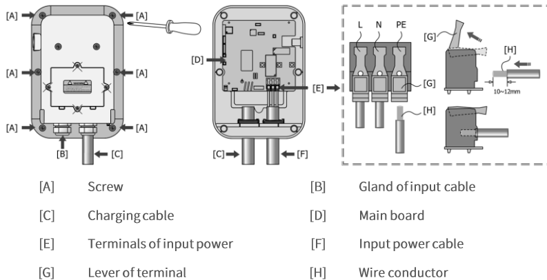
Fig. 5-6 Open the wallbox and wiring
