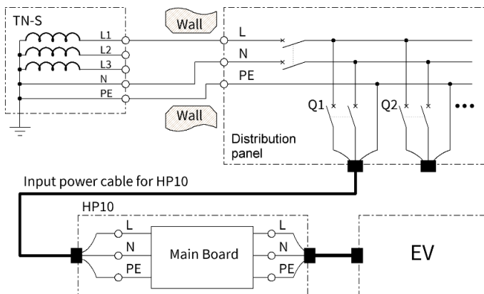
Fig. 5-3 HP10 work in TN-S system
