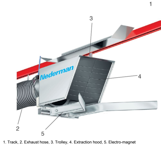
1. Track, 2. Exhaust hose, 3. Trolley, 4. Extraction hood, 5. Electro-magnet
