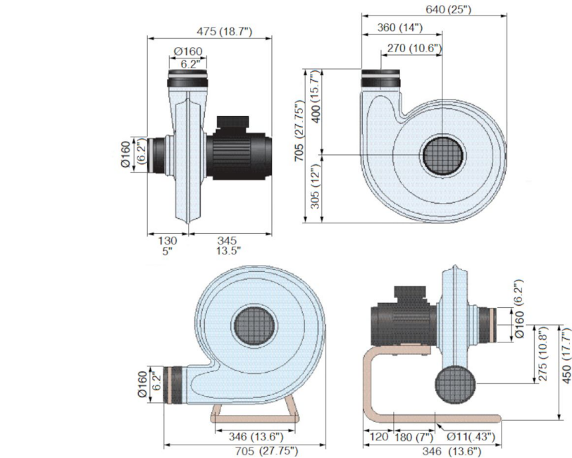
N29 fan, version with and without stand
