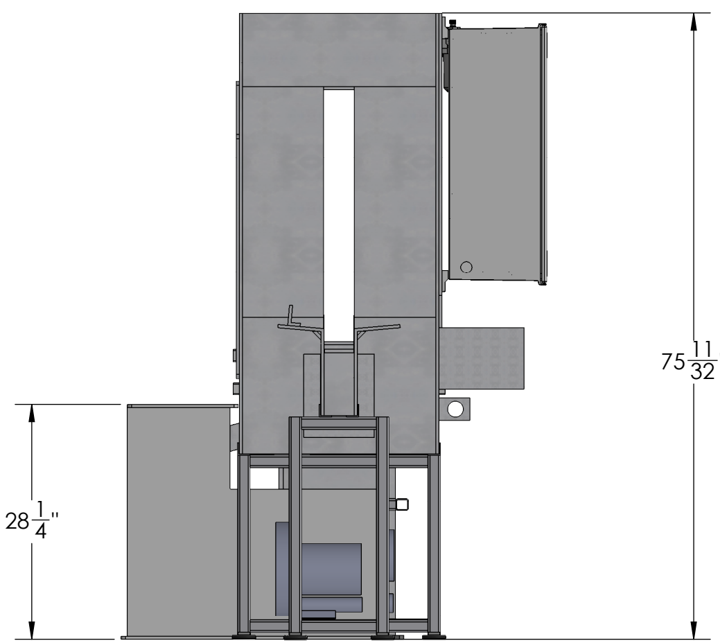
SIDE
