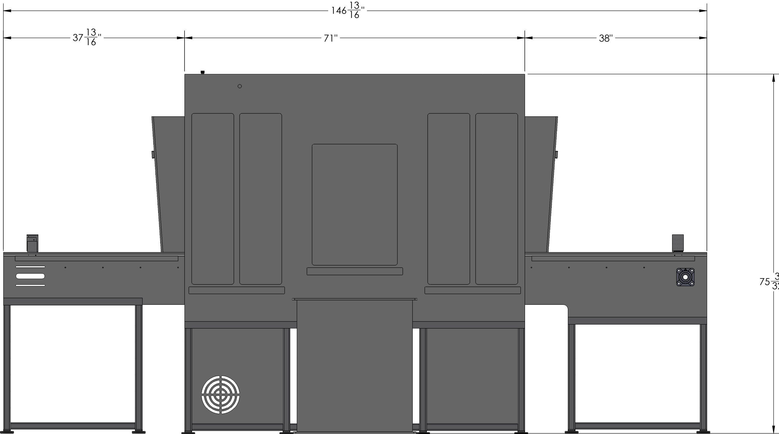
54" INFEED
