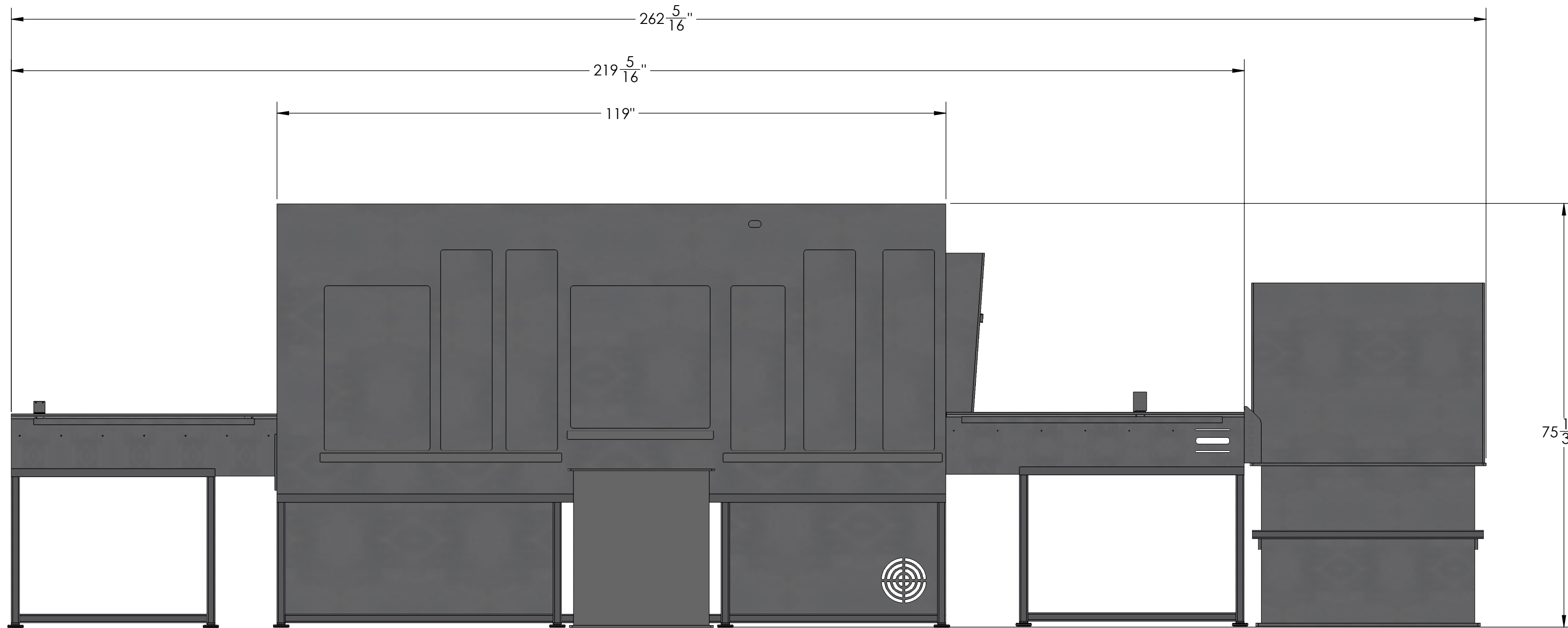
47" OUTFEED
