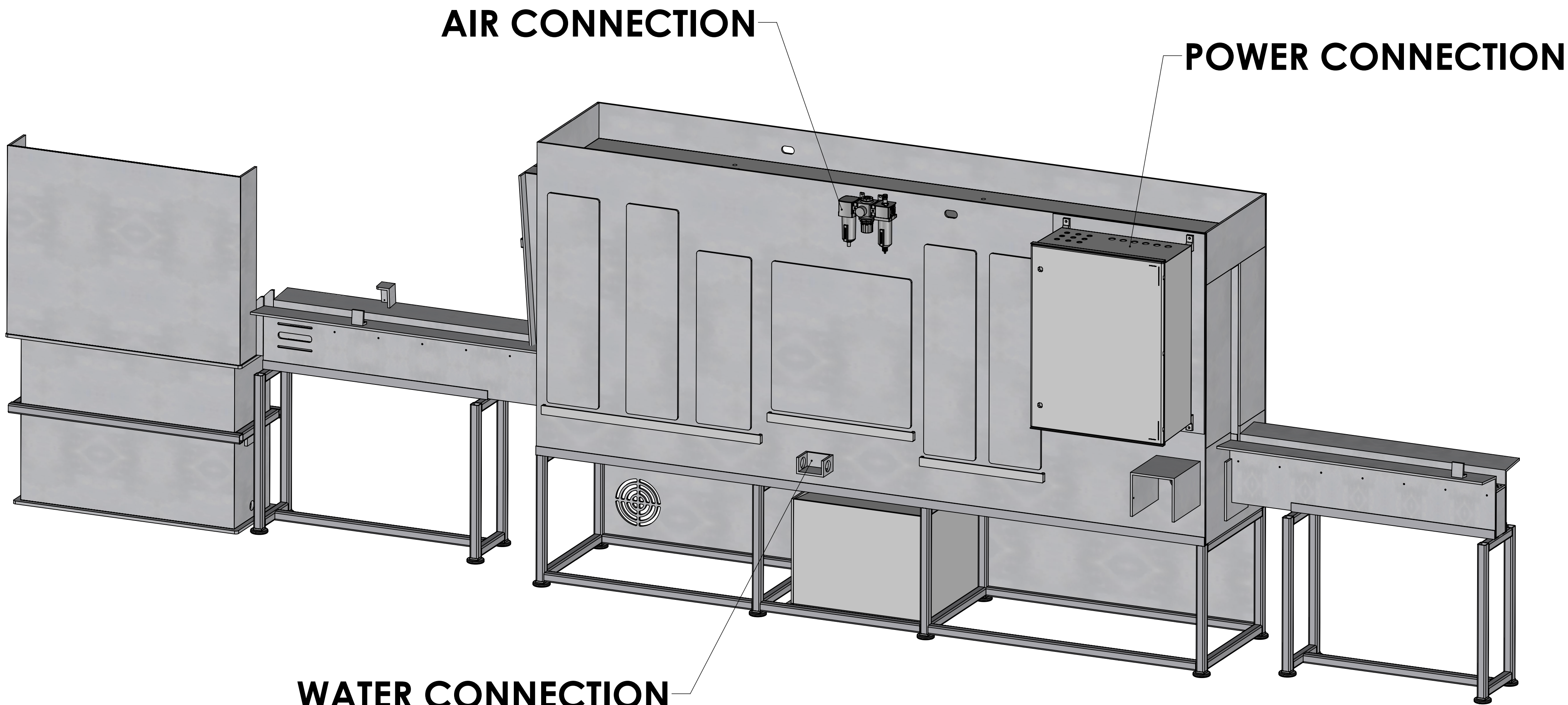
BACK ISO
