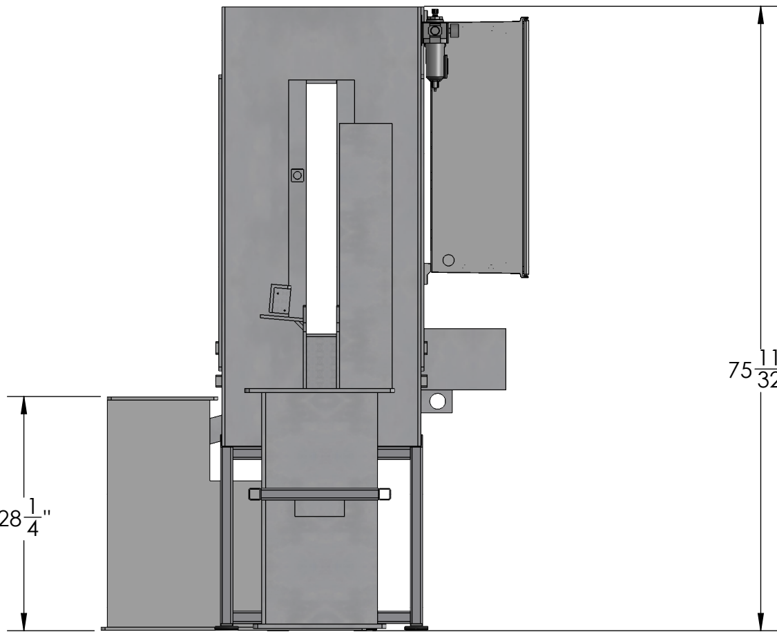
SIDE
