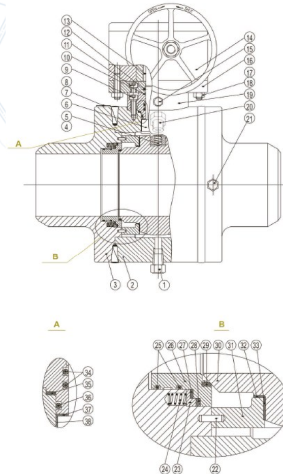
Full welded Trunnion Ball Valve
