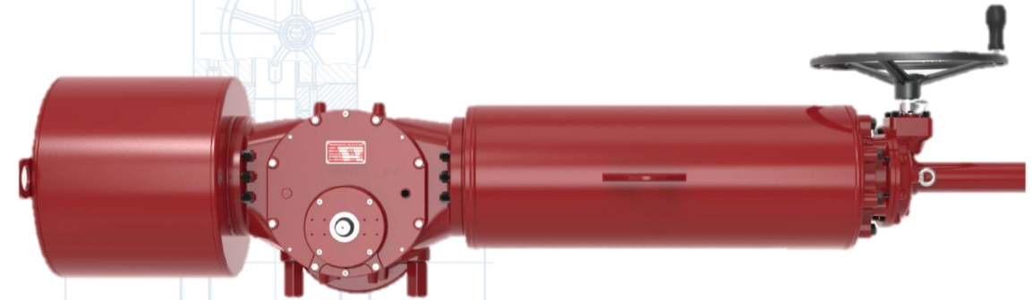
Single action Spring return, with handwheel
