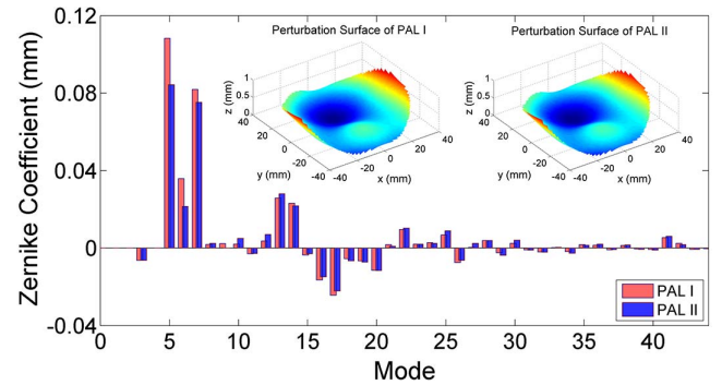
Fig. 2. Zernike coefficients of the PAL rear surface. The perturbation surfaces represent the deviation of the rear surface from a spherical background surface with a radius of curvature of 200 mm.
