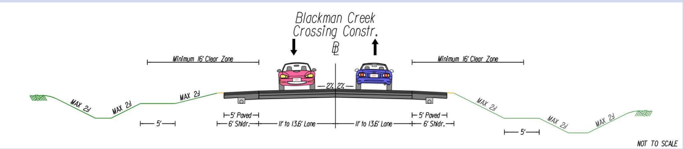
Blackman Creek Proposed Design: Typical Cross Section
