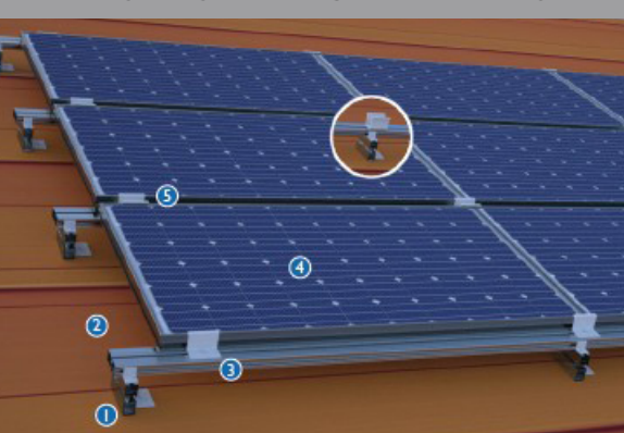
RACKING FRAMES AND RAILING
