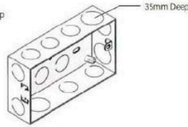
2 Gang Flush Box(63)
