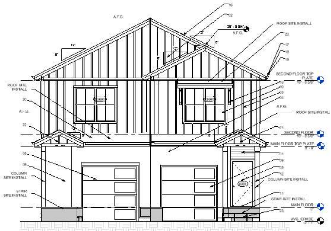
① FRONT ELEVATION ARCH 1/4" = 1'-0"
