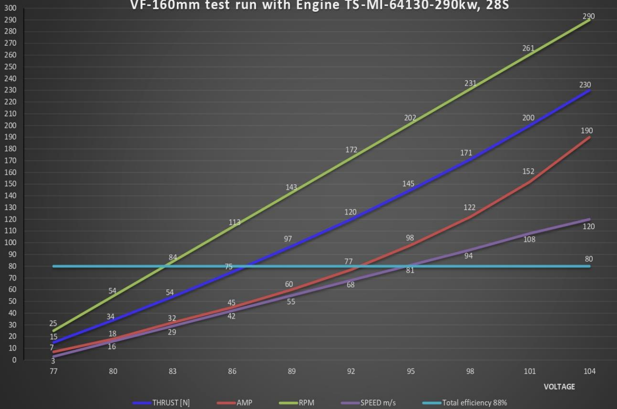
VF-160mm test run with Engine TS-MI-64130-290kw, 28S
