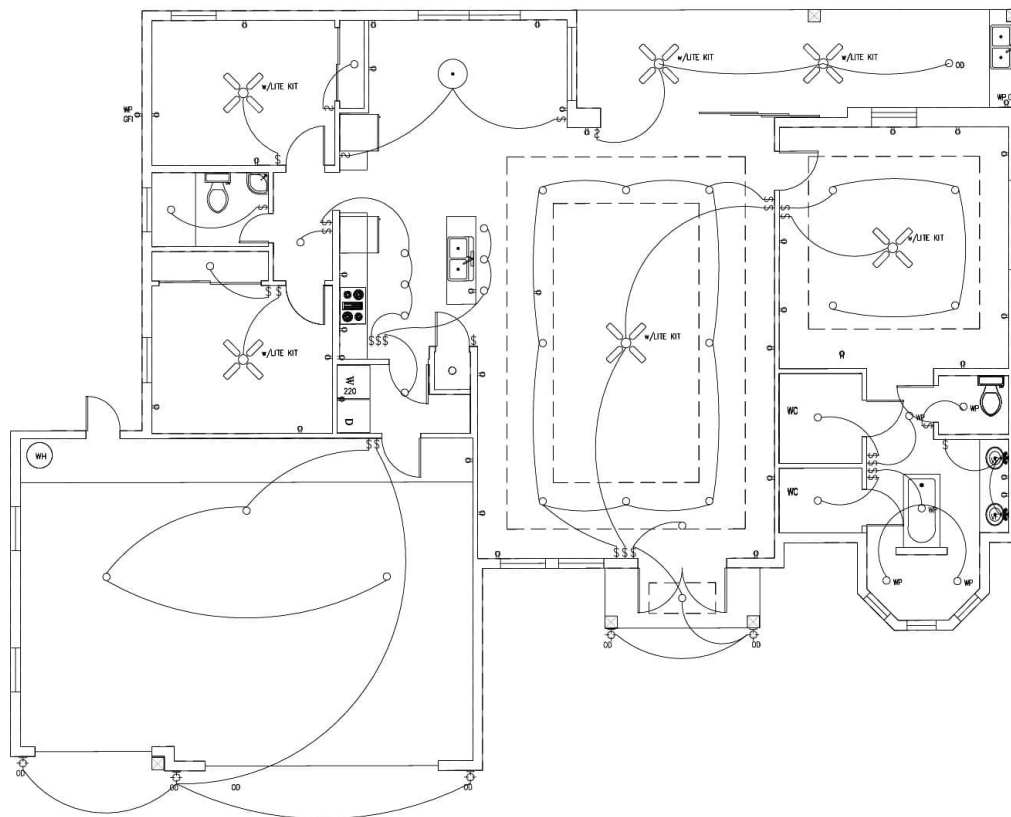
PROPOSED INTERIOR ELECTRICAL PLAN SCALE: 1/4" = 1'-0"
