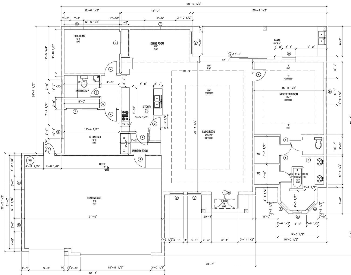
PROPOSED FLOOR PLAN SCALE: 1/4" = 1'-0"
