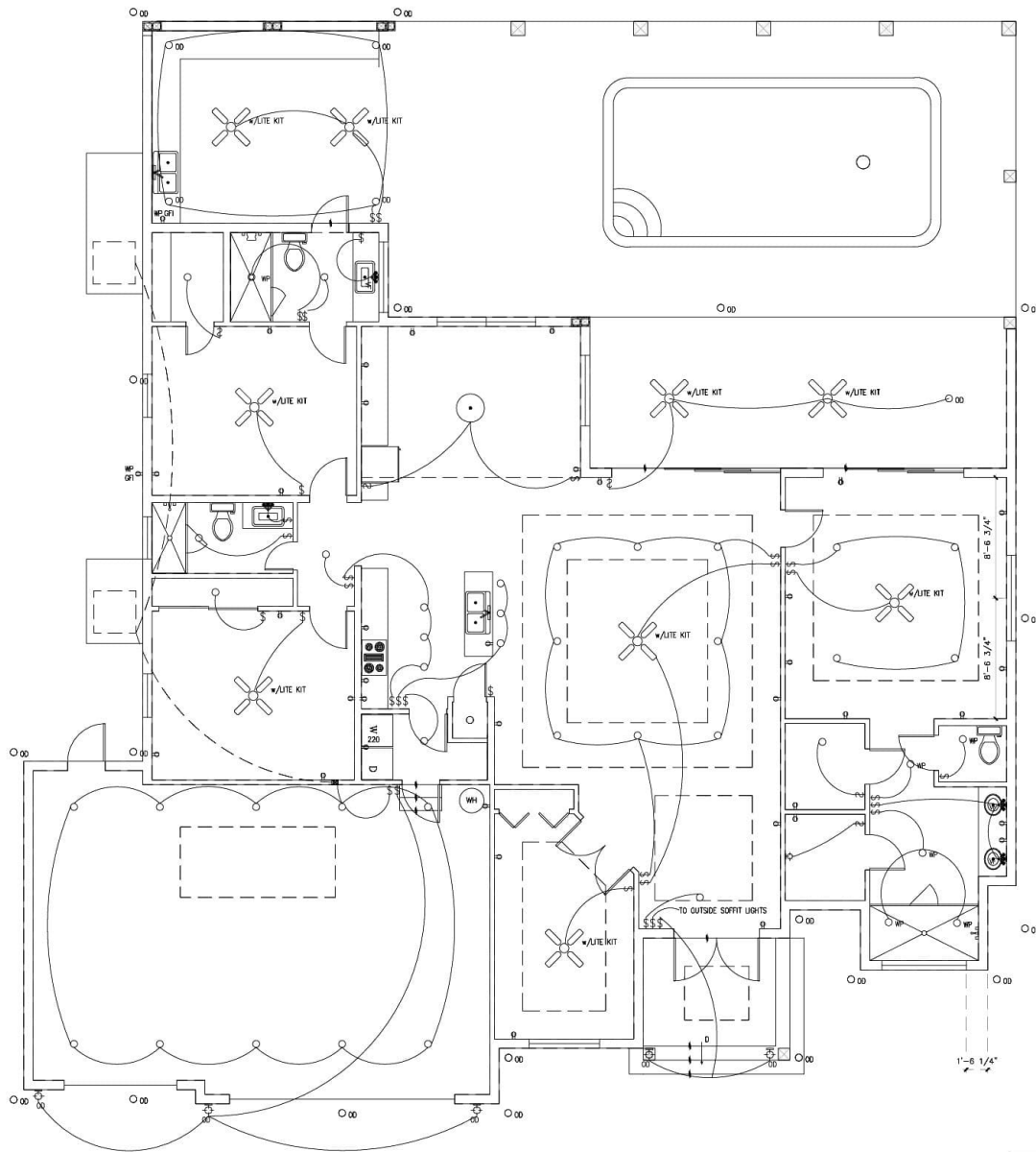
PROPOSED INTERIOR ELECTRICAL PLAN SCALE: 1/4" = 1'-0"
