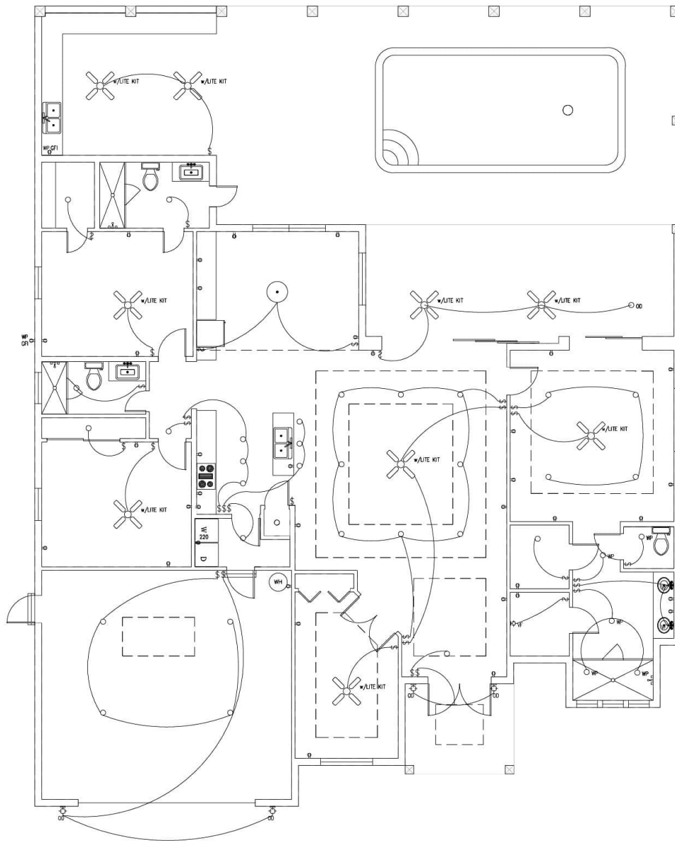
PROPOSED INTERIOR ELECTRICAL PLAN SCALE: 1/4" = 1'-0"
