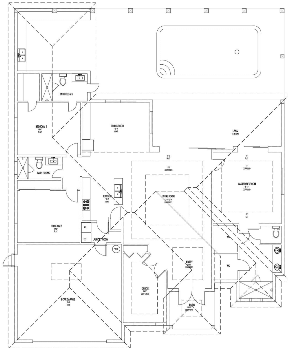
PROPOSED ROOF PLAN SCALE: 1/4" = 1'-0"
