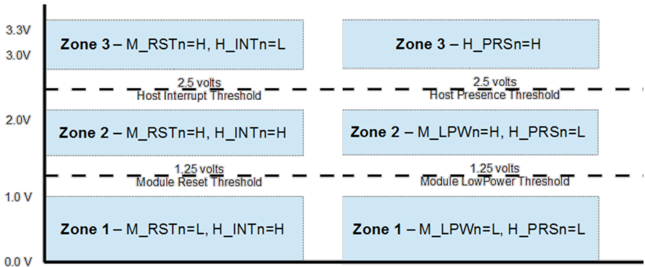
Figure 1. Voltage Zones
