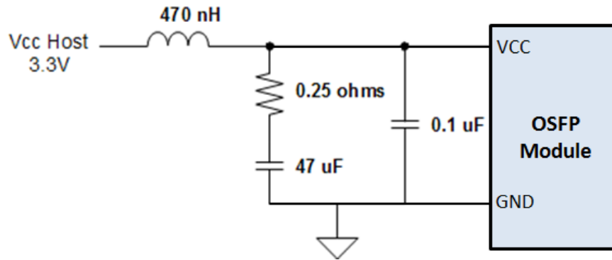
Figure 5. Recommended Power Supply Filter
