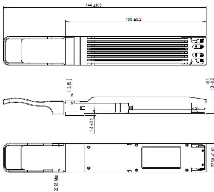
Figure 6. Mechanical Outline
